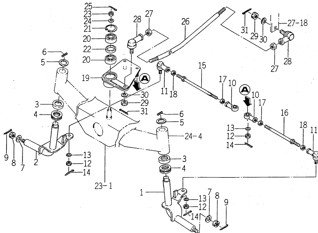
FIG. 25 KNUCKLE ARM SYSTEM
