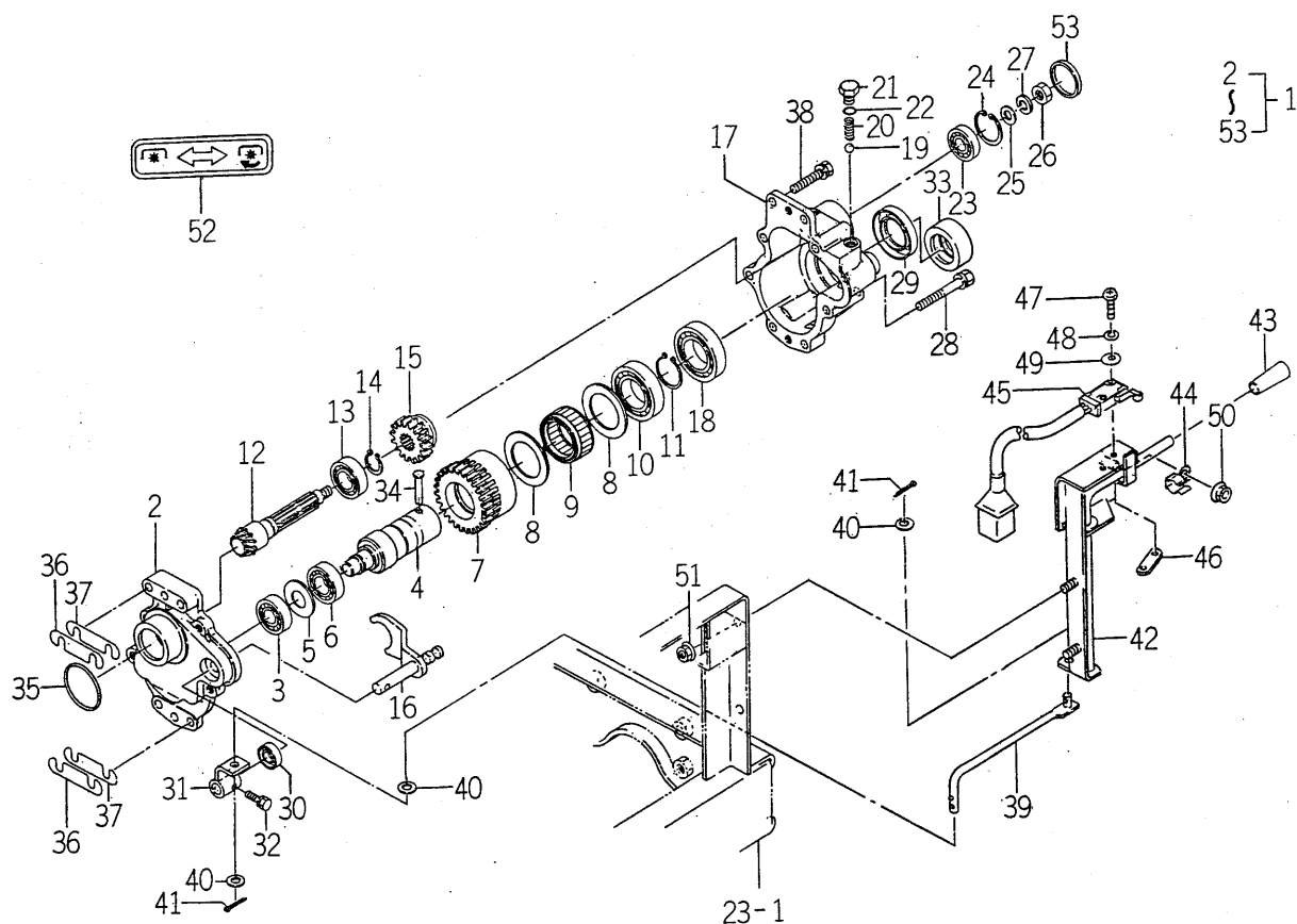
FIG. 21 REAR PTO SYSTEM (OPTION)
