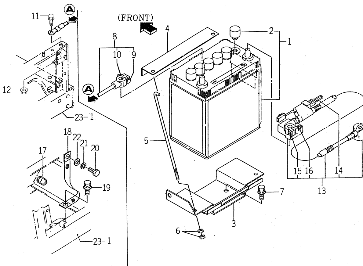
FIG. 5 BATTERY SYSTEM
