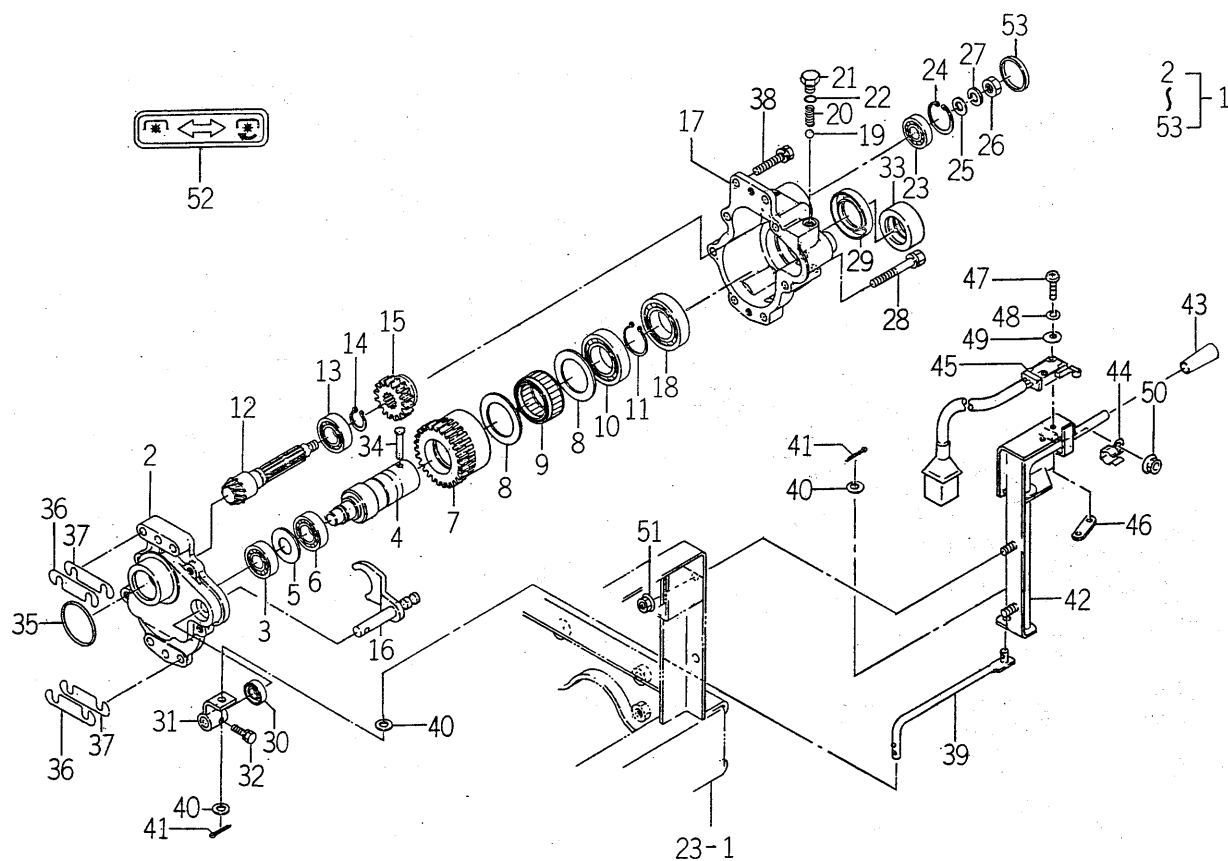
FIG. 21 REAR PTO SYSTEM (OPTION)
