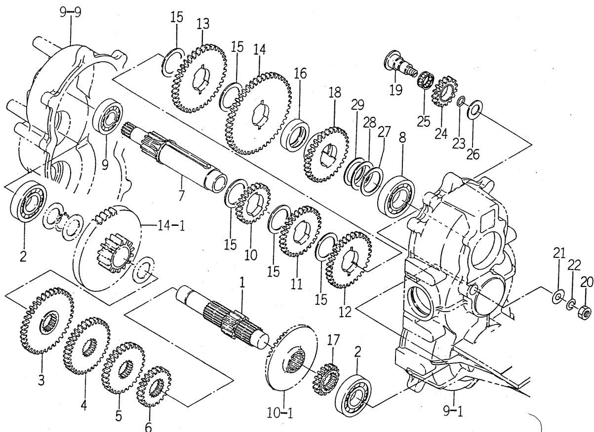
FIG. 11 CHANGE SHAFT SYSTEM
