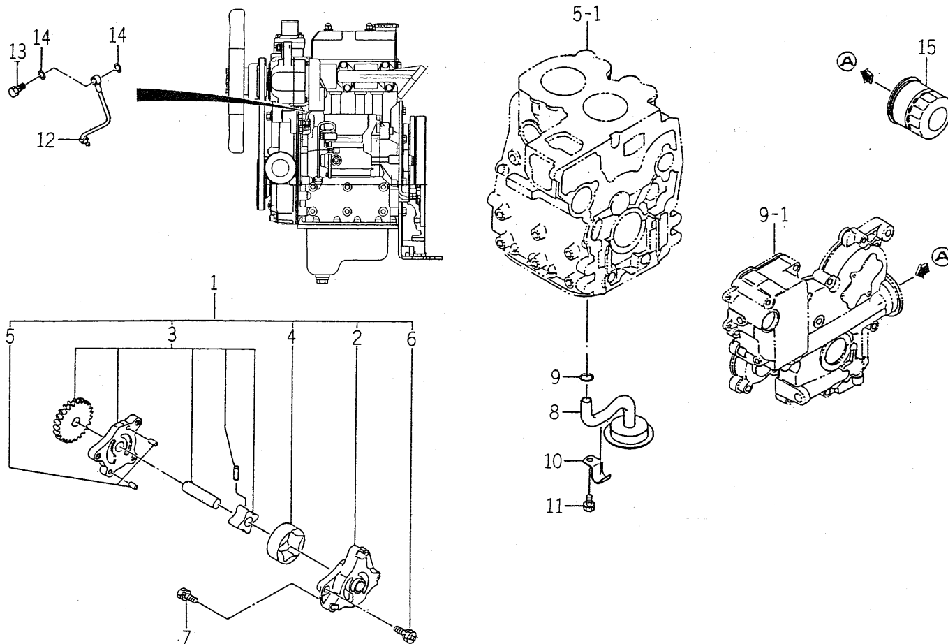
FIG. 16 OIL PUMP
