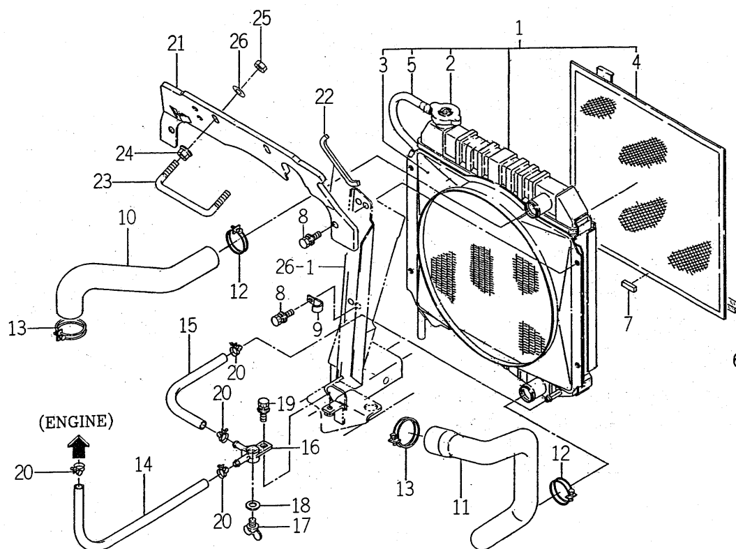
FIG. 2 RADIATOR SYSTEM
