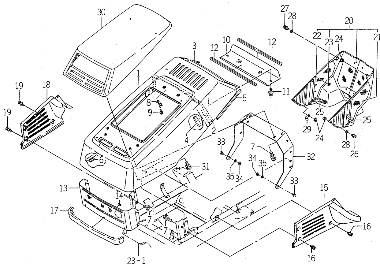
FIG. 34 HOOD SYSTEM
