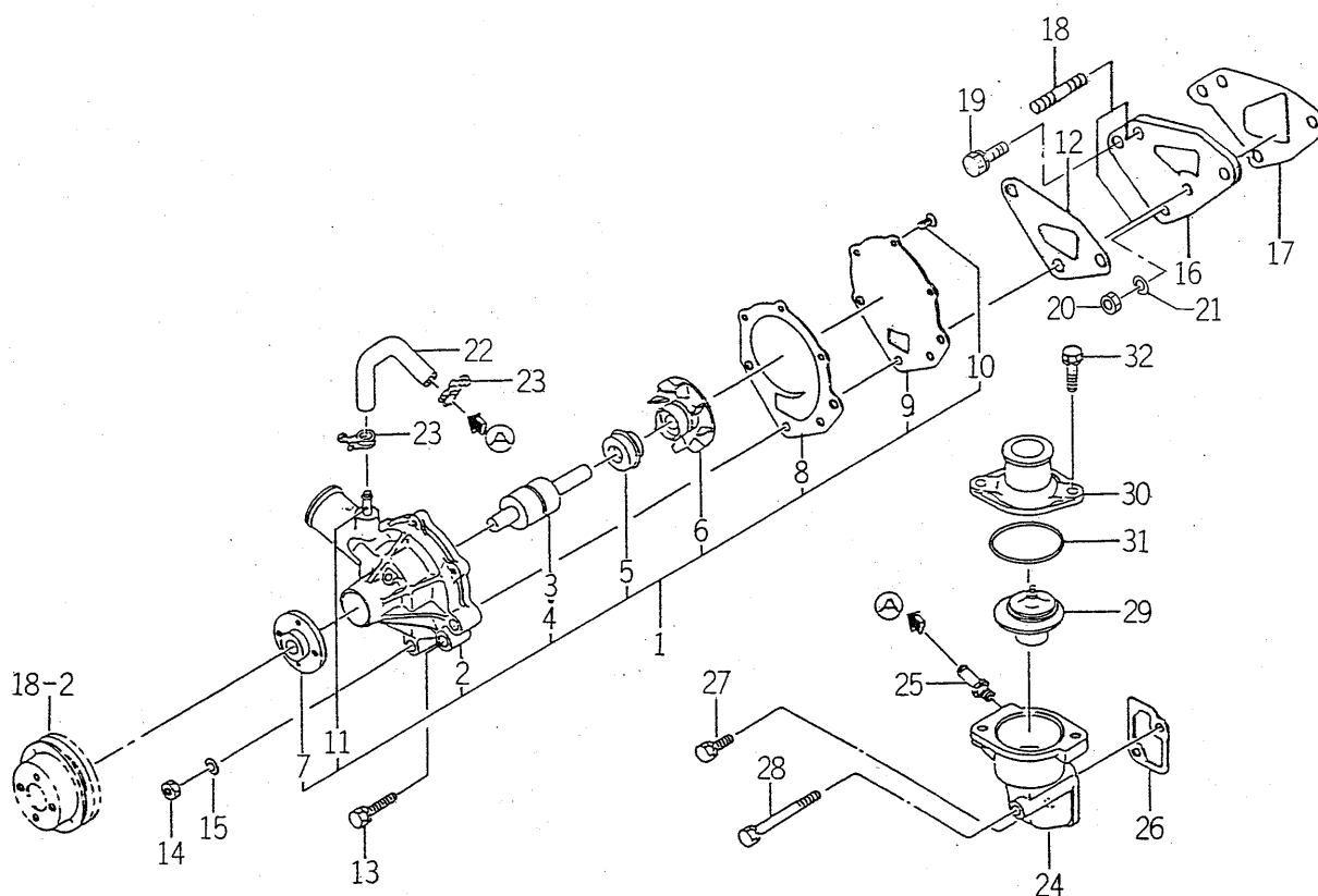
FIG. 17 WATER PUMP
