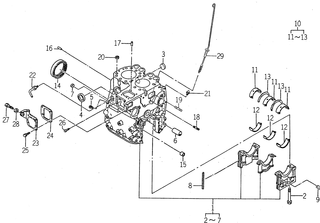
FIG. 5 CYLINDER BLOCK
