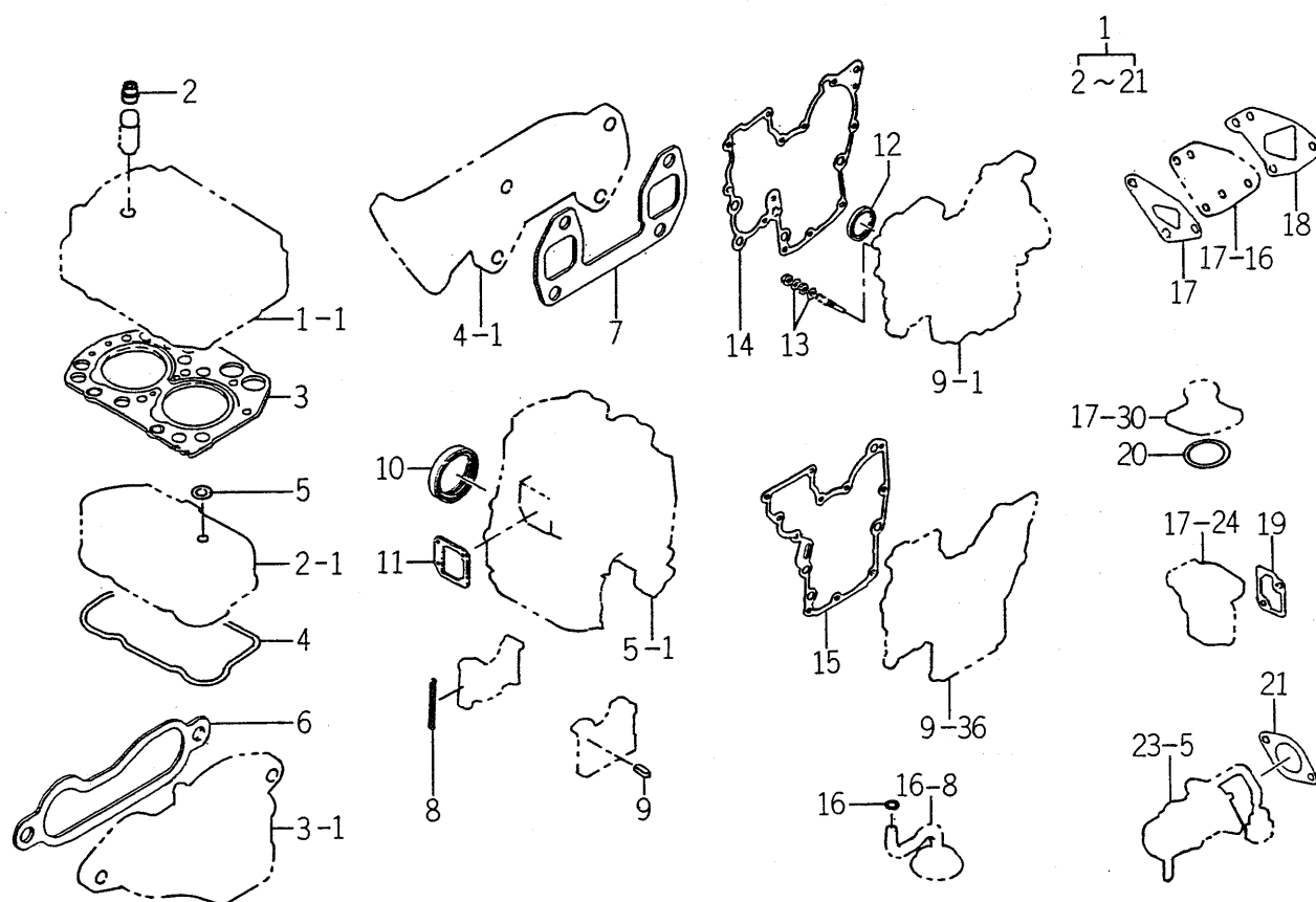
FIG. 24 REPAIR KIT
