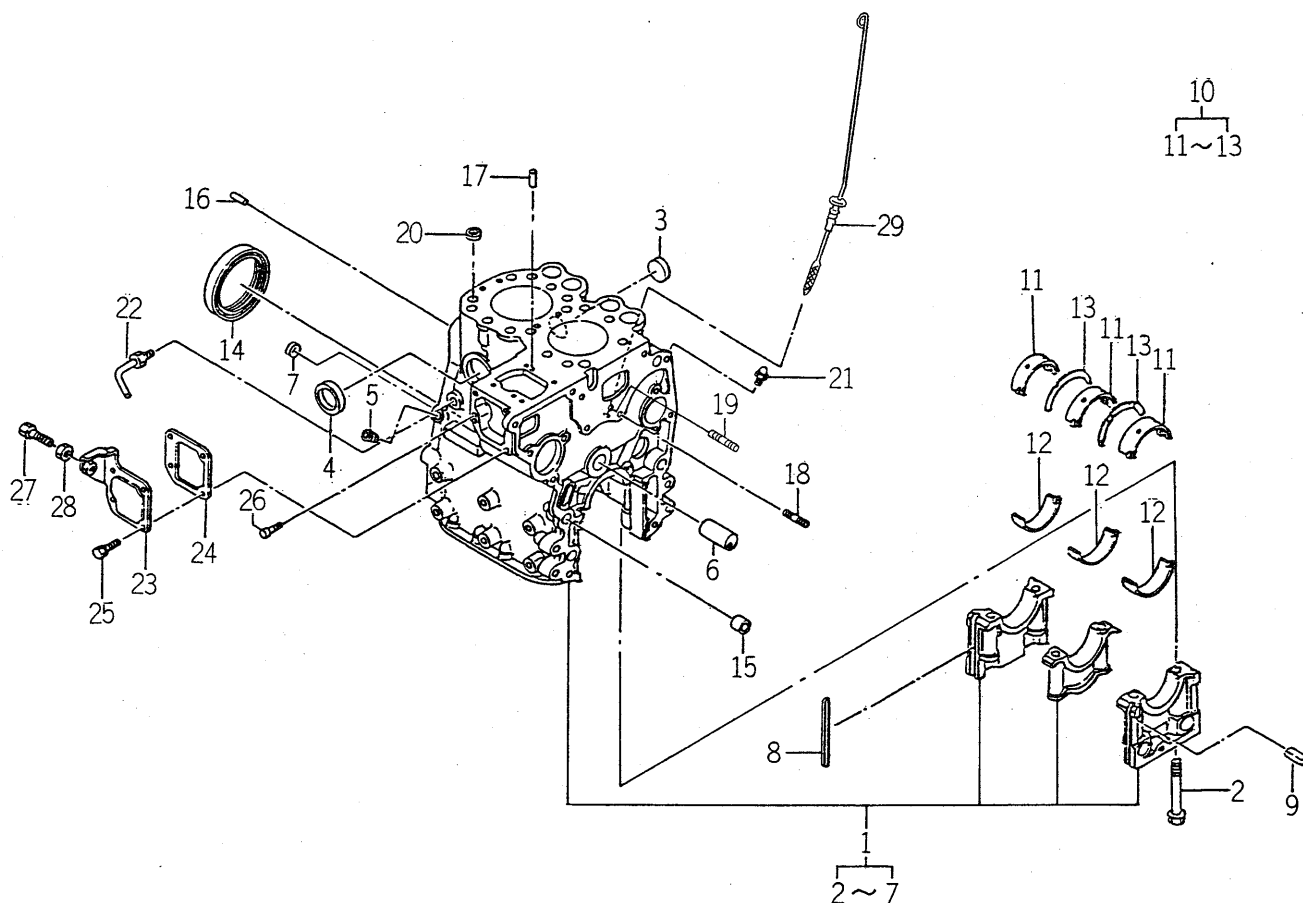
FIG. 5 CYLINDER BLOCK
