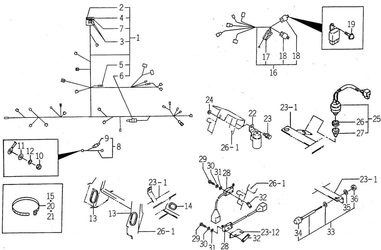
FIG. 41 HARNESS SYSTEM (S TYPE)
