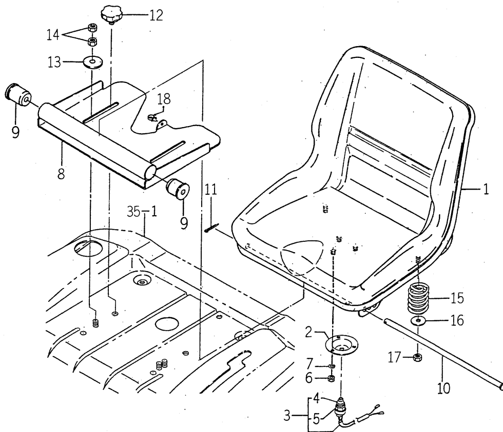
FIG. 36 SEAT SYSTEM
