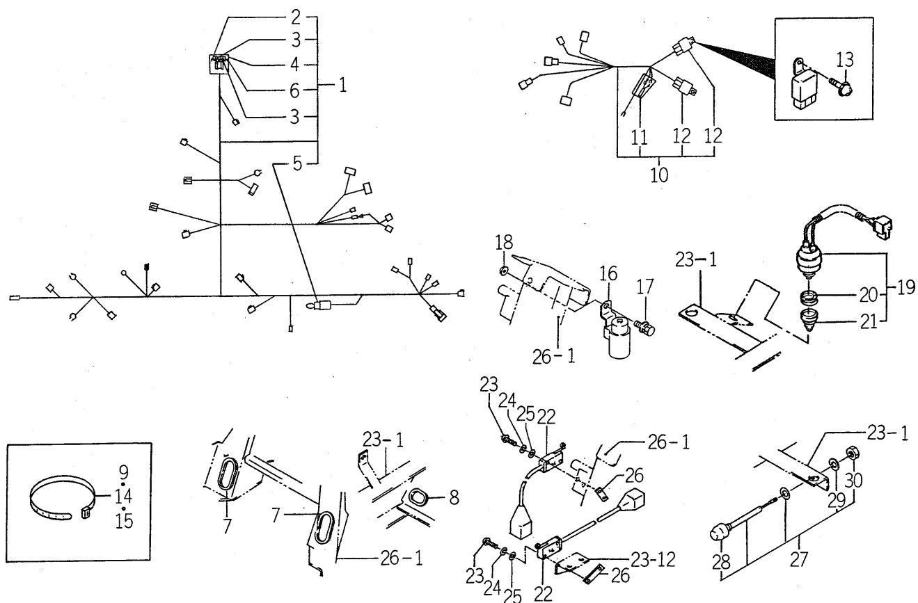
FIG. 40 HARNESS SYSTEM (EXCEPT S TYPE)
