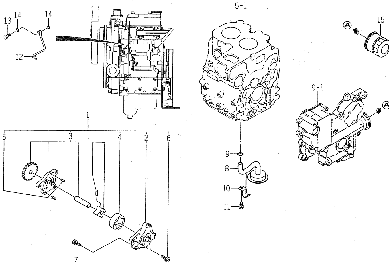
FIG. 16 OIL PUMP
