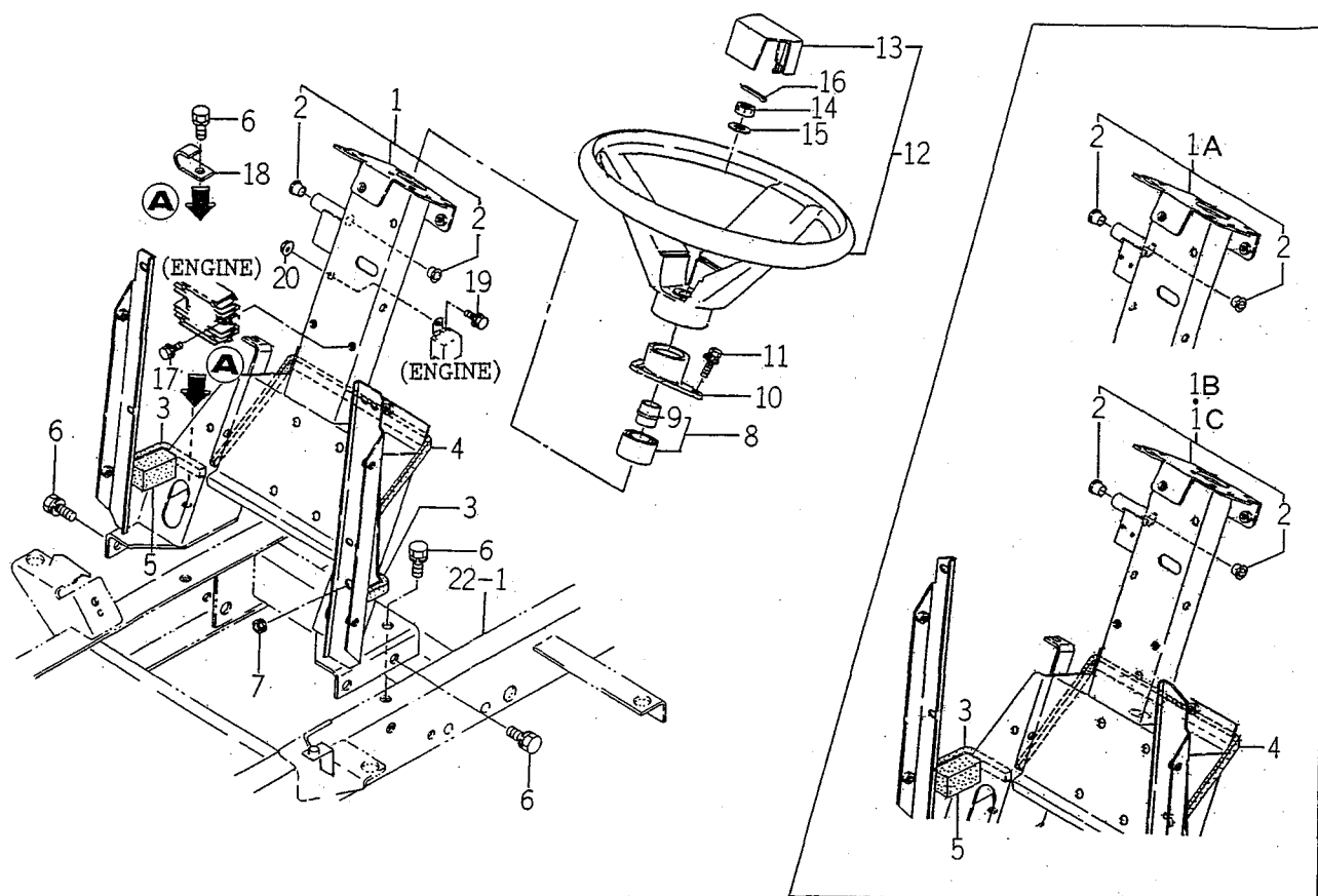
FIG. 25 POST (STEERING) and WHEEL (STEERING) SYSTEM
