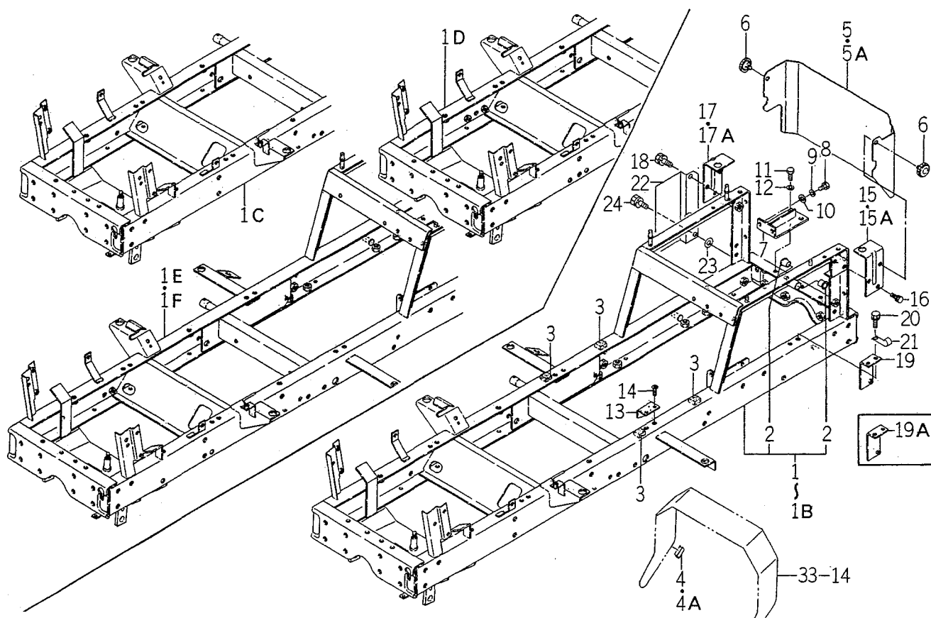
FIG. 22 CHASSIS SYSTEM
