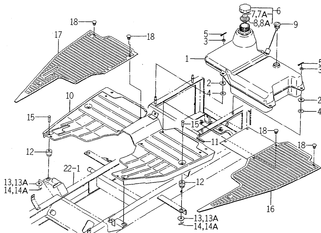
FIG. 37 TANK (FUEL) and STEP SYSTEM
