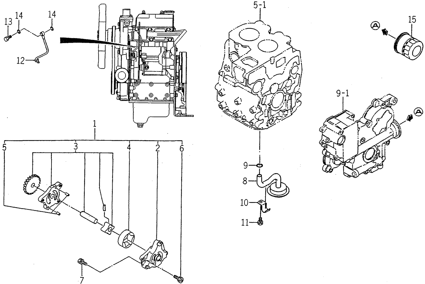
FIG. 16 OIL PUMP
