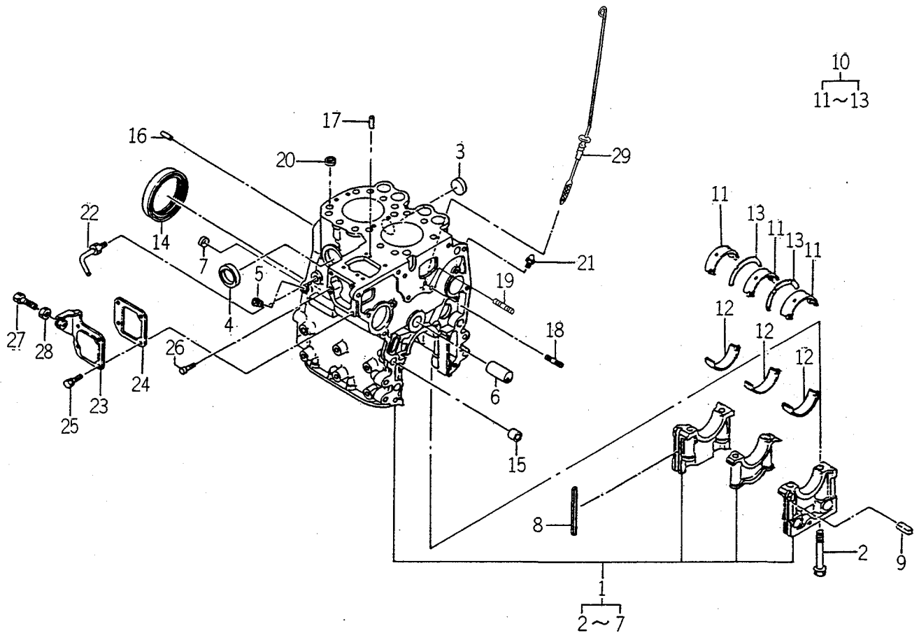
FIG. 5 CYLINDER BLOCK
