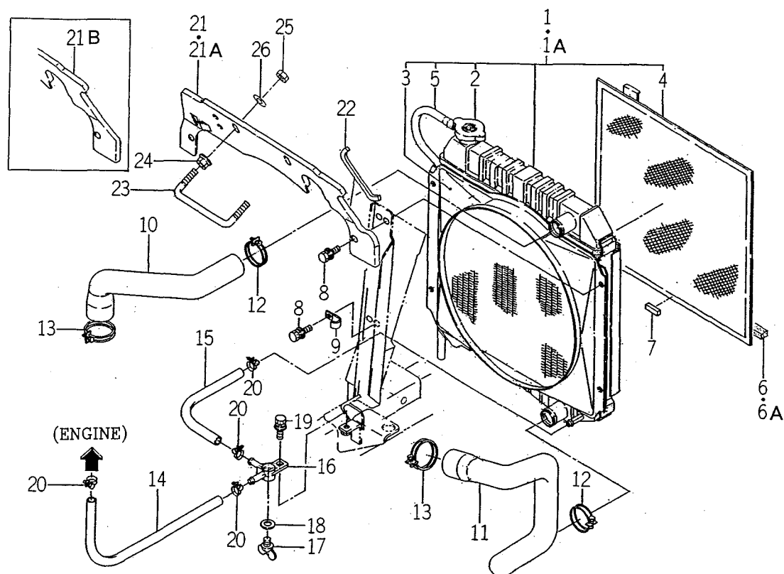
FIG. 2 RADIATOR SYSTEM
