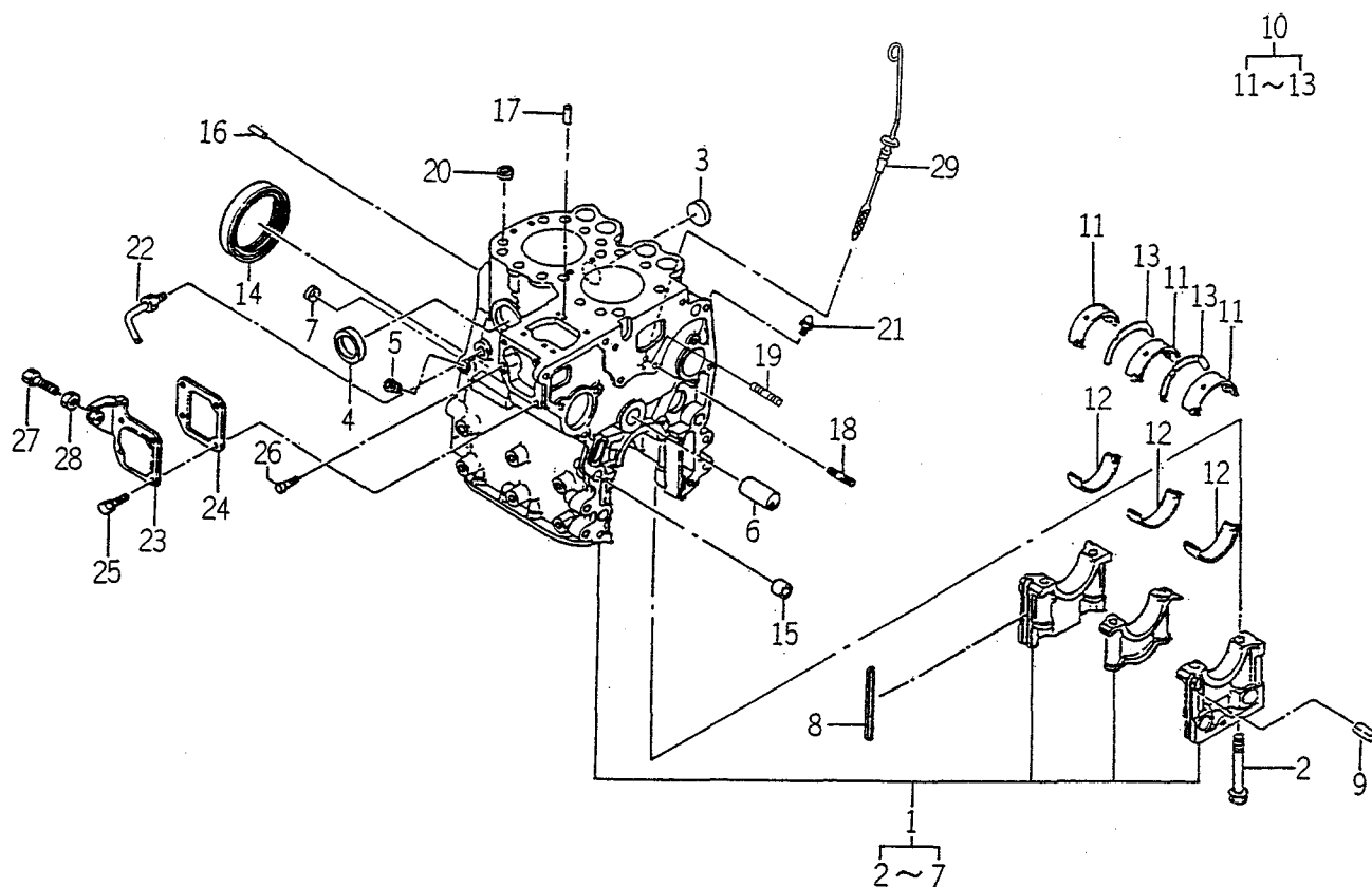
FIG. 5 CYLINDER BLOCK
