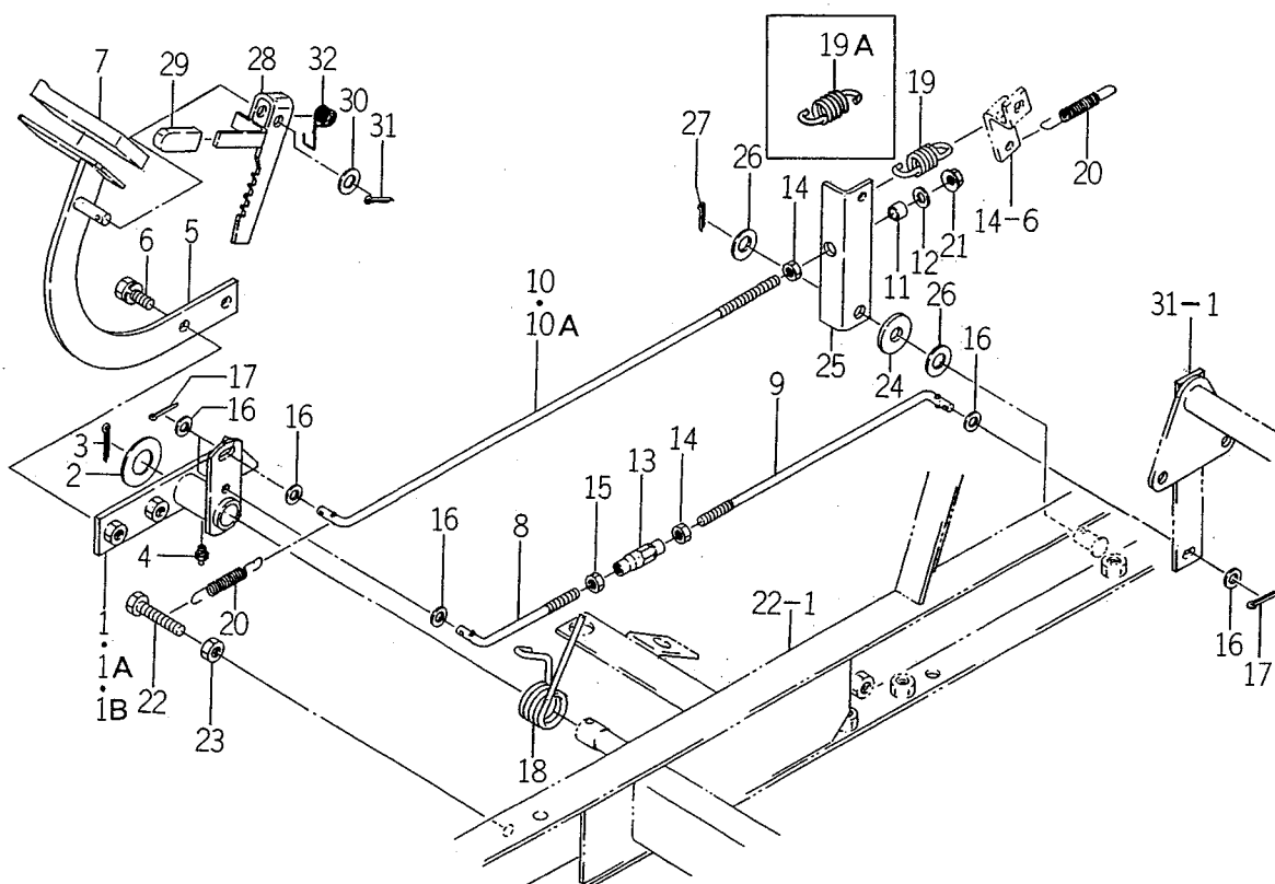
FIG. 15 ARM (CLUTCH/BRAKE) and ARM (PEDAL) SYSTEM
