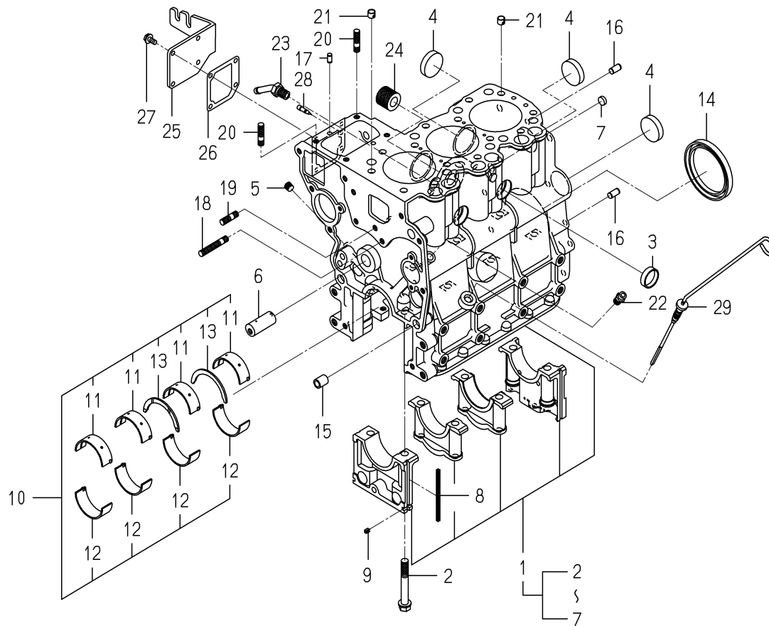
FIG.201 CYLINDER BLOCK
