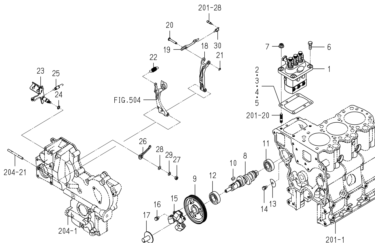
FIG.502 INJECTION PUMP
