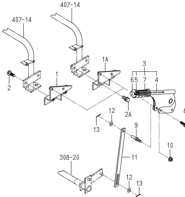
FIG.310 BRAKE(PARKING)SYSTEM(G TYPE)
