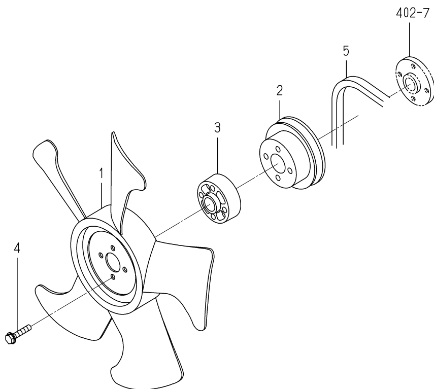
FIG.403 COOLING FAN
