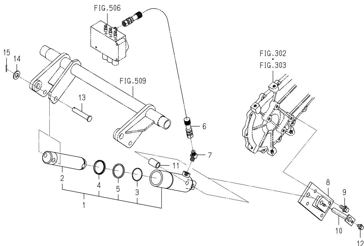
FIG.502 CYLINDER(LIFT)SYSTEM
