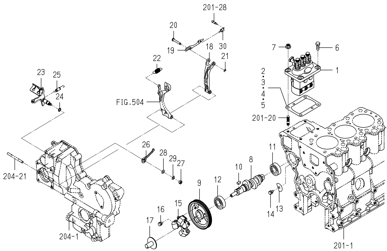
FIG.502 INJECTION PUMP
