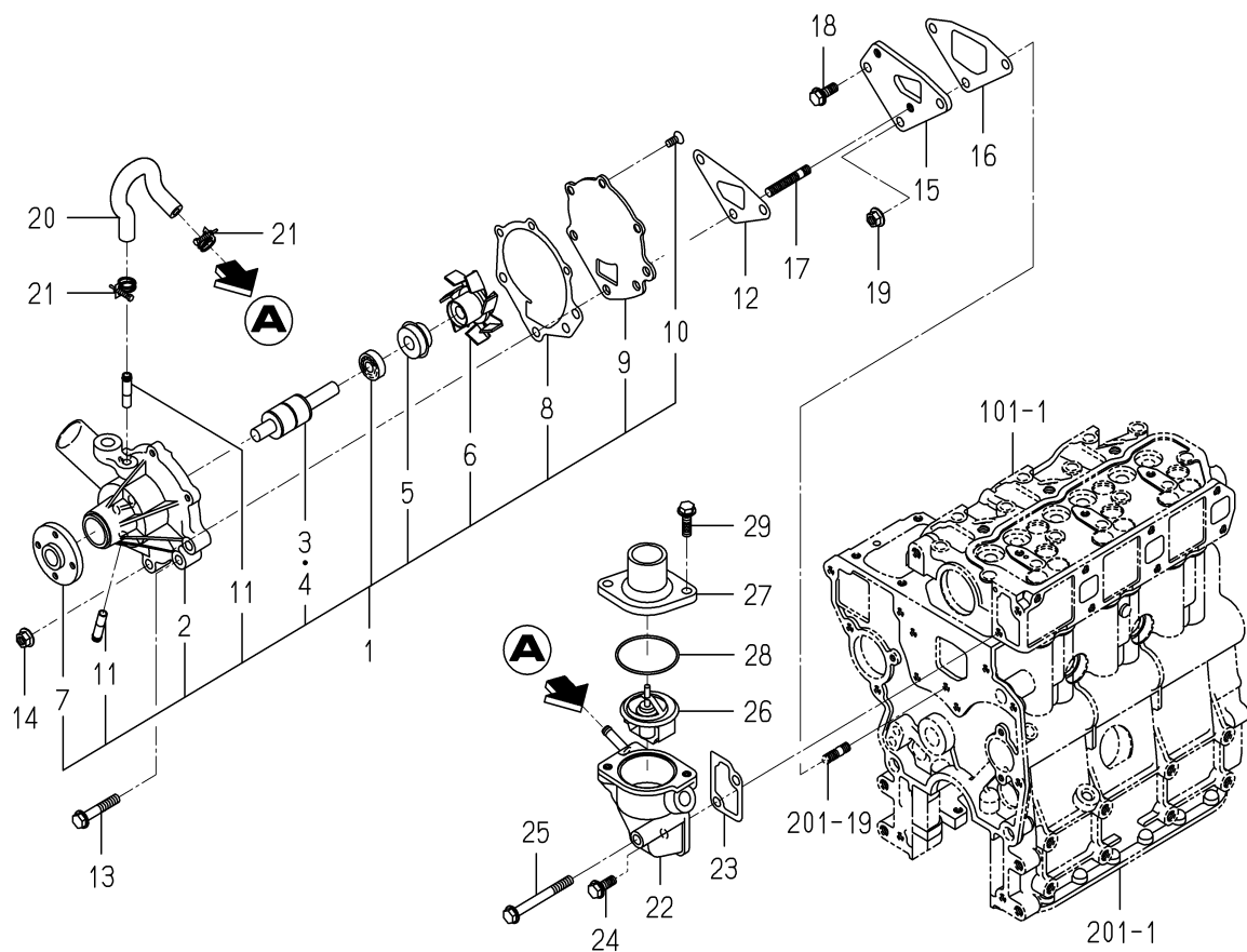
FIG.402 WATER PUMP
