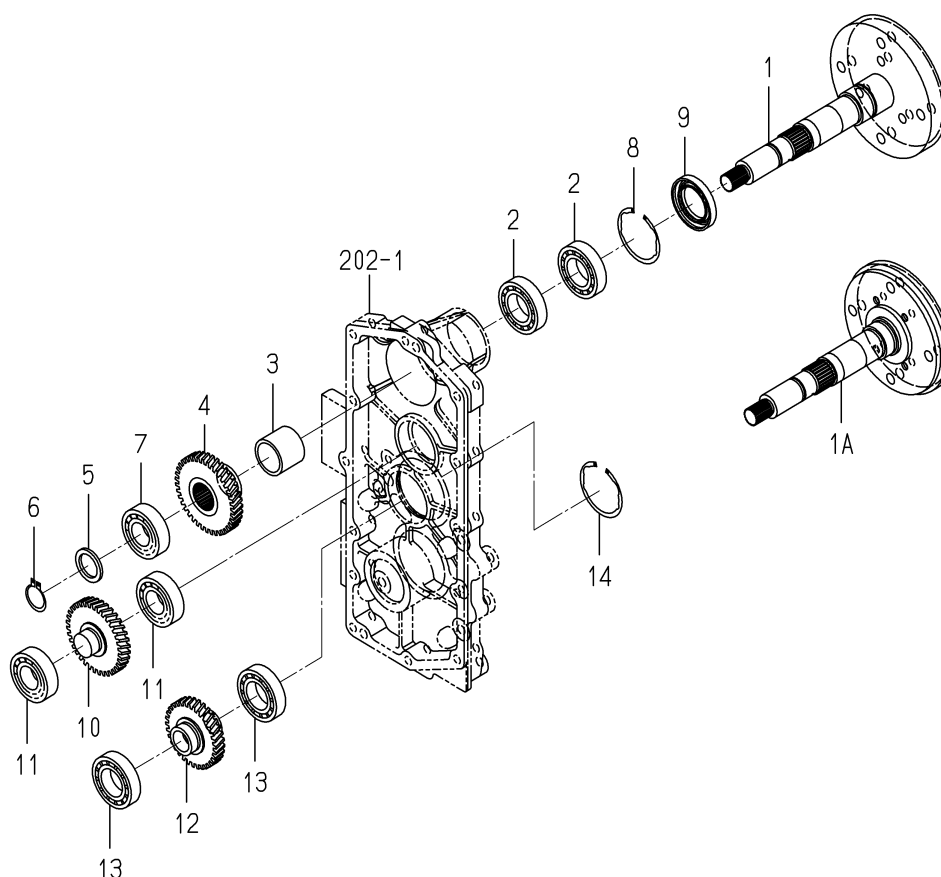
FIG.203 GEAR(INPUT)SYSTEM
