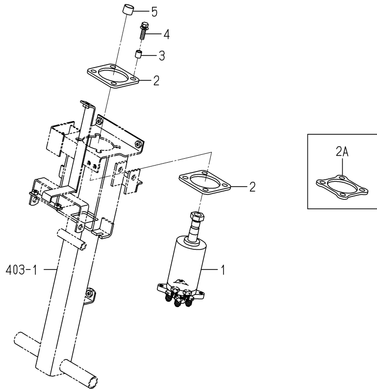
FIG.404 CONTROLLER(STEERING)SYSTEM
