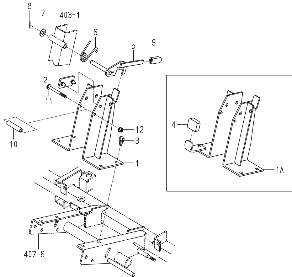
FIG.402 LEVER(TILT)SYSTEM
