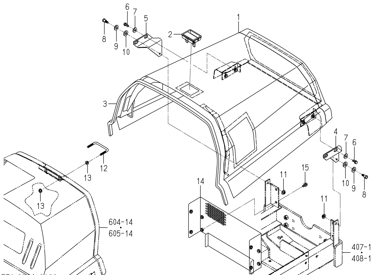
FIG.601 HOOD SYSTEM
