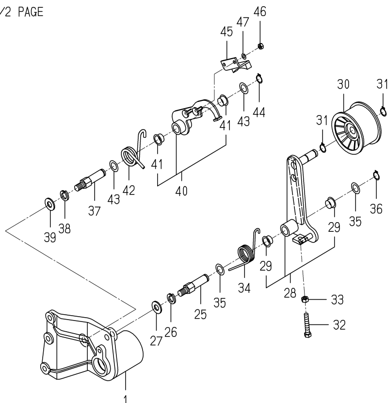
FIG.213 DRIVE(PTO/SIDE)SYSTEM(B TYPE)(2/2)
