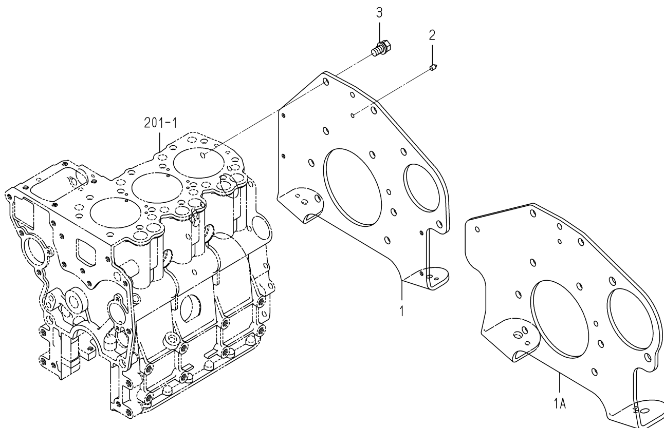
FIG.203 REAR PLATE
