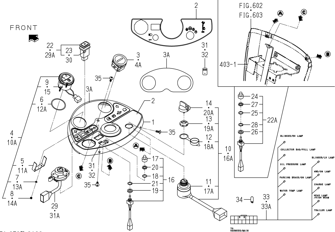
FIG.609 PANEL SYSTEM(G TYPE)
