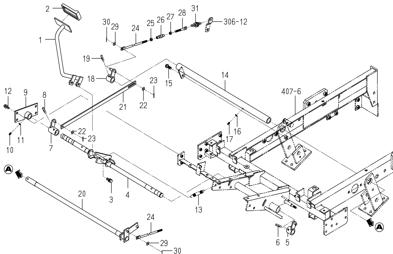
FIG.308 PEDAL(BRAKE)SYSTEM(G TYPE)
