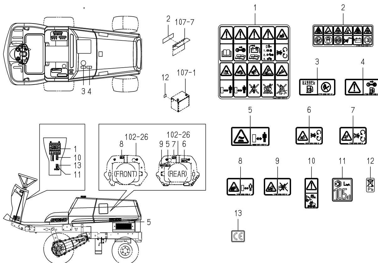
FIG.911 LABEL(CAUTION) (EXCEPT SFH240F-B TYPE)
