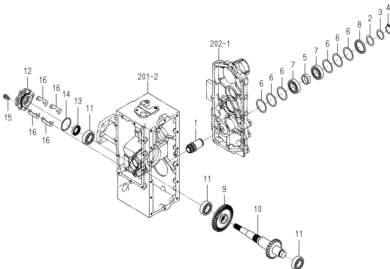
FIG.206 GEAR(DRIVE)SYSTEM(EXCEPT G TYPE)
