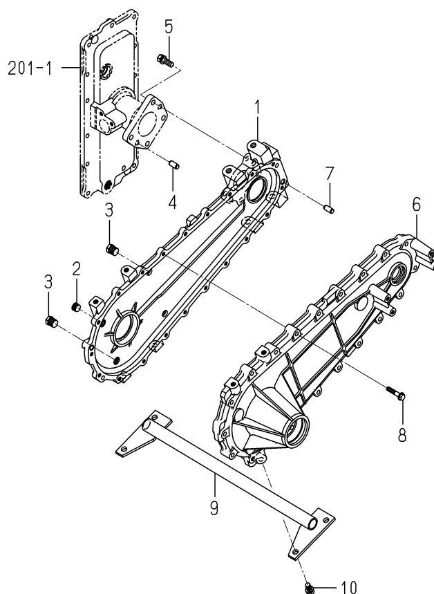
FIG.301 HOUSING(AXLE/FRONT)SYSTEM
