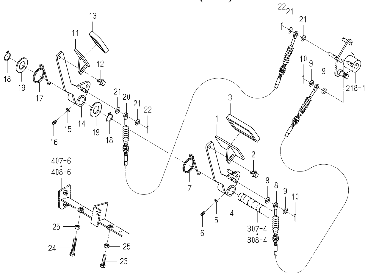
FIG.219 PEDAL(HST)SYSTEM
