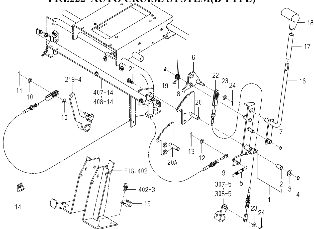
FIG.222 AUTO CRUISE SYSTEM(B TYPE)
