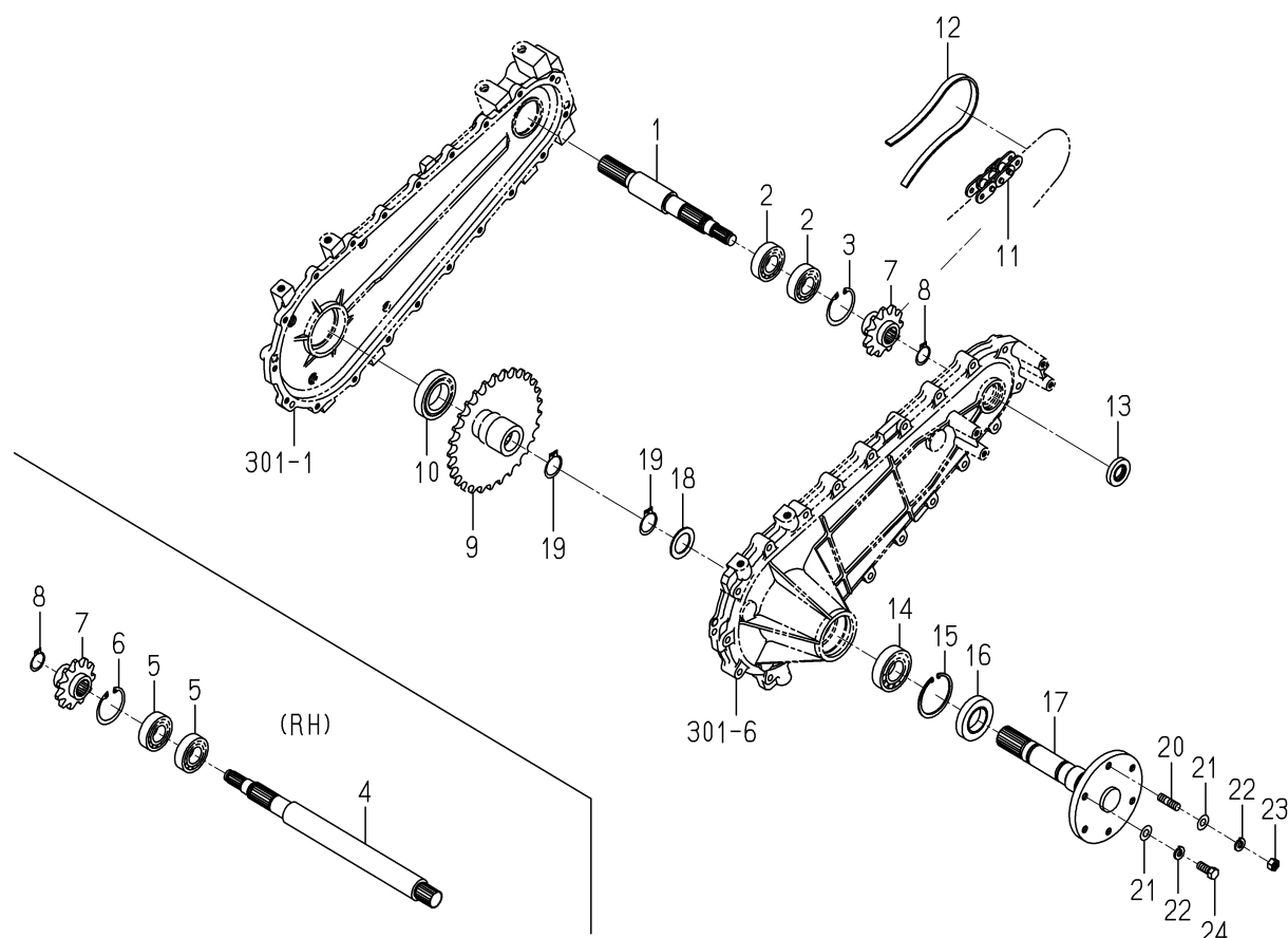
FIG.303 SHAFT(WHEEL/FRONT)SYSTEM(G TYPE)
