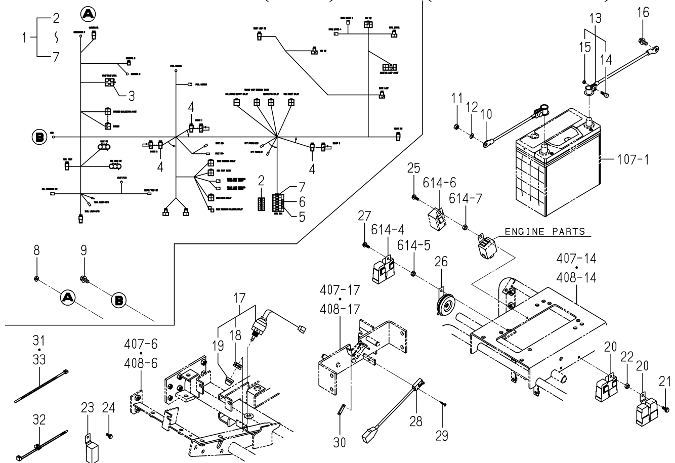
FIG.610 HARNESS(MAIN)SYSTEM(EXCEPT G TYPE)
