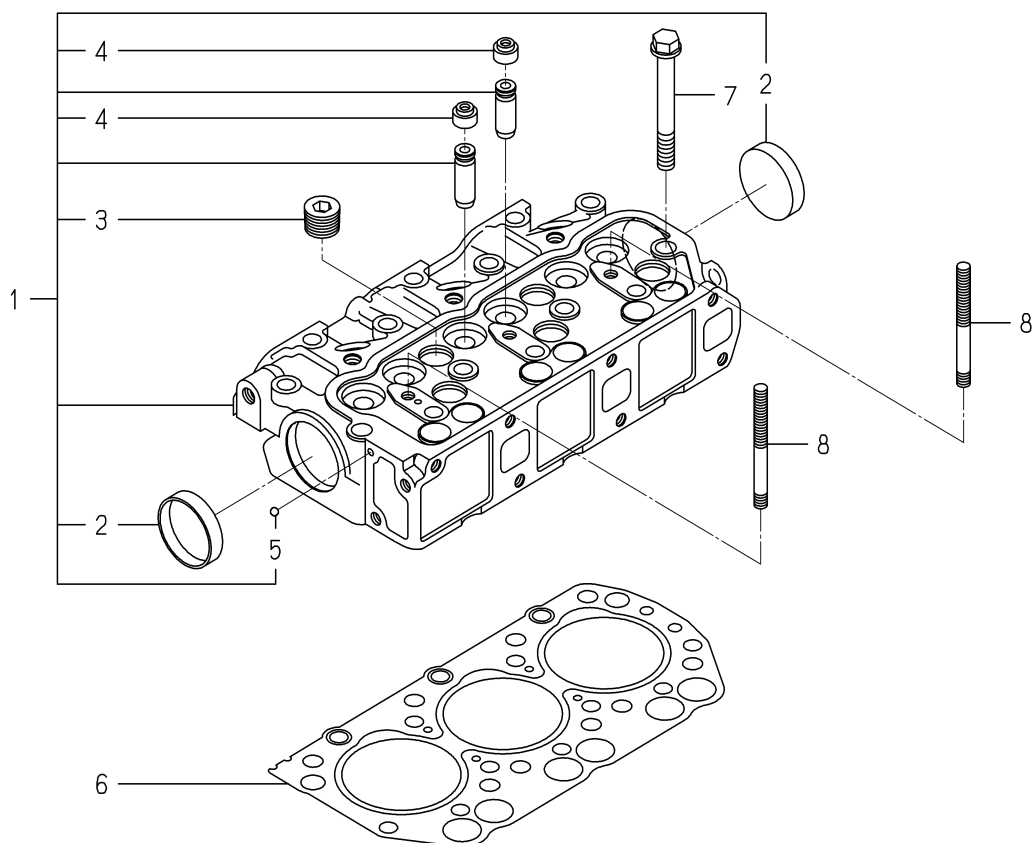
FIG.101 CYLINDER HEAD
