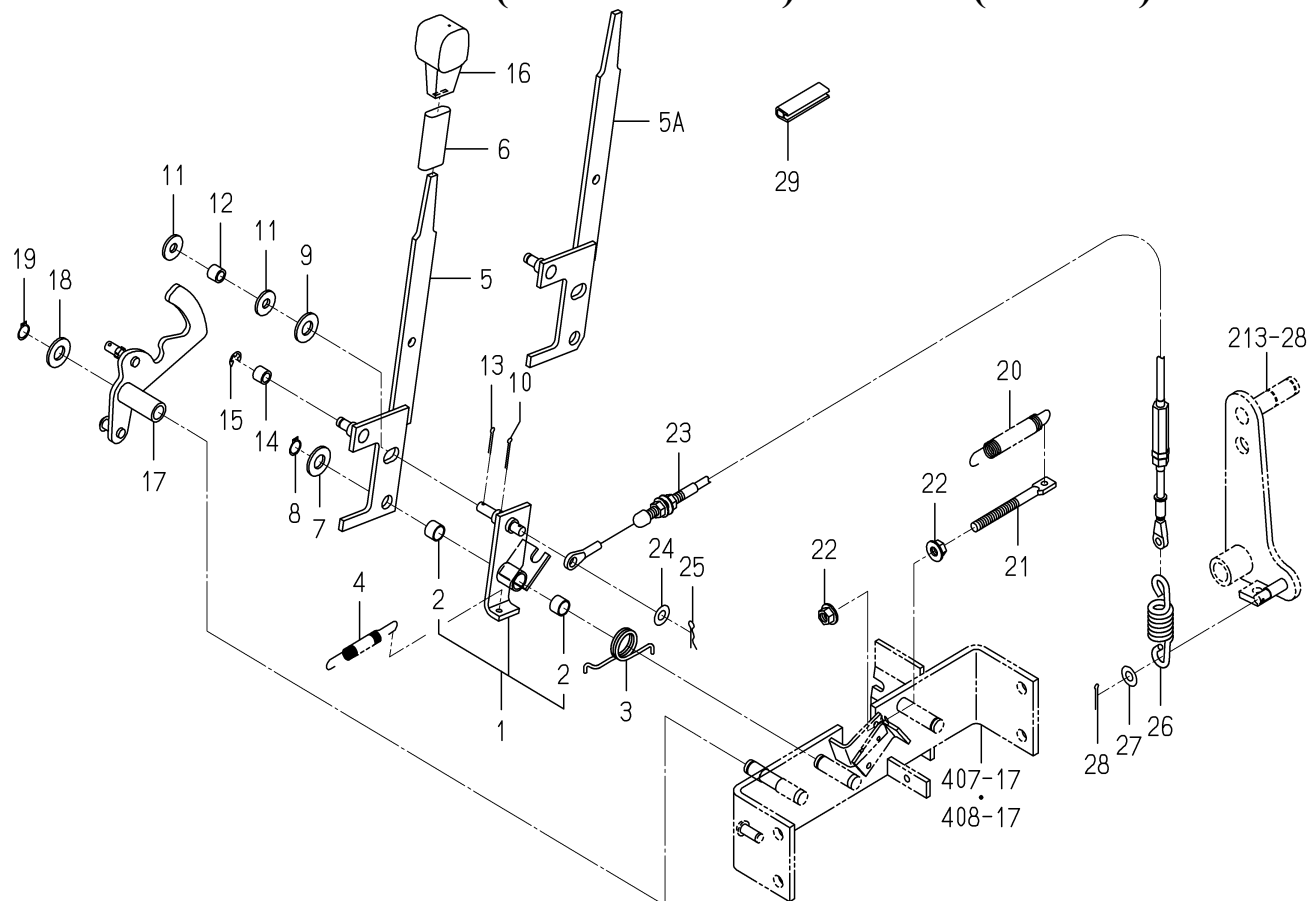
FIG.220 LEVER(PTO/MOWER)SYSTEM(B TYPE)
