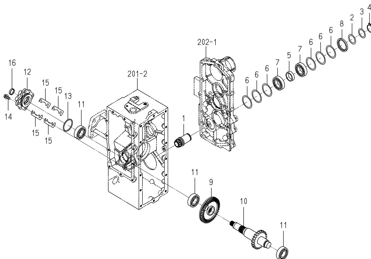
FIG.207 GEAR(DRIVE)SYSTEM(G TYPE)
