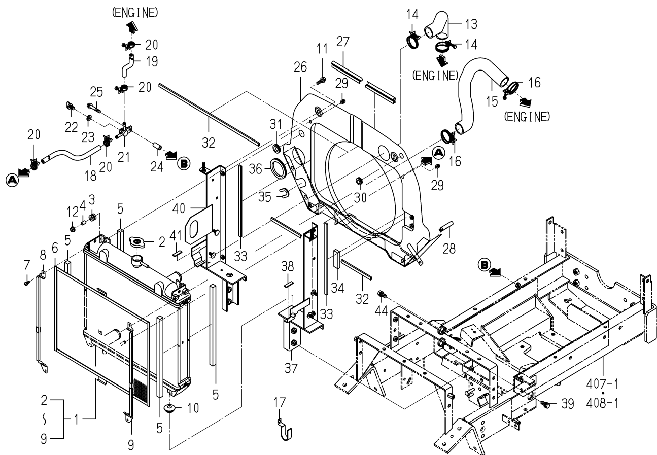
FIG.102 RADIATOR SYSTEM(1/2)
