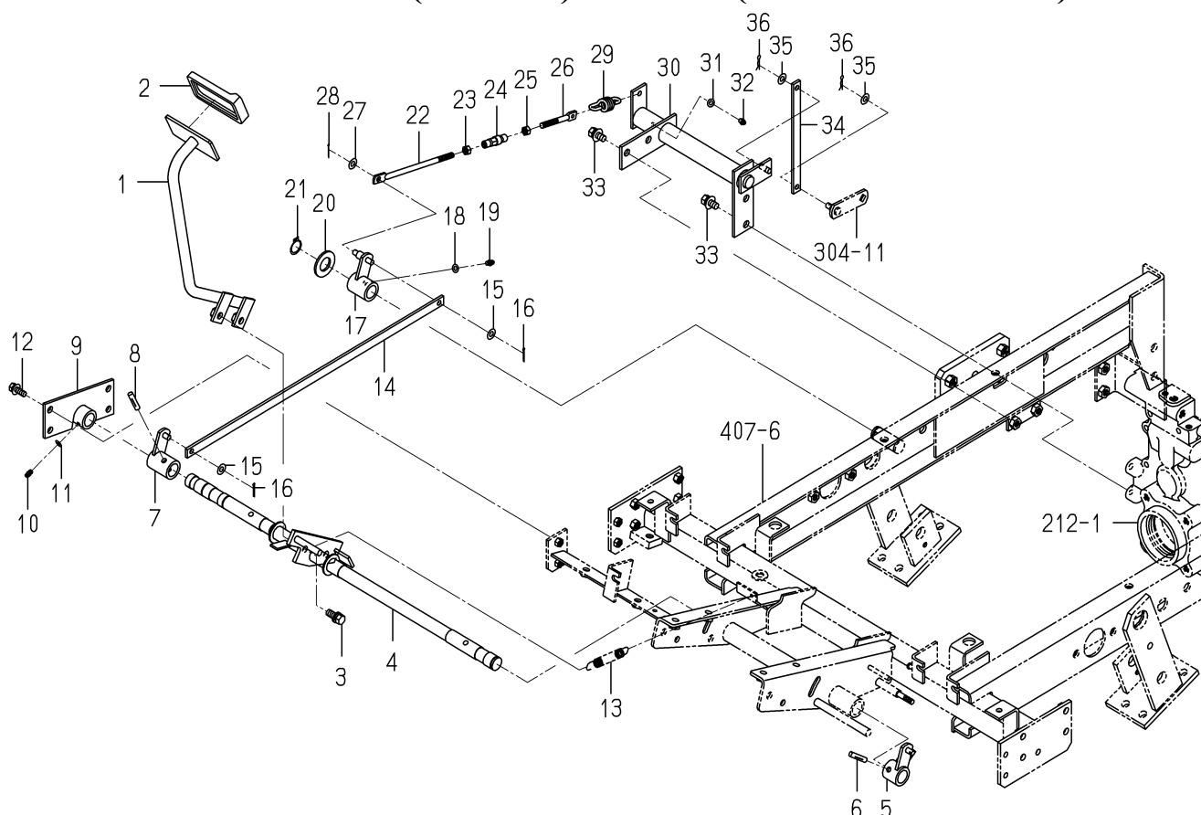
FIG.307 PEDAL(BRAKE)SYSTEM(EXCEPT G TYPE)
