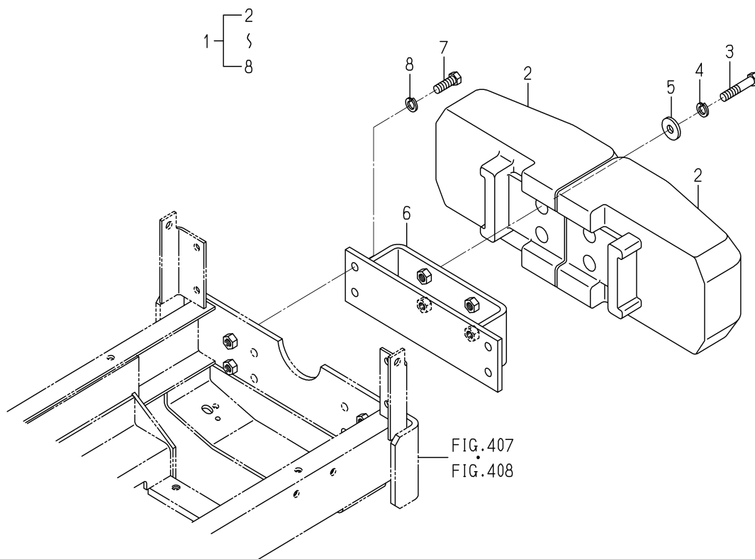
FIG.912 WEIGHT(REAR)SYSTEM(W TYPE) (EXCEPT W TYPE:OPTION)
