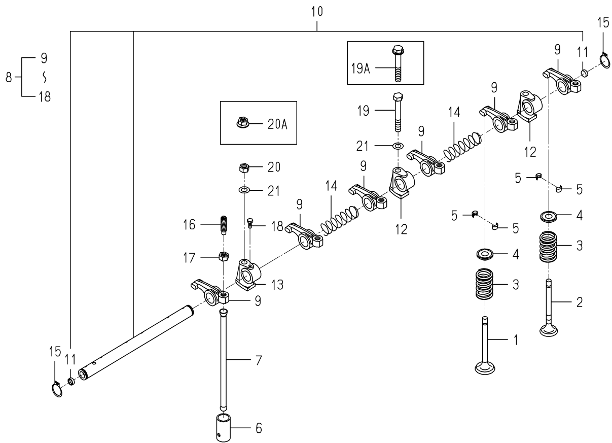
FIG.301 VALVE
