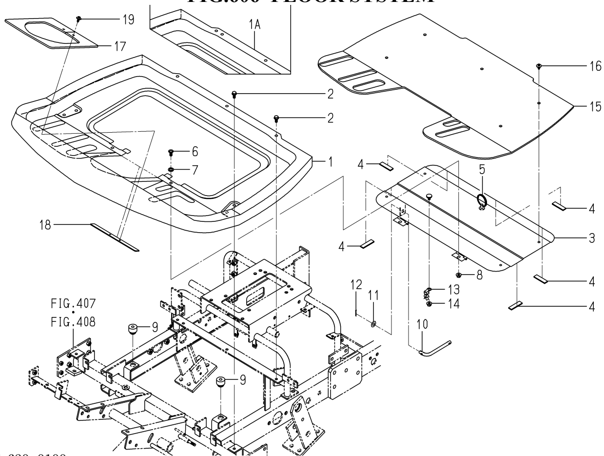
FIG.606 FLOOR SYSTEM
