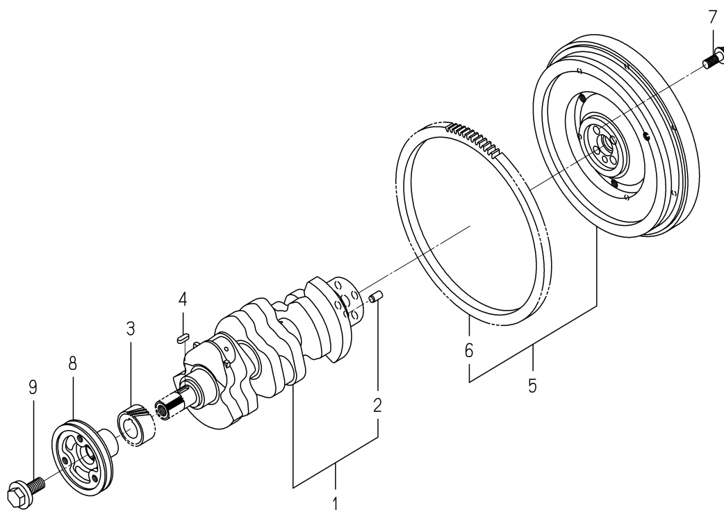
FIG.304 CRANK SHAFT
