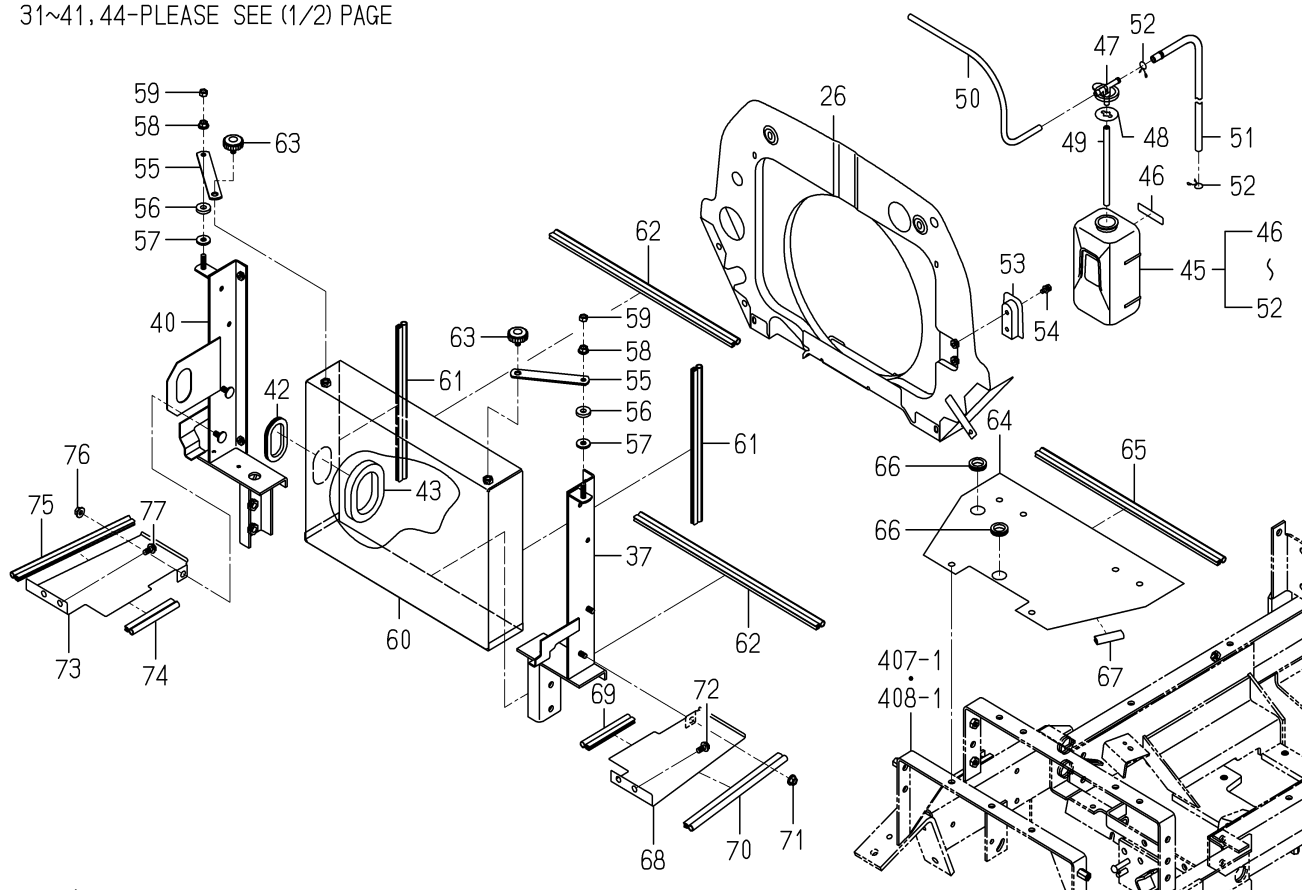
FIG.102 RADIATOR SYSTEM(2/2)
