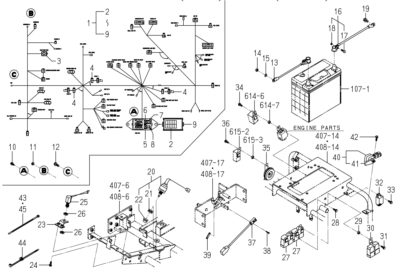
FIG.611 HARNESS(MAIN)SYSTEM(G TYPE)
