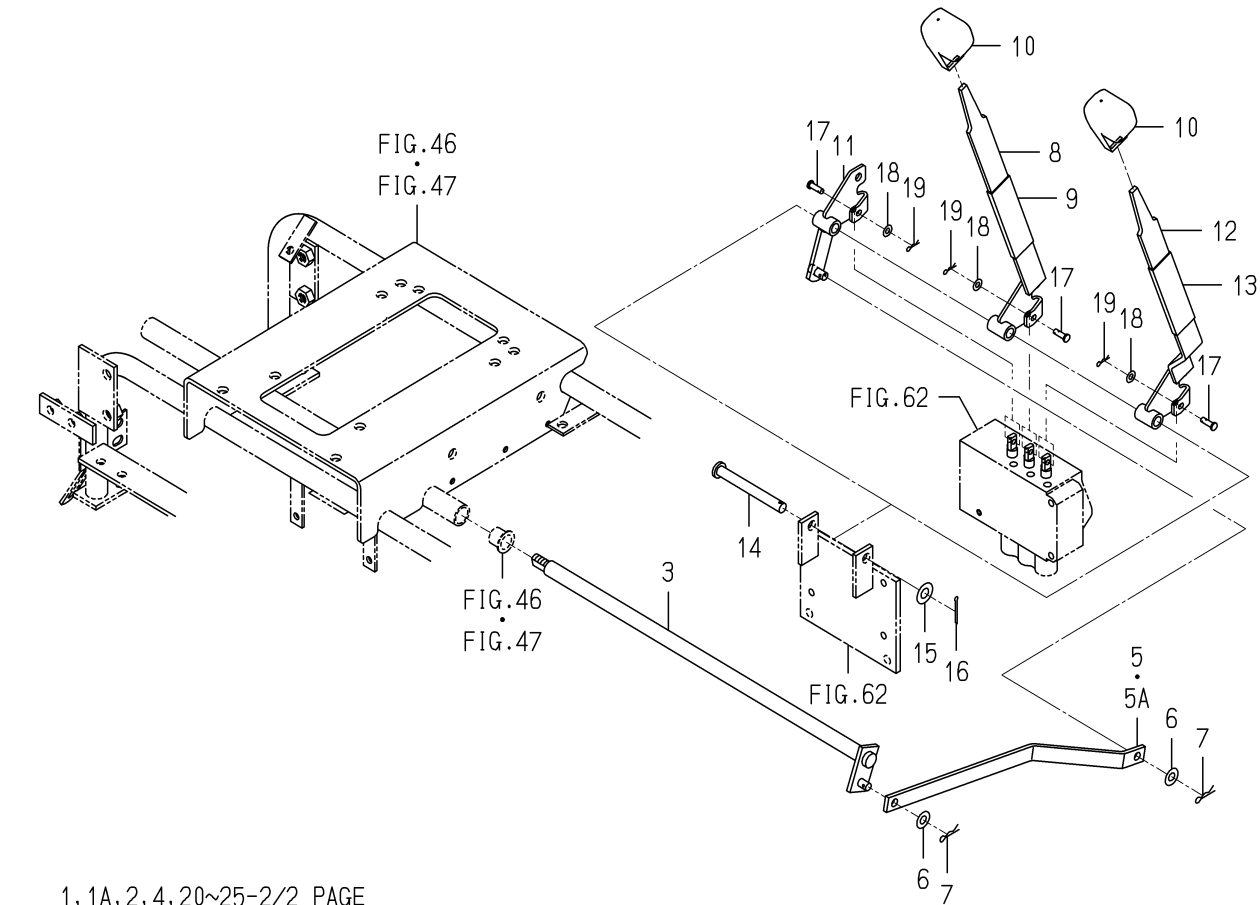
FIG. 57 CONTROL SYSTEM(1/2)
