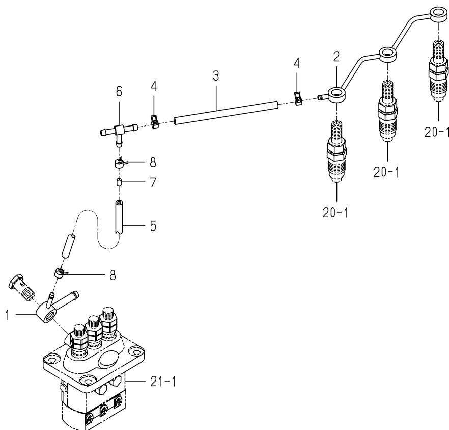
FIG. 22 FUEL PIPE
