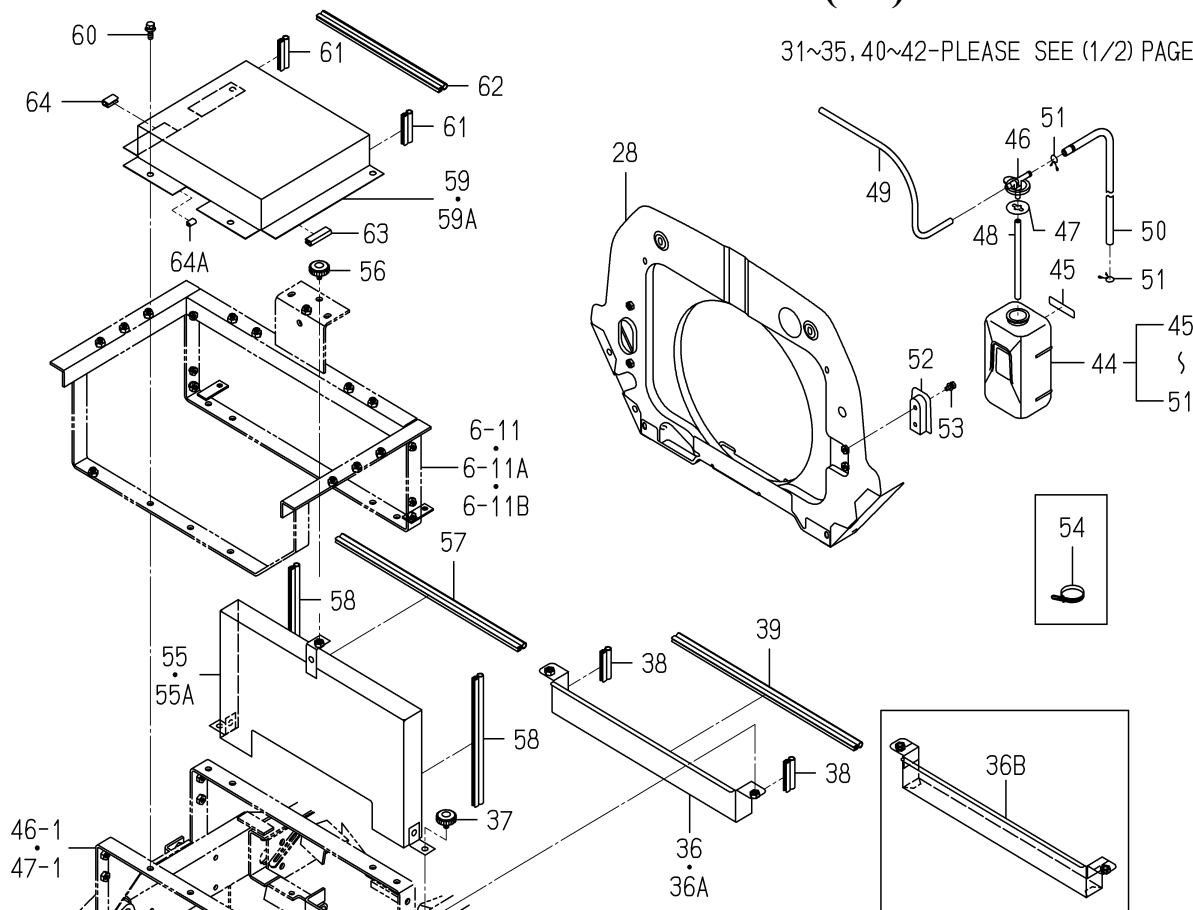
FIG. 2 RADIATOR SYSTEM(2/2)
