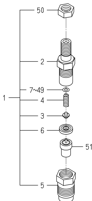
FIG. 28 COMPONENT PARTS FOR 6215-300-036-10 ON Fig.20
