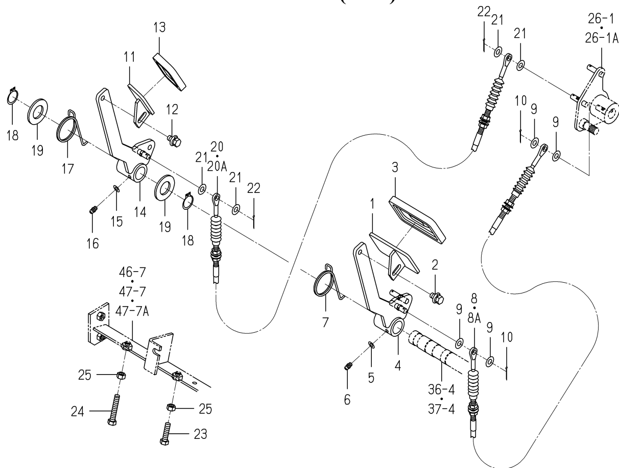
FIG. 27 PEDAL(HST)SYSTEM
