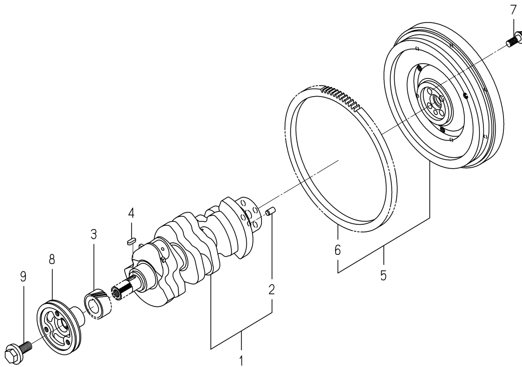
FIG. 16 CRANK SHAFT
