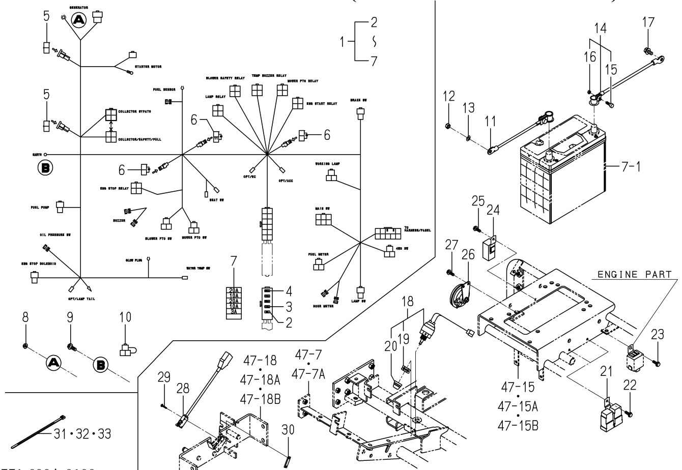
FIG. 77 HARNESS SYSTEM(SFH220:EXCEPT G TYPE)
