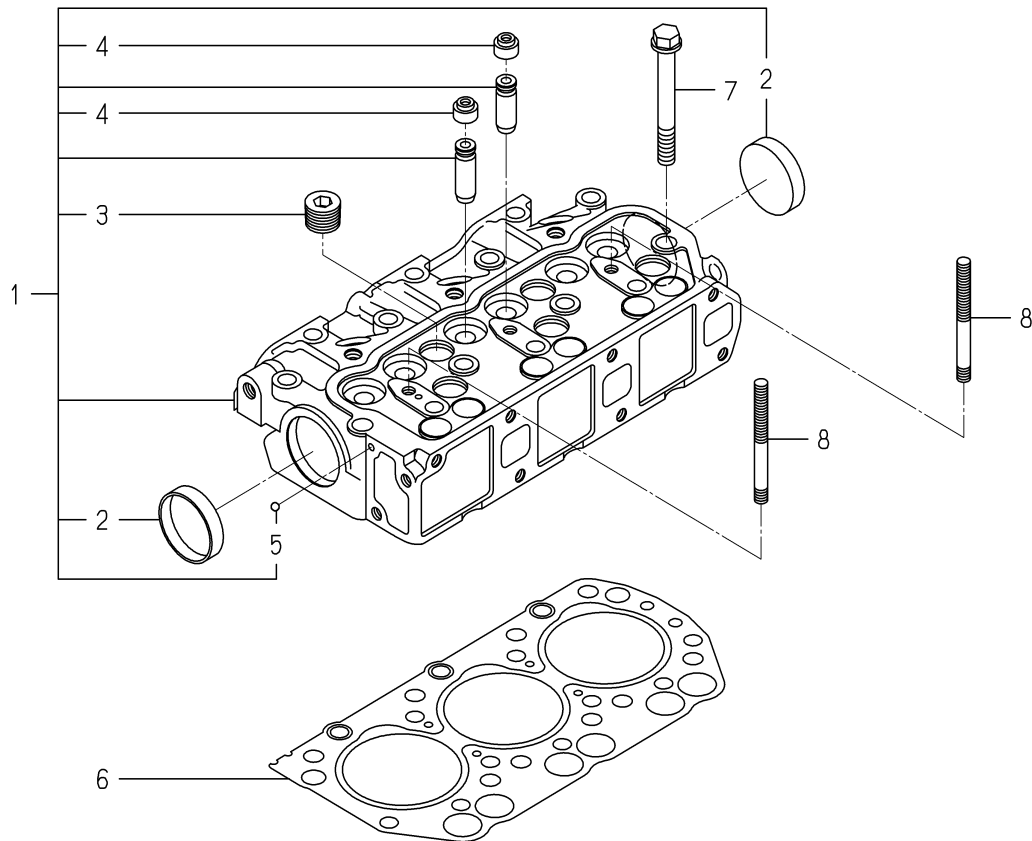
FIG. 2 CYLINDER HEAD
