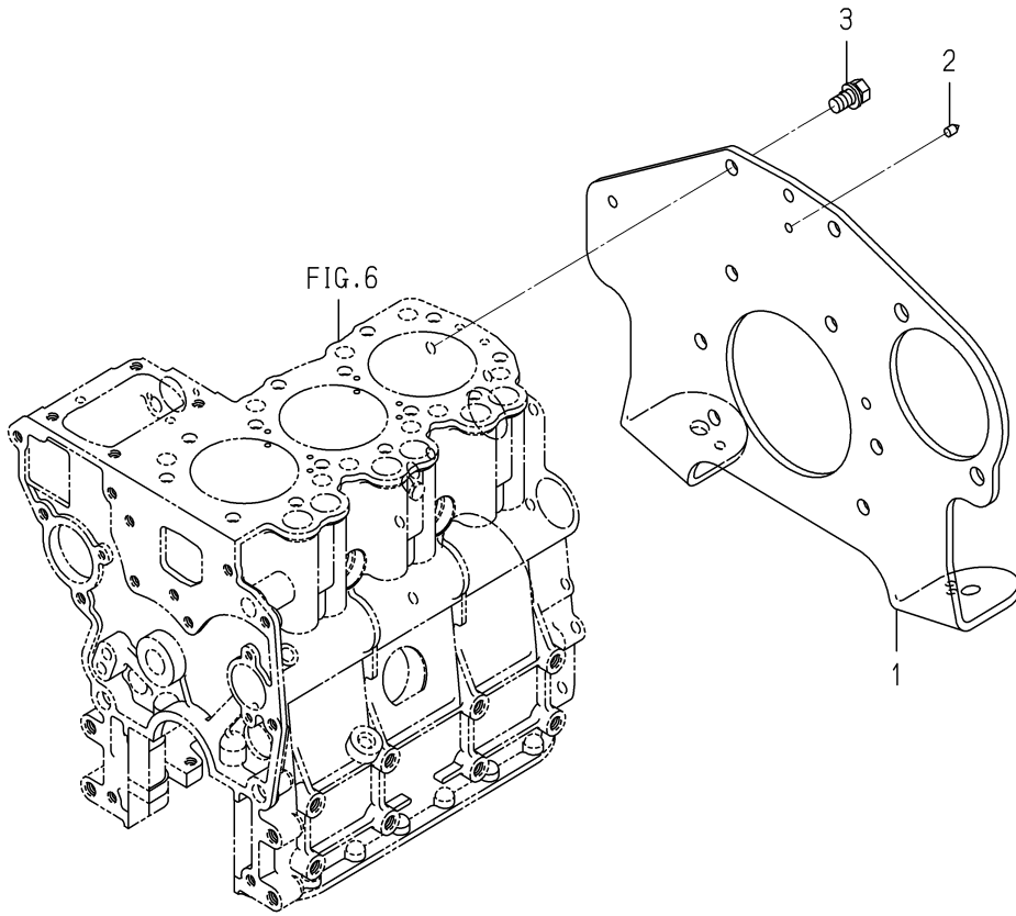
FIG. 9 REAR PLATE
