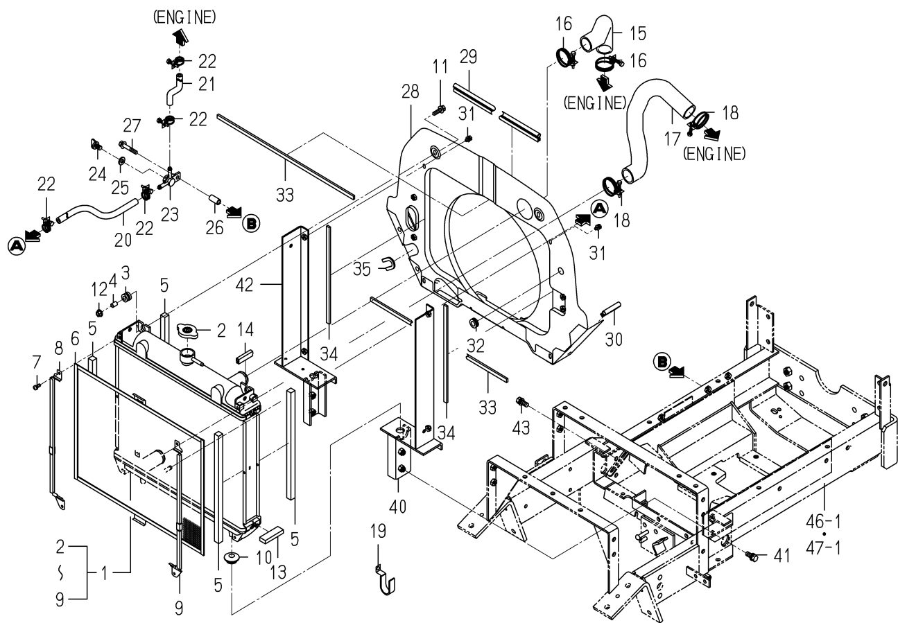
FIG. 2 RADIATOR SYSTEM(1/2)
