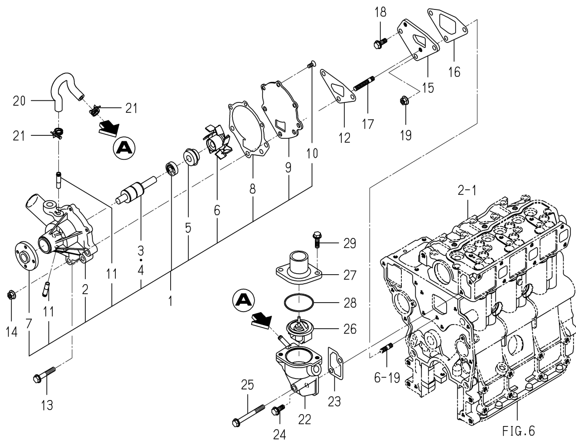
FIG. 18 WATER PUMP
