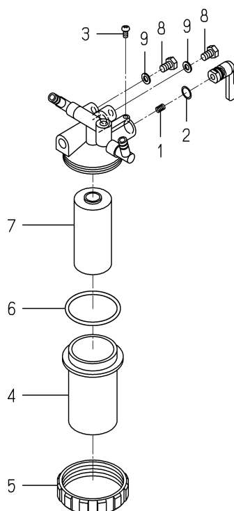
FIG. 99 COMPONENT PARTS FOR 1672-105-210-00 ON Fig.5
