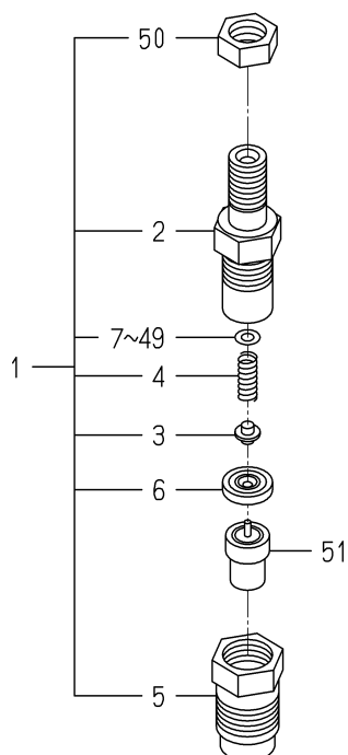
FIG. 28 COMPONENT PARTS FOR 6215-300-036-10 ON Fig.20
