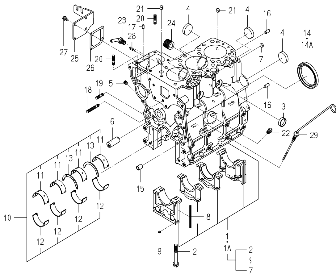
FIG. 6 CYLINDER BLOCK
