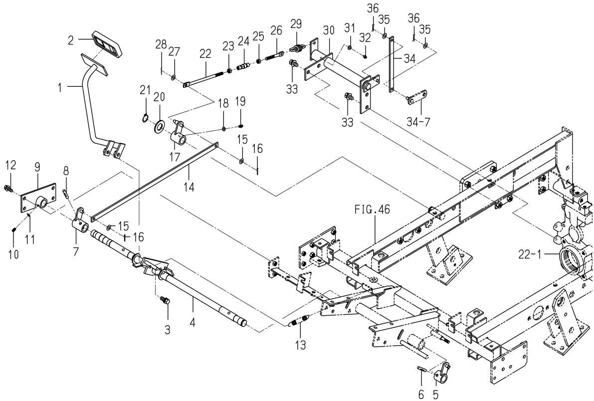
FIG. 36 PEDAL(BRAKE)SYSTEM (SFH220:EXCEPT G TYPE) (SFH240:EXCEPT G TYPE)
