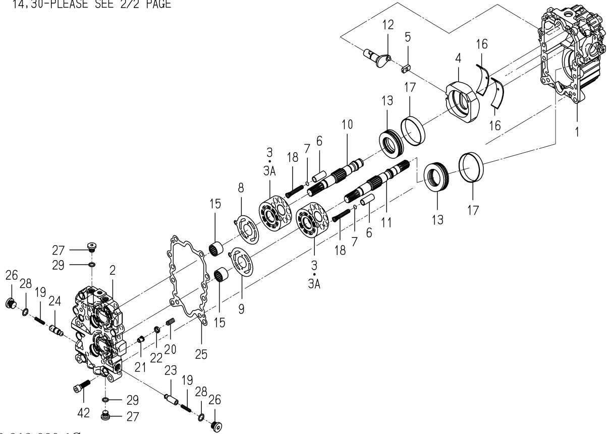
FIG. 98 COMPONENT PARTS(1/2) FOR K510-012-000-10 ON Fig.14,15
