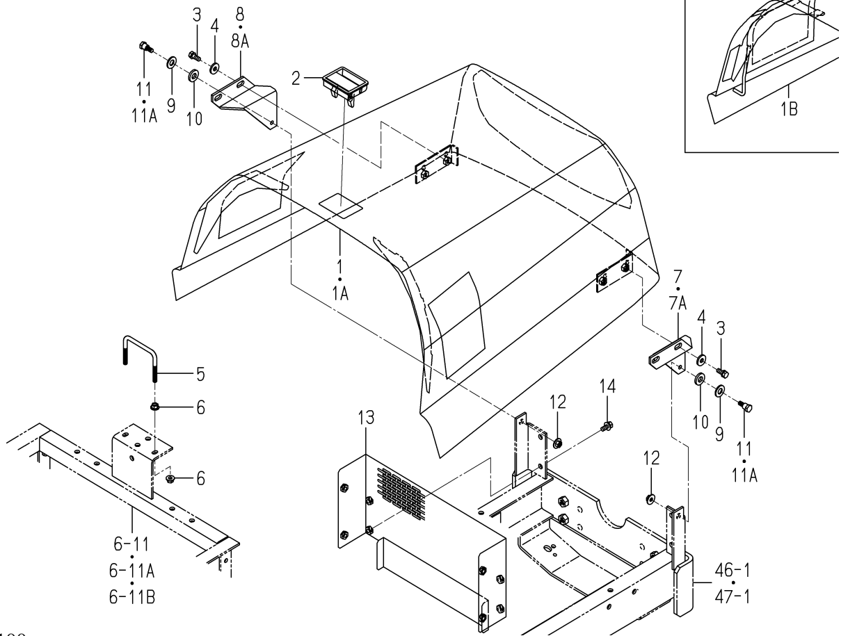
FIG. 67 HOOD SYSTEM
