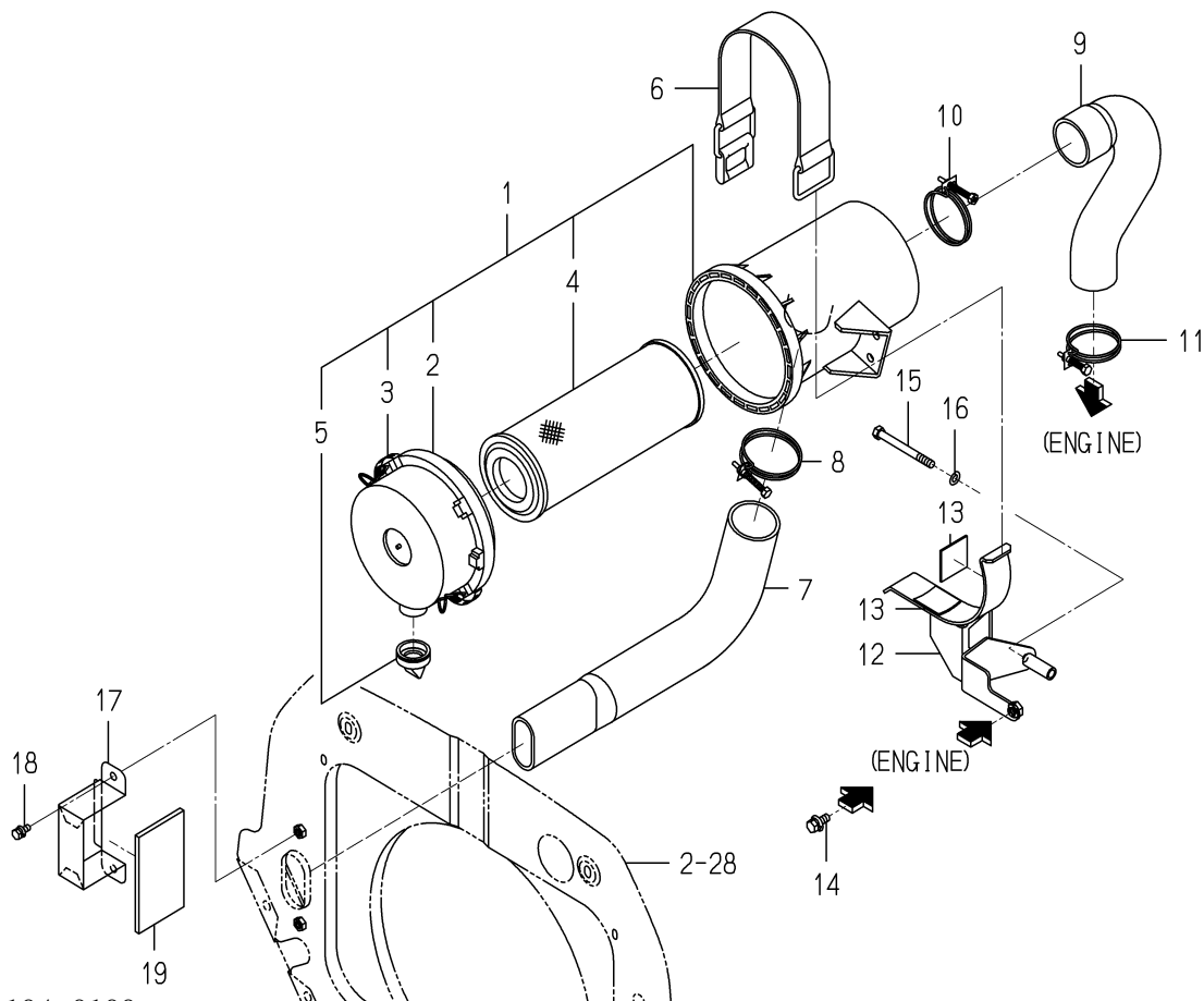
FIG. 4 CLEANER(AIR)SYSTEM
