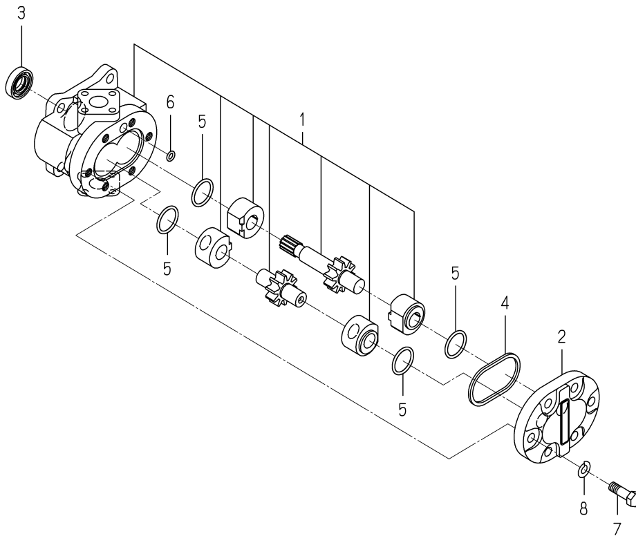
FIG. 97 COMPONENT PARTS FOR K135-023-000-00 ON Fig.61
