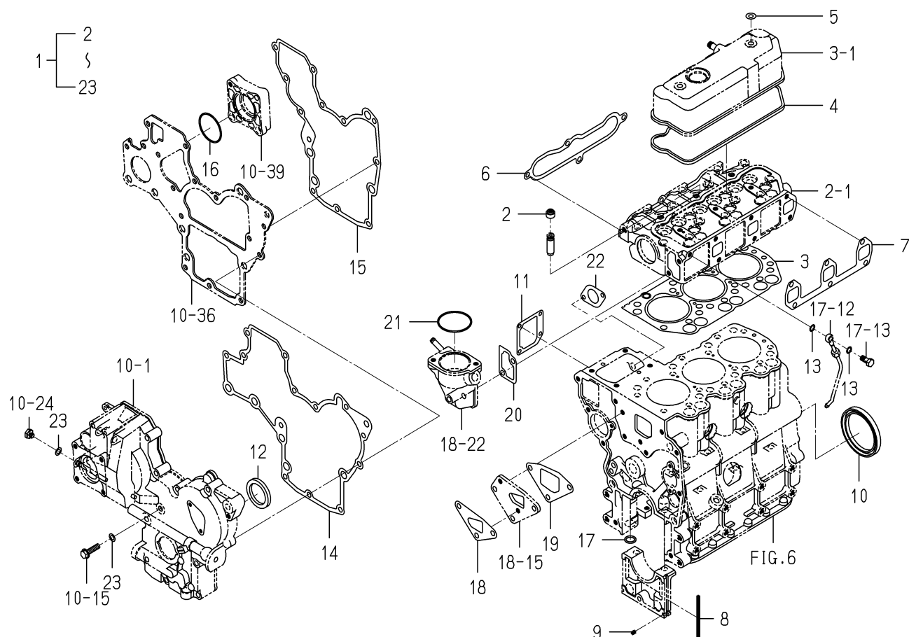
FIG. 27 REPAIR PARTS(OPTION)
