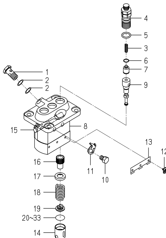
FIG. 29 COMPONENT PARTS FOR 6215-600-103-10 ON Fig.21
