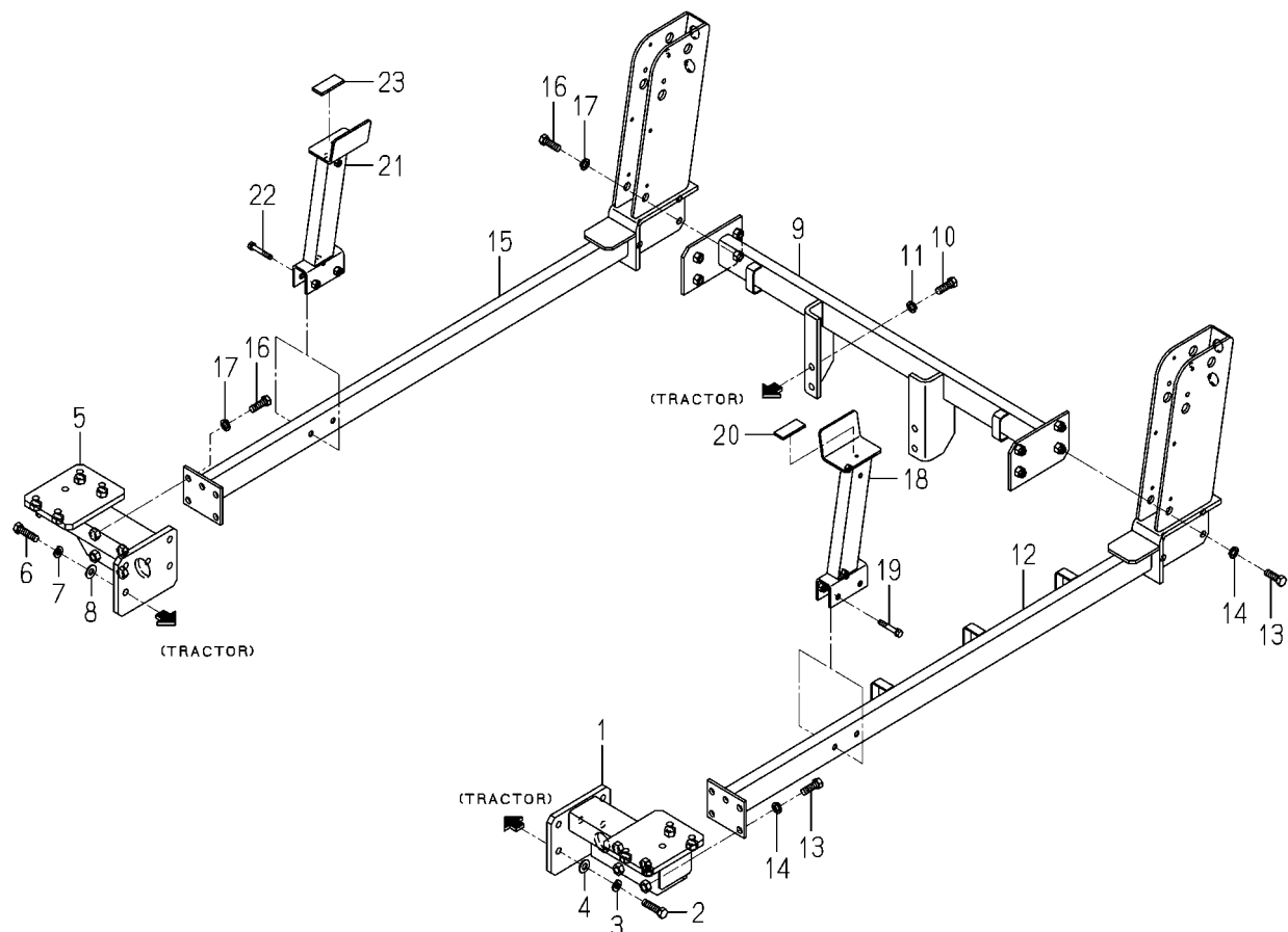
FIG. 2 FRAME SYSTEM(H TYPE)
