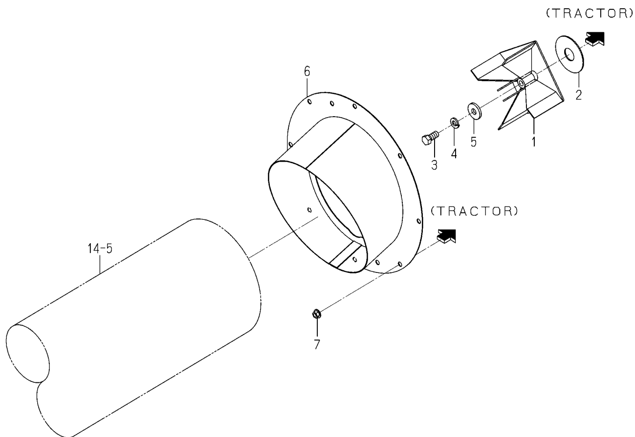
FIG. 15 BLOWER SYSTEM
