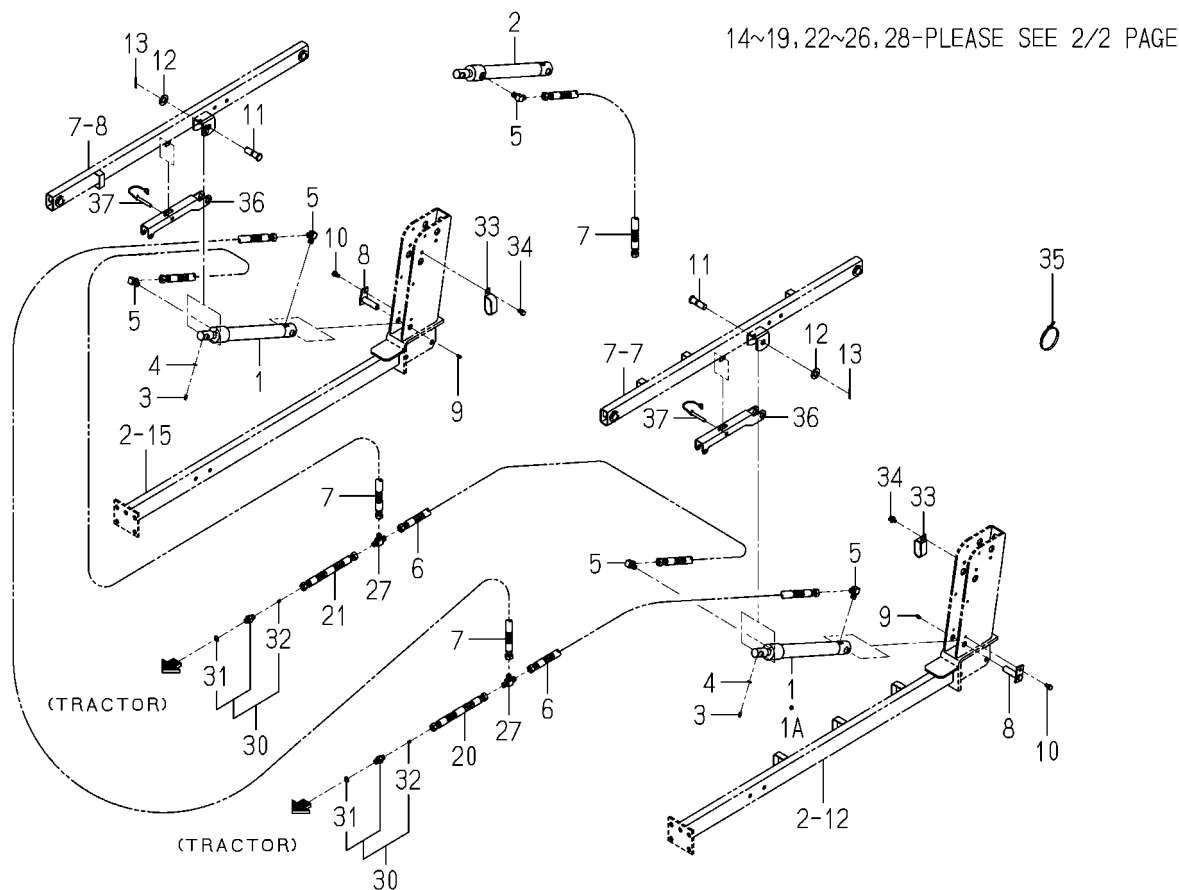
FIG. 9 CYLINDER SYSTEM(H TYPE)(1/2)
