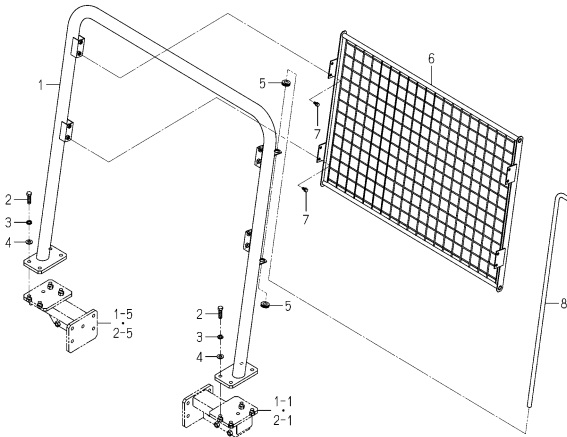
FIG. 16 GUARD SYSTEM
