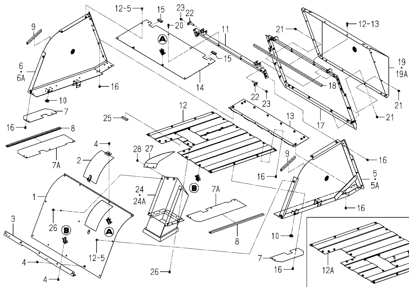
FIG. 3 CONTAINER SYSTEM
