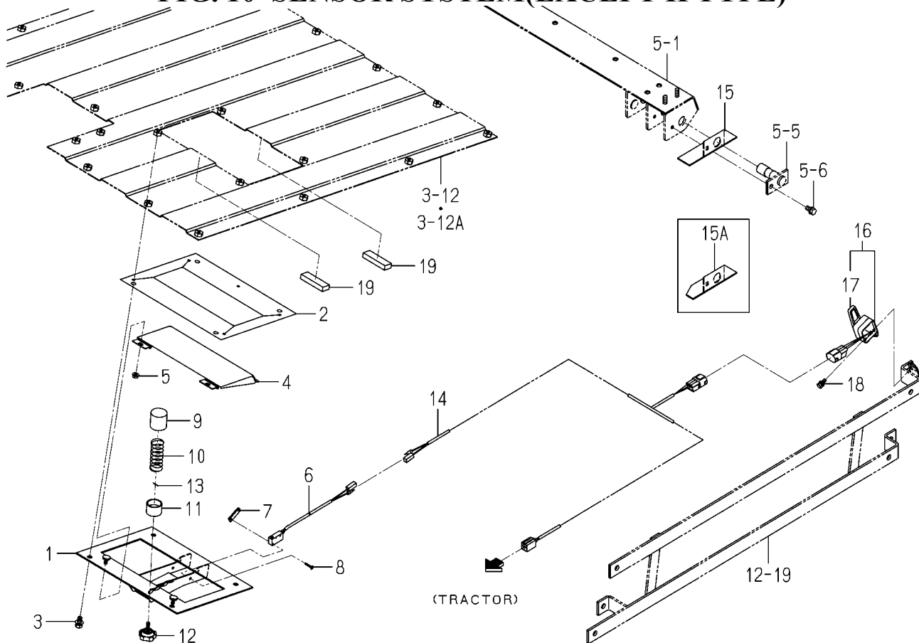
FIG. 10 SENSOR SYSTEM(EXCEPT H TYPE)
