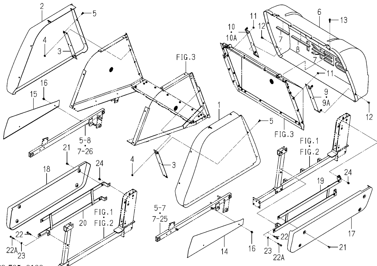
FIG. 12 COVER SYSTEM
