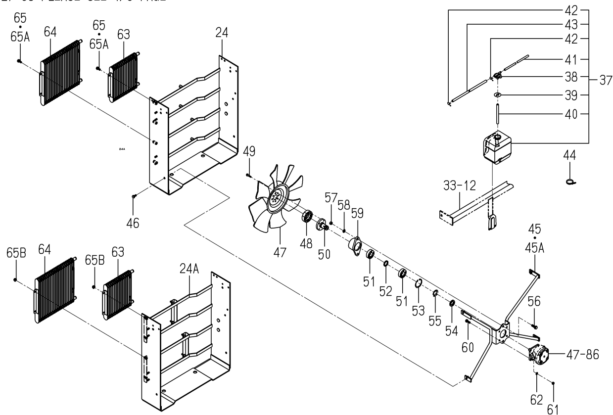
FIG. 2 RADIATOR SYSTEM(438 TYPE)(2/3)
