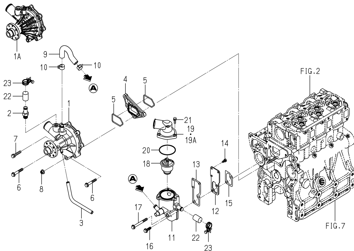
FIG. 20 WATER PUMP
