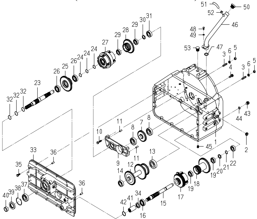
FIG. 14 CASE(TRANSMISSION/FRONT)SYSTEM
