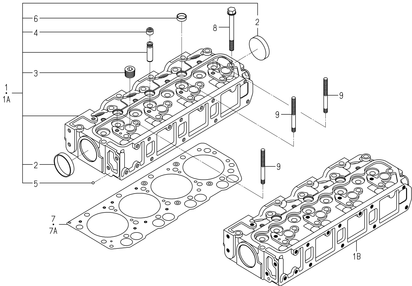
FIG. 2 CYLINDER HEAD
