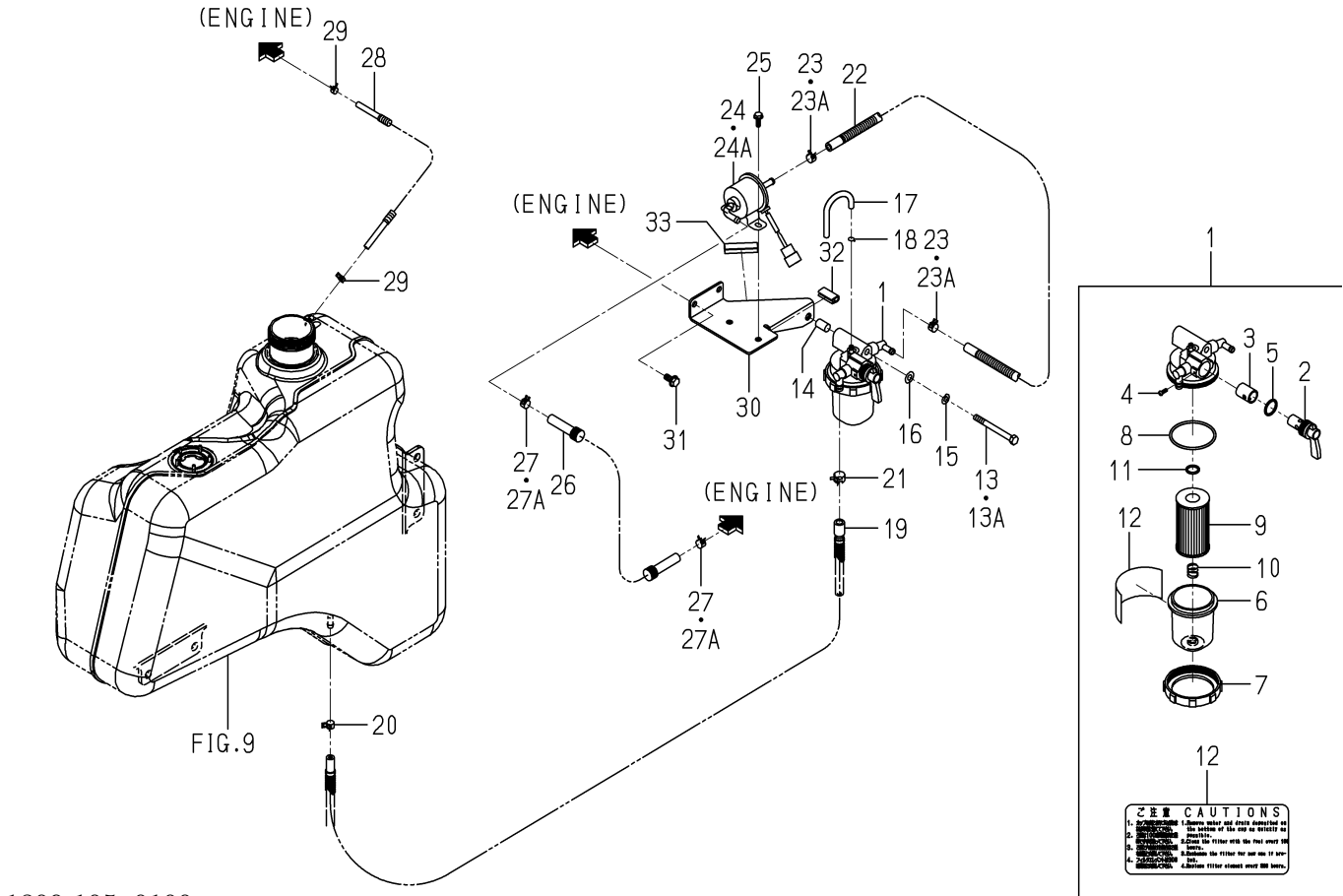
FIG. 7 PIPING(FUEL)SYSTEM(450 TYPE)
