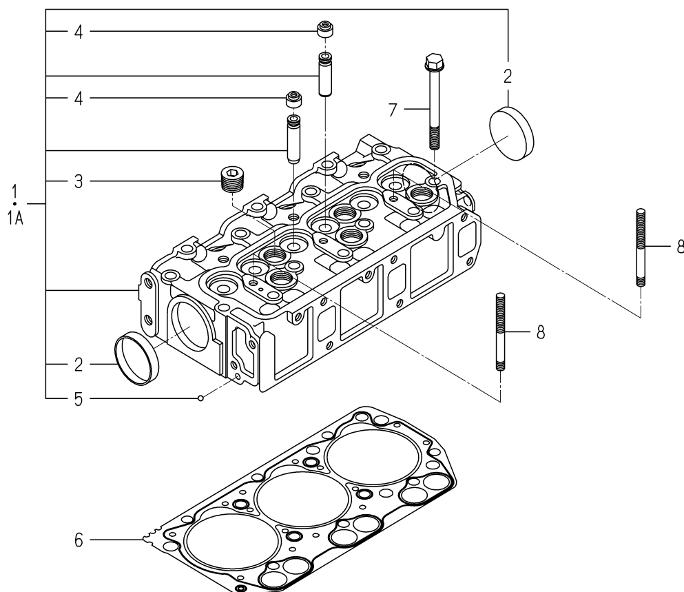
FIG. 2 CYLINDER HEAD
