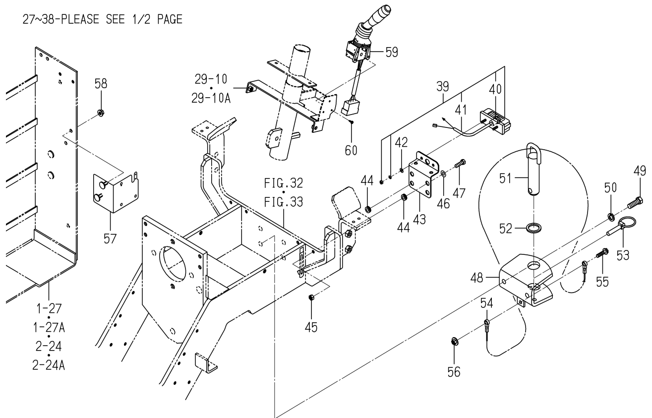
FIG. 55 LIGHT SYSTEM(2/2)
