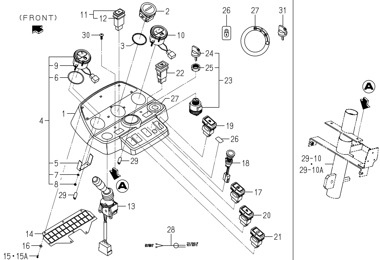
FIG. 56 PANEL SYSTEM
