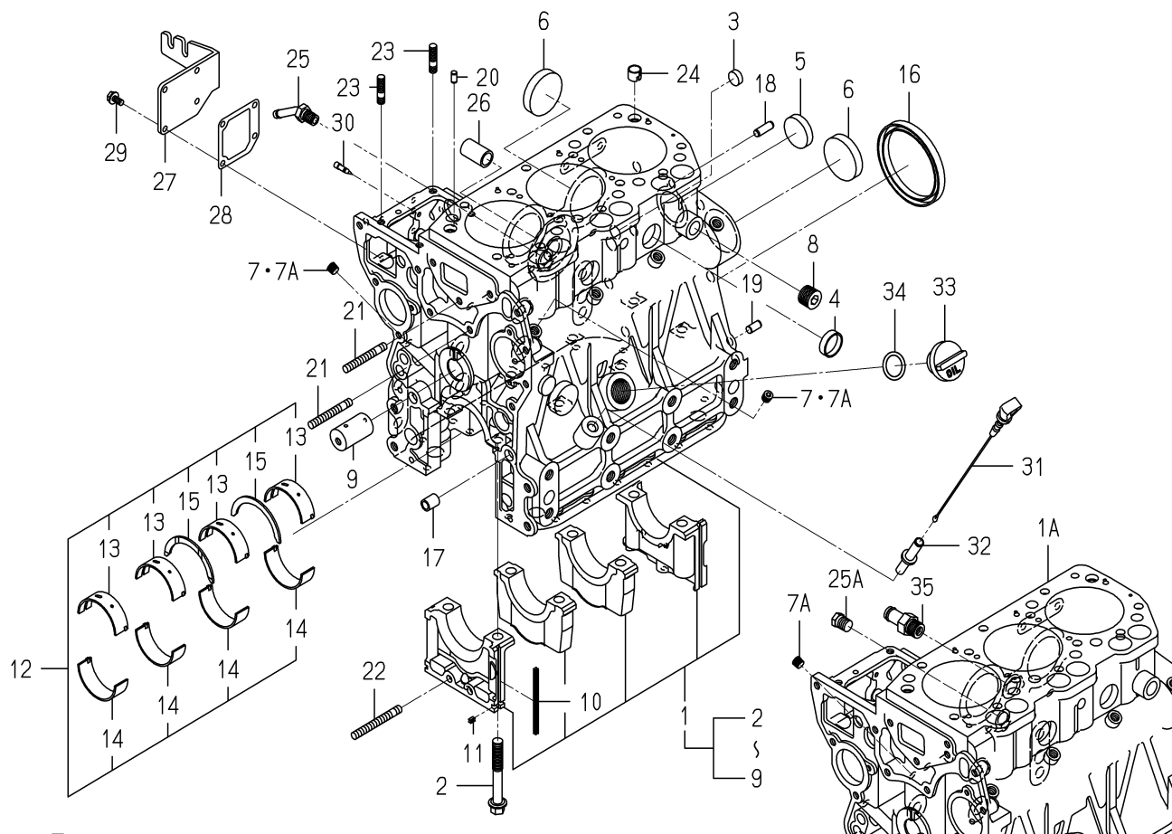
FIG. 7 CYLINDER BLOCK
