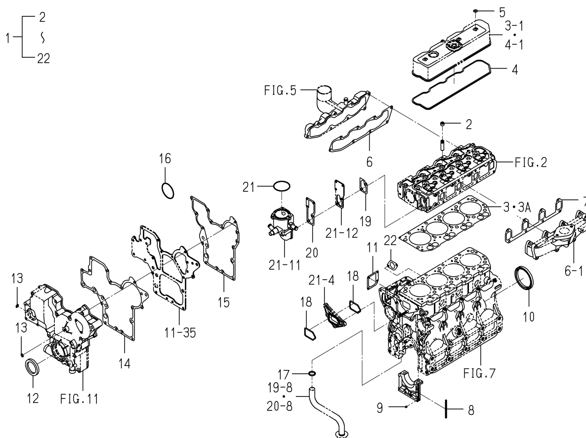
FIG. 30 REPAIR PARTS(OPTION)
