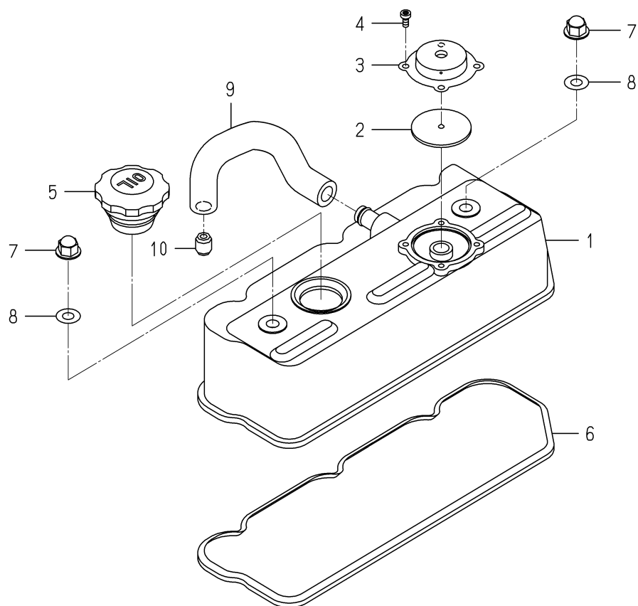
FIG. 4 CYLINDER HEAD COVER
