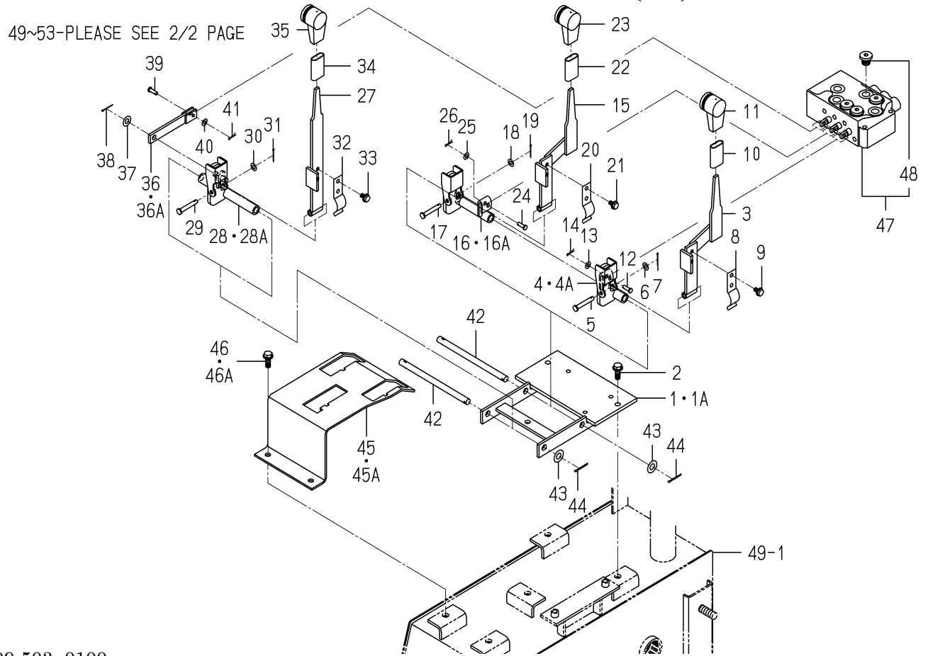
FIG. 43 CONTROL SYSTEM(1/2)
