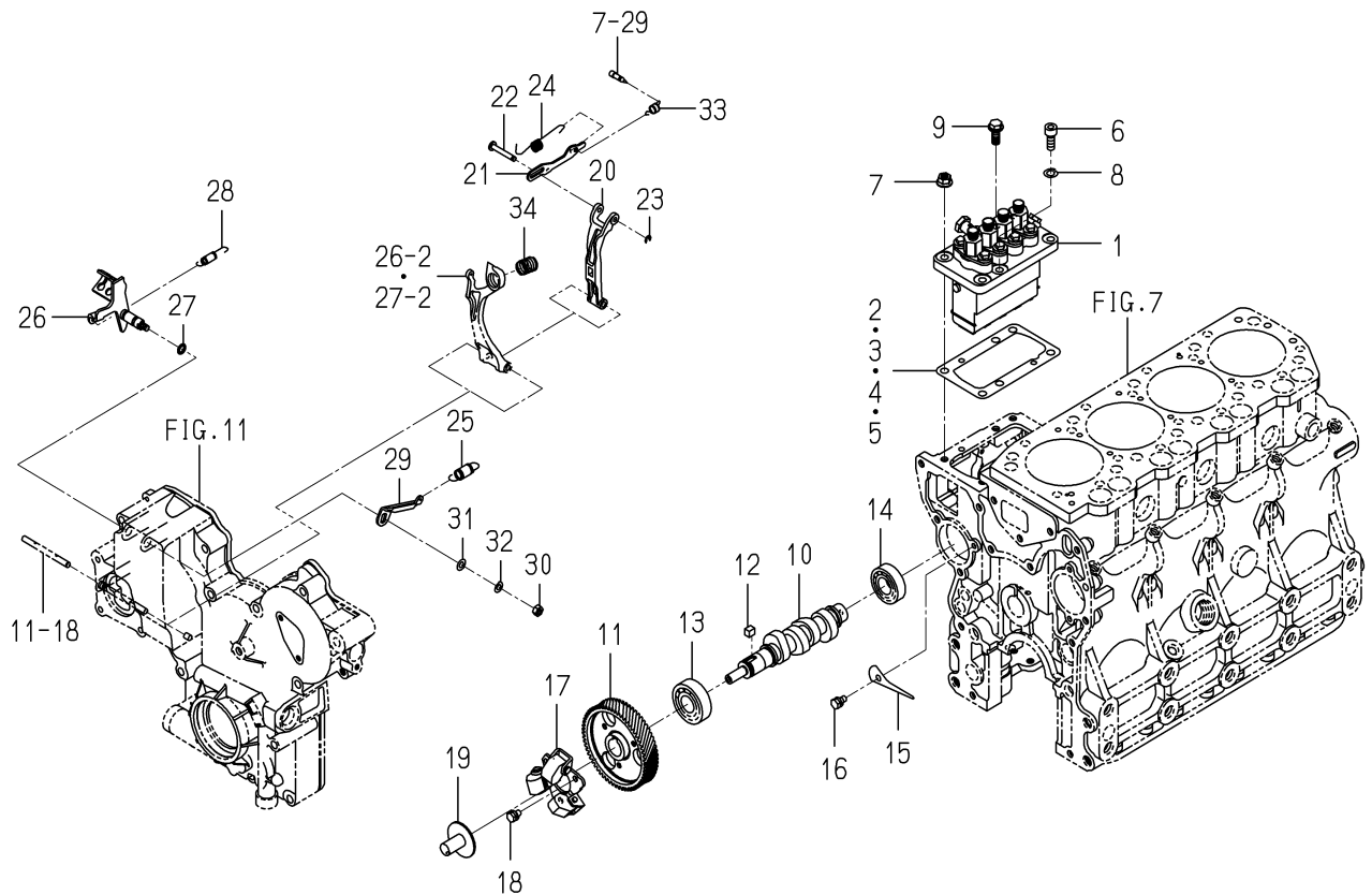
FIG. 24 INJECTION PUMP
