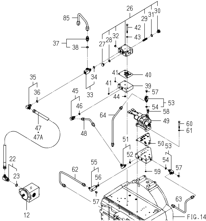
FIG. 47 PIPING(CONTROL)SYSTEM(2/3)
