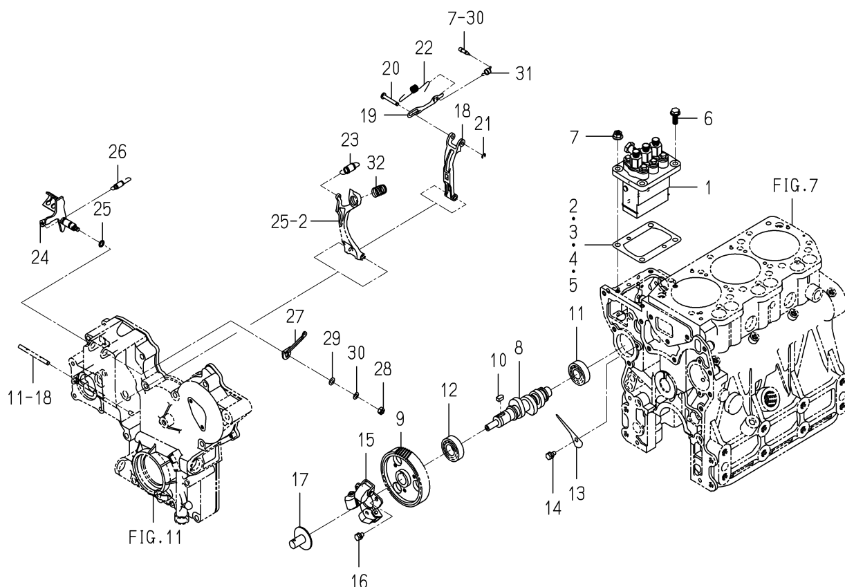
FIG. 23 INJECTION PUMP
