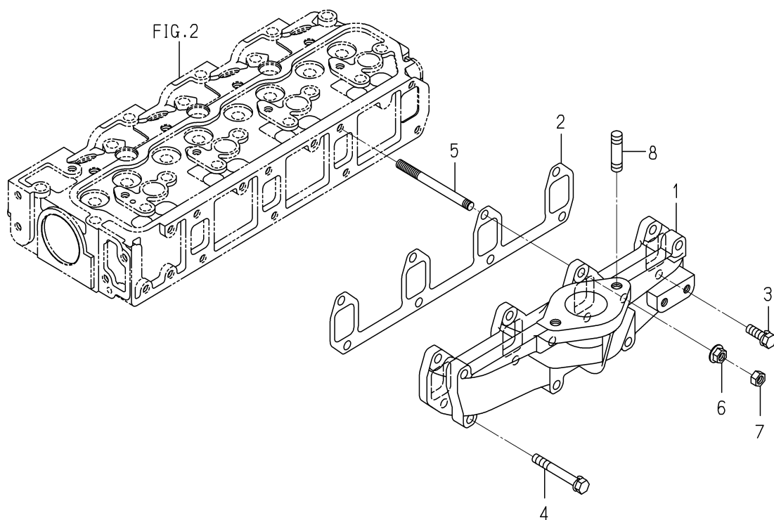
FIG. 6 EXHAUST MANIFOLD
