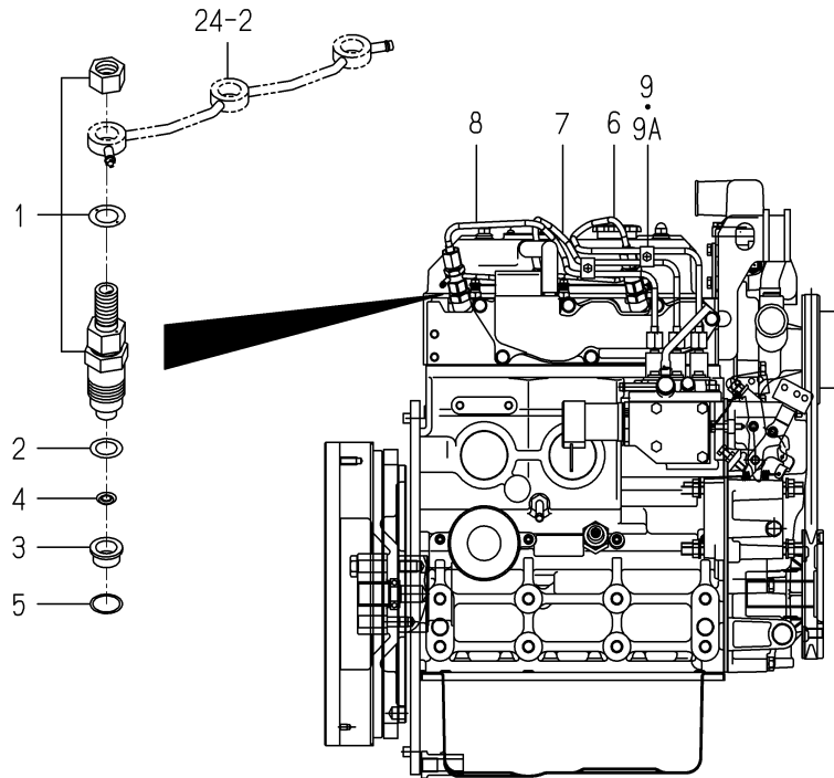
FIG. 22 INJECTION NOZZLE
