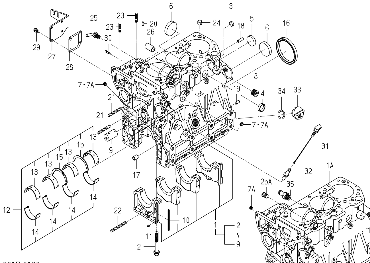
FIG. 7 CYLINDER BLOCK
