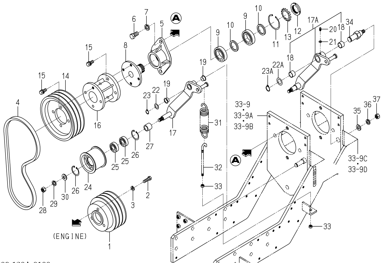
FIG. 13 PULLEY(INPUT)SYSTEM(438 TYPE)
