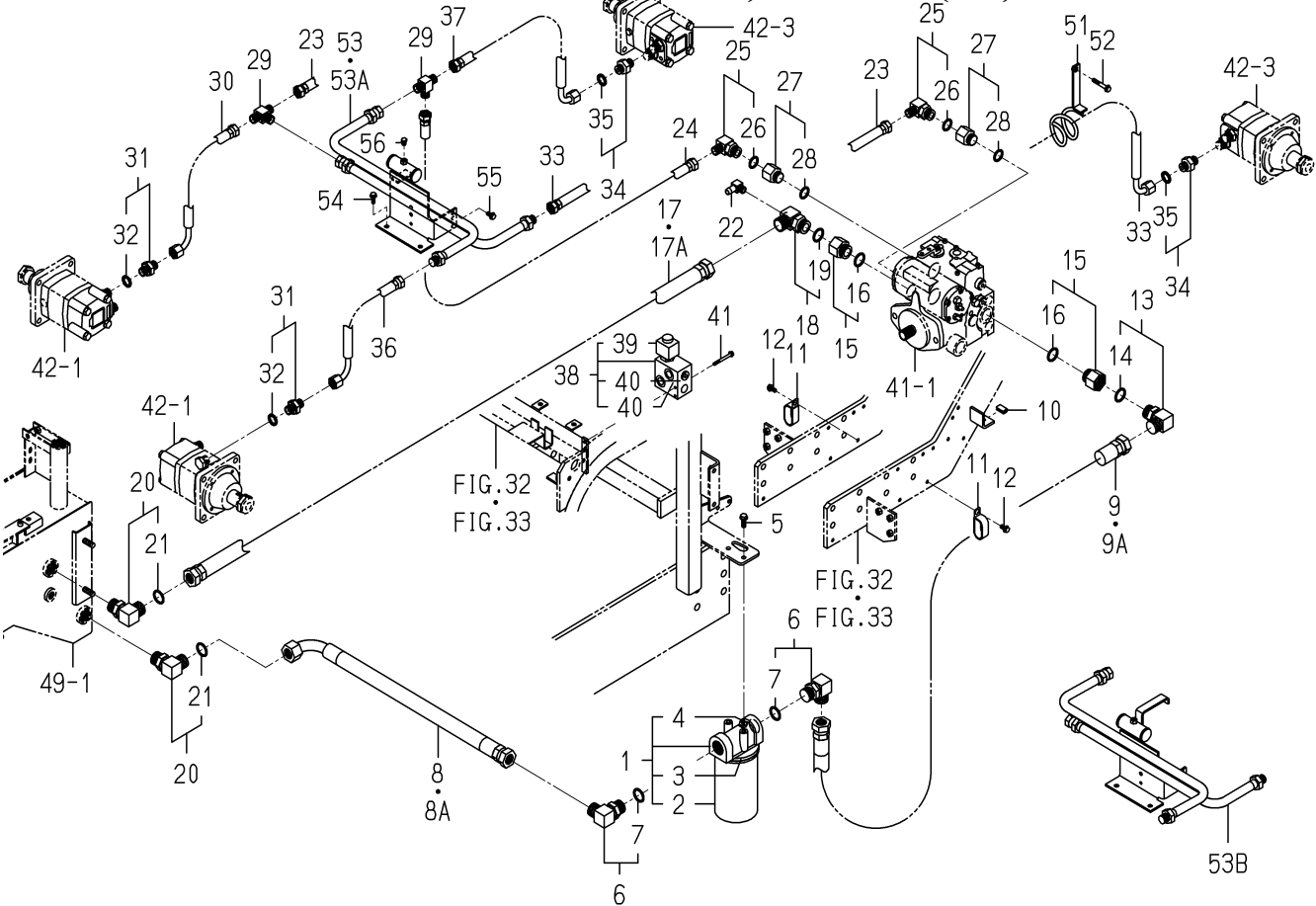
FIG. 46 PIPING(PUMP)SYSTEM(1/2)
