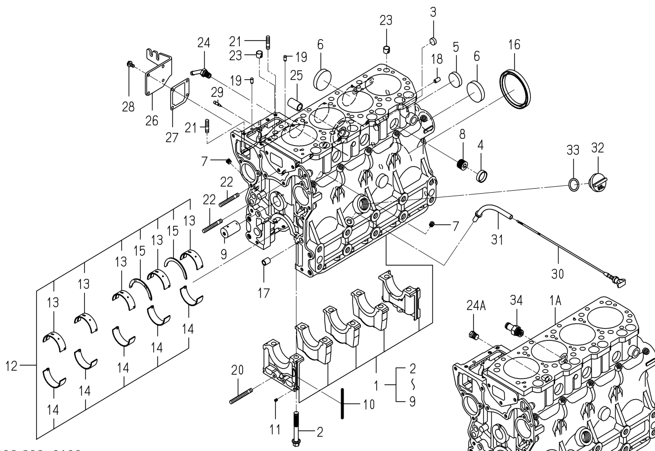
FIG. 7 CYLINDER BLOCK
