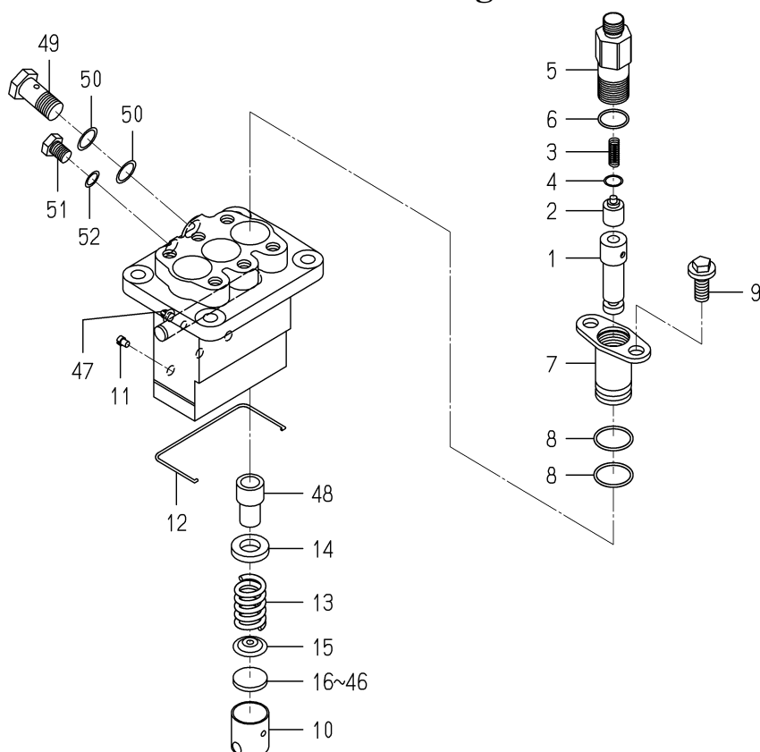
FIG. 30 COMPONENT PARTS FOR 6215-600-104-20 ON Fig.023
