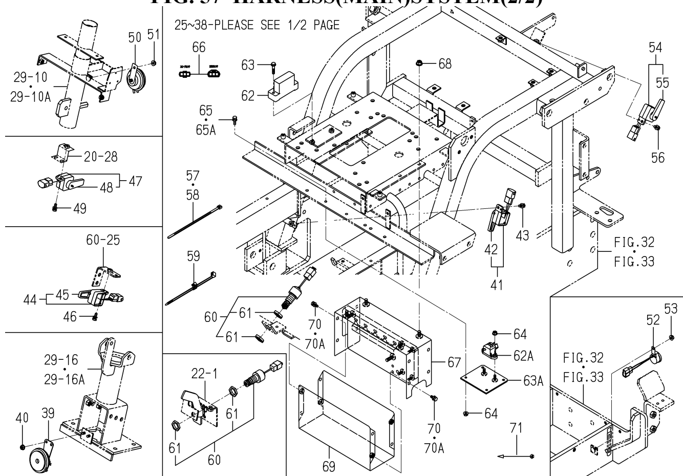
FIG. 57 HARNESS(MAIN)SYSTEM(2/2)
