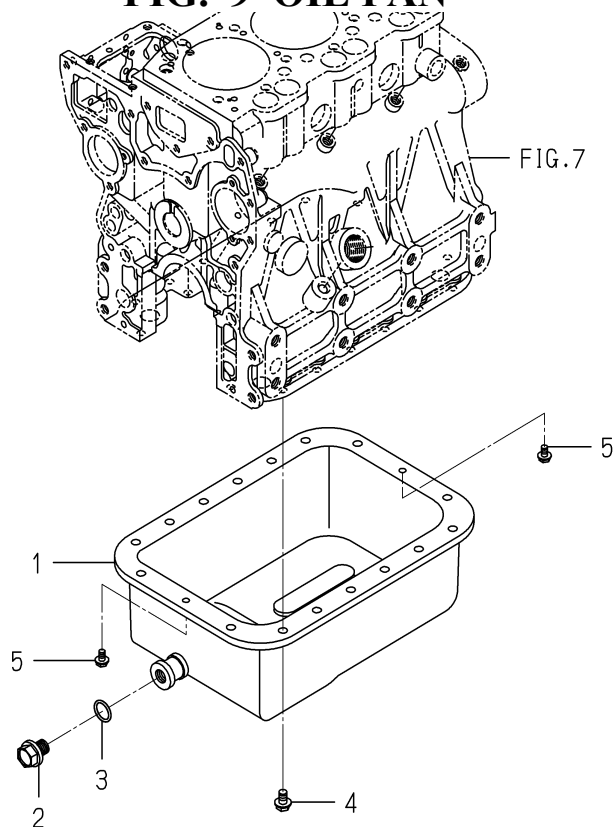
FIG. 9 OIL PAN
