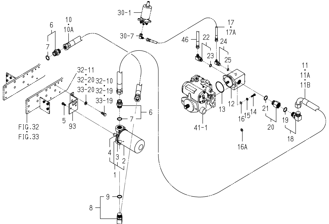
FIG. 47 PIPING(CONTROL)SYSTEM(1/3)
