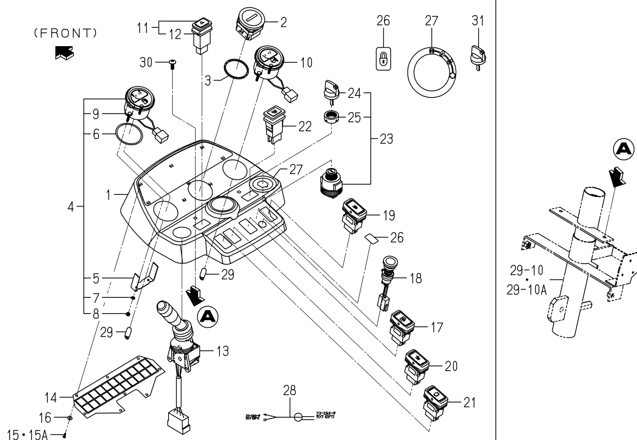
FIG. 56 PANEL SYSTEM
