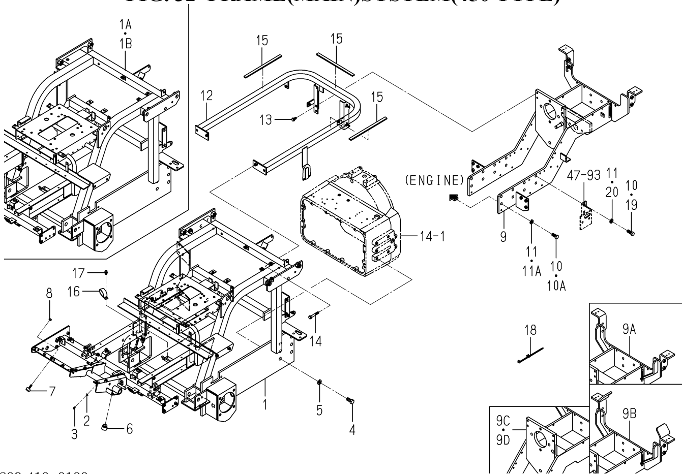
FIG. 32 FRAME(MAIN)SYSTEM(450 TYPE)
