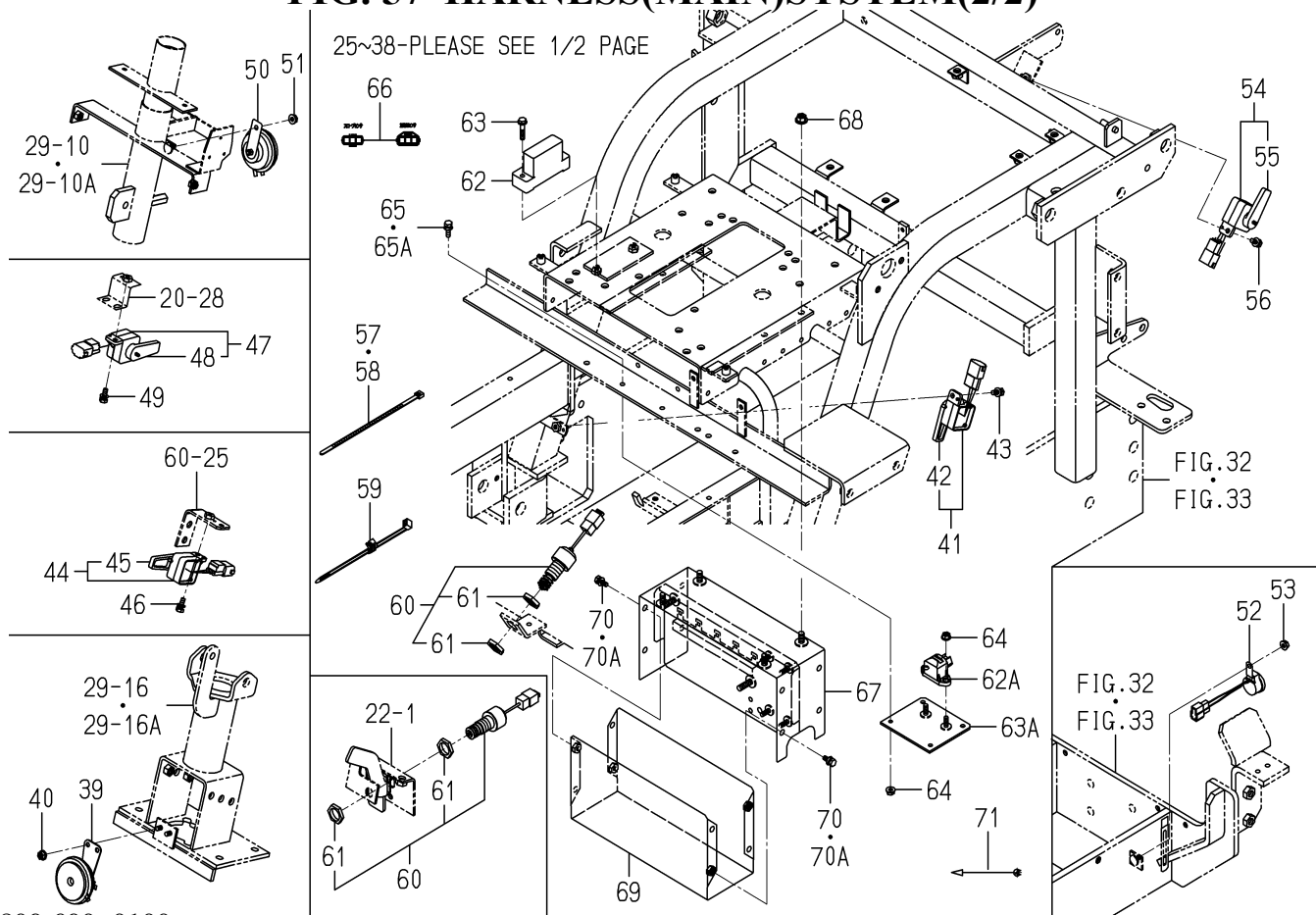
FIG. 57 HARNESS(MAIN)SYSTEM(2/2)
