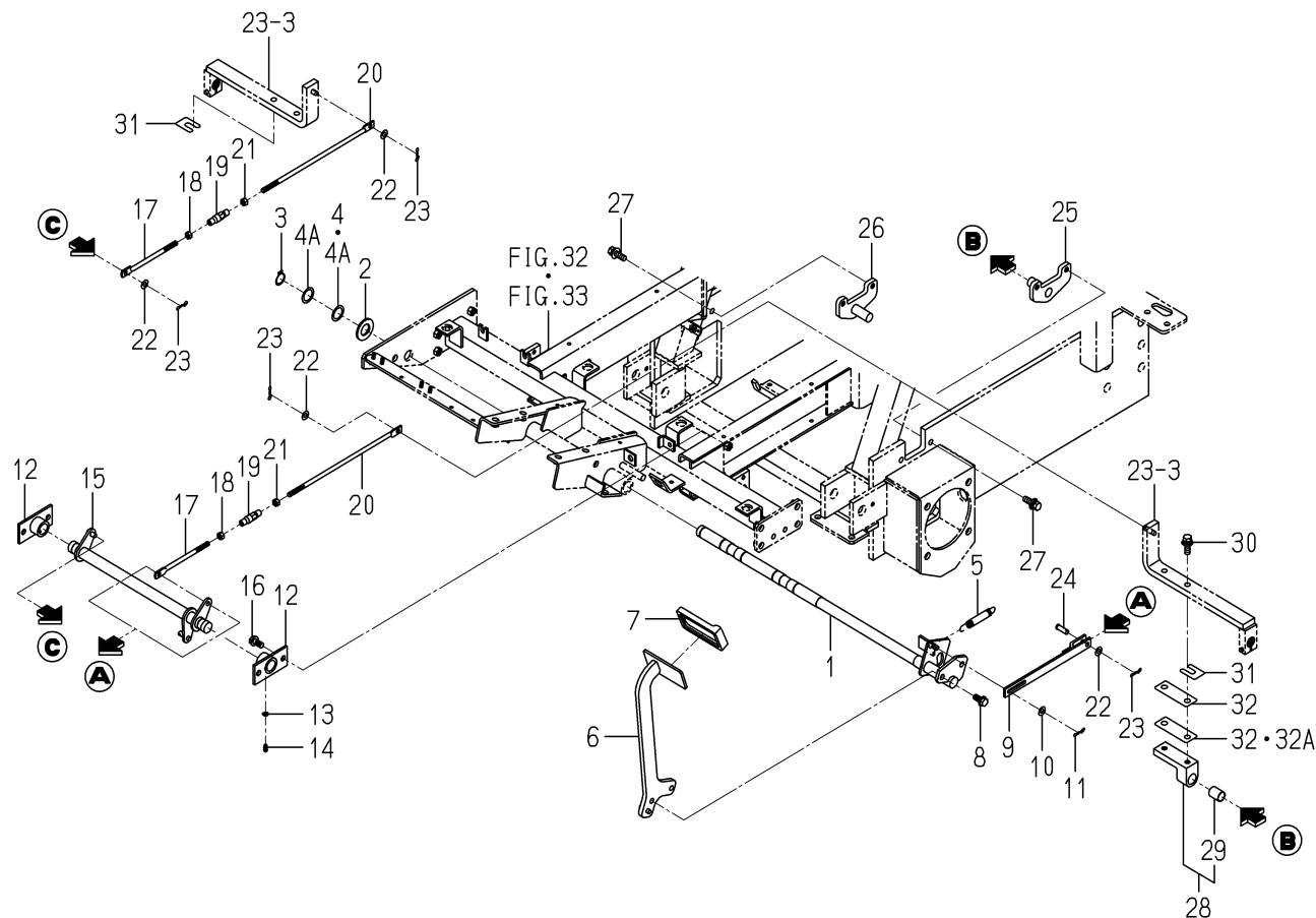
FIG. 24 PEDAL(BRAKE)SYSTEM
