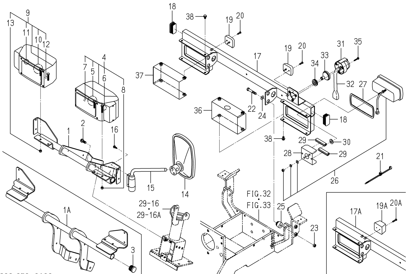
FIG. 55 LIGHT SYSTEM(1/2)
