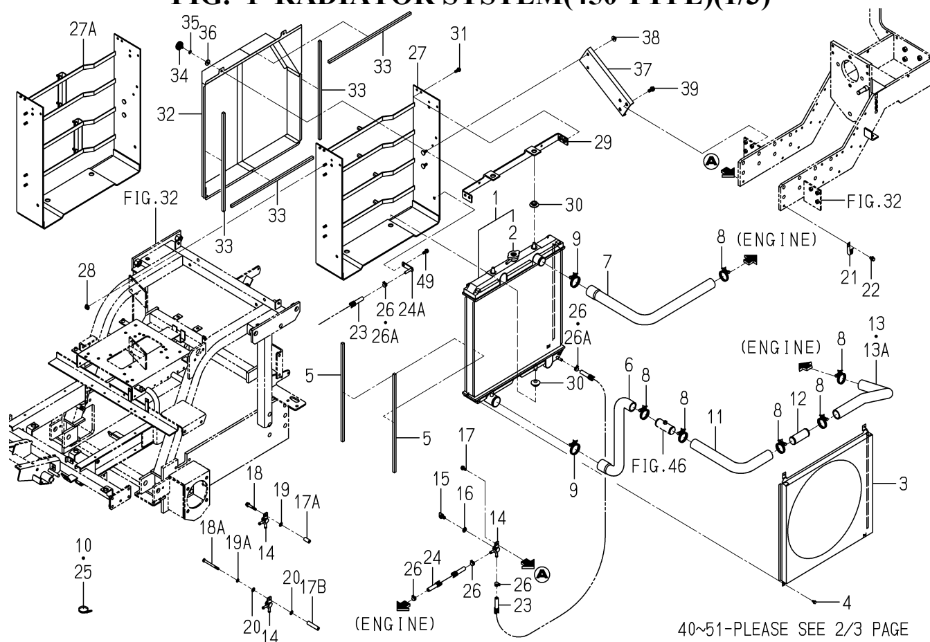
FIG. 1 RADIATOR SYSTEM(450 TYPE)(1/3)
