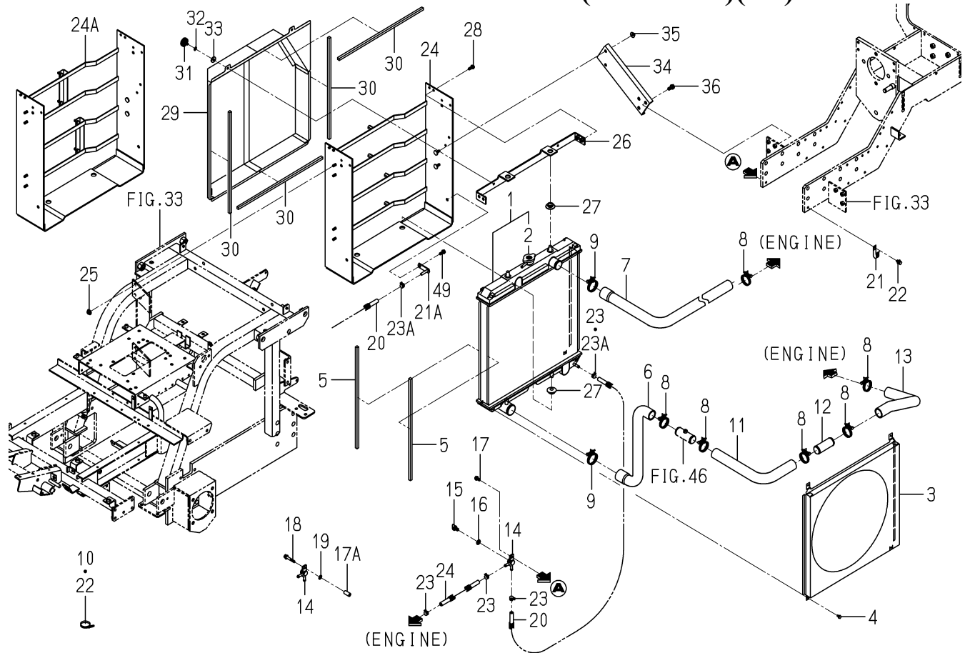
FIG. 2 RADIATOR SYSTEM(438 TYPE)(1/3)
