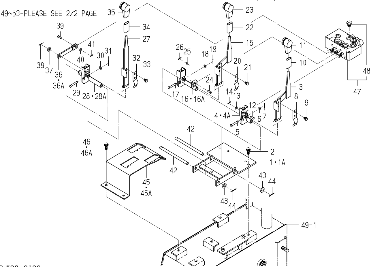
FIG. 43 CONTROL SYSTEM(1/2)
