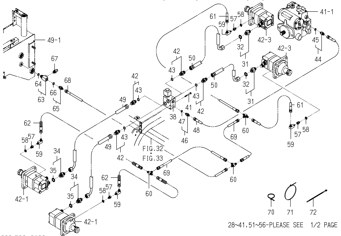
FIG. 46 PIPING(PUMP)SYSTEM(2/2)
