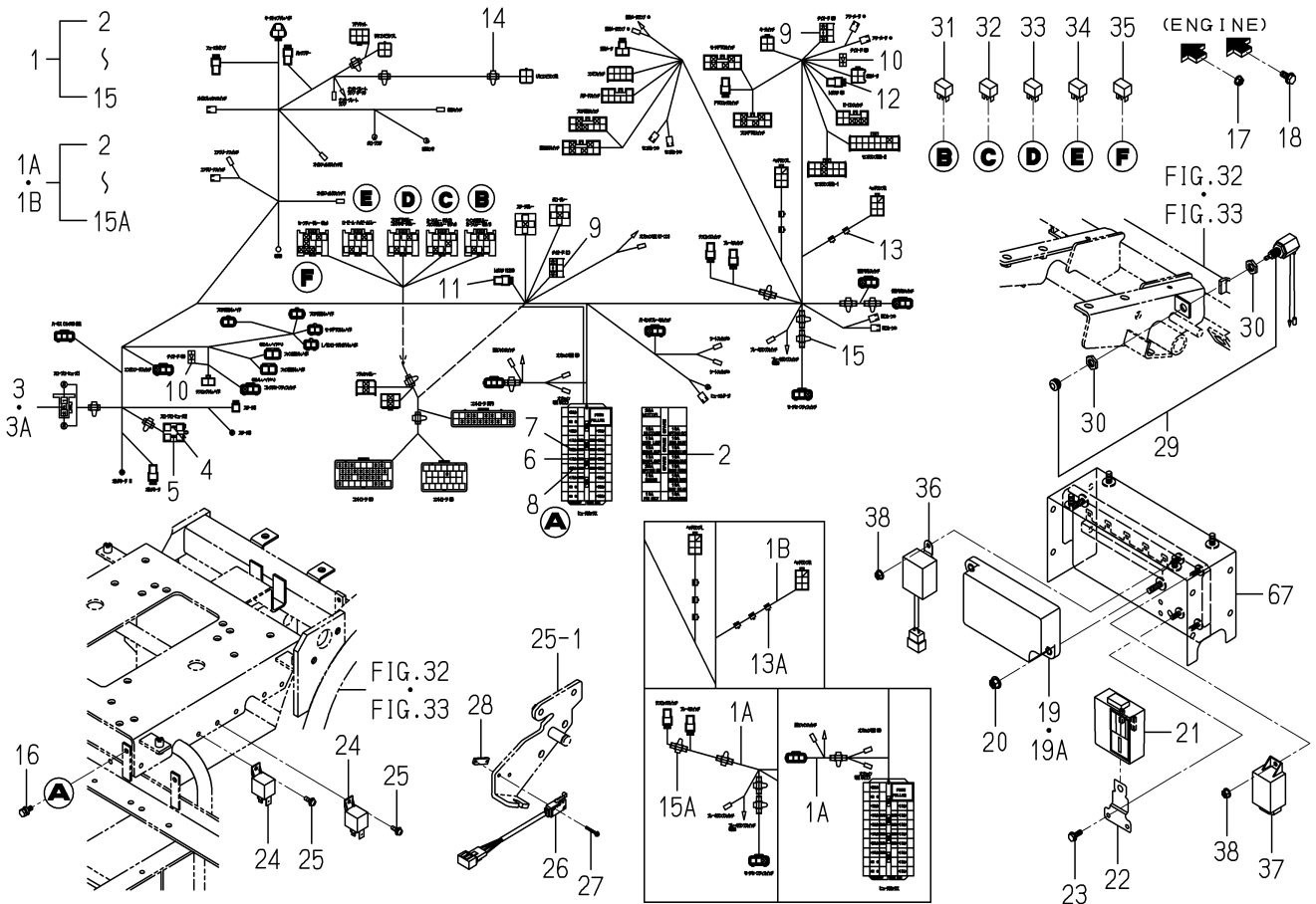
FIG. 57 HARNESS(MAIN)SYSTEM(1/2)
