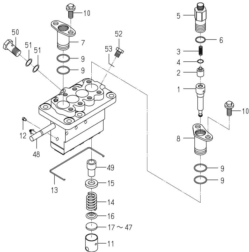
FIG. 32 COMPONENT PARTS FOR 6215-600-119-20 ON Fig.024
