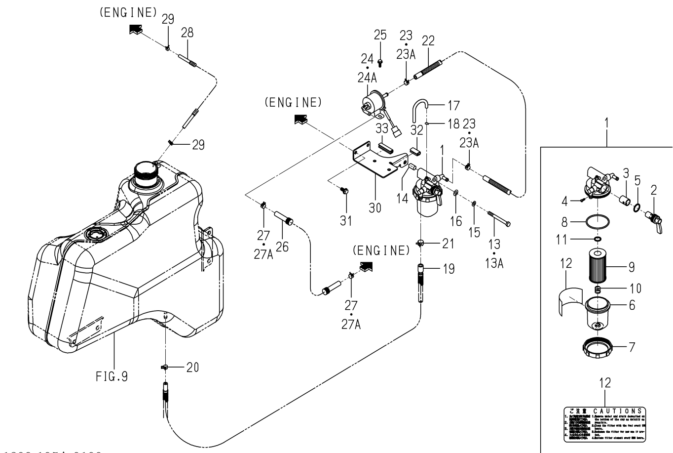
FIG. 8 PIPING(FUEL)SYSTEM(438 TYPE)
