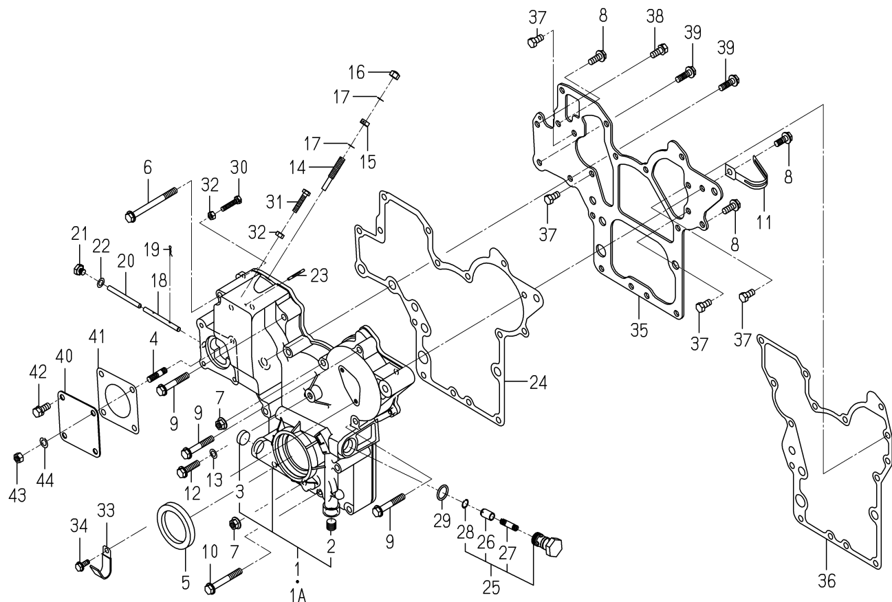
FIG. 11 TIMING GEAR CASE
