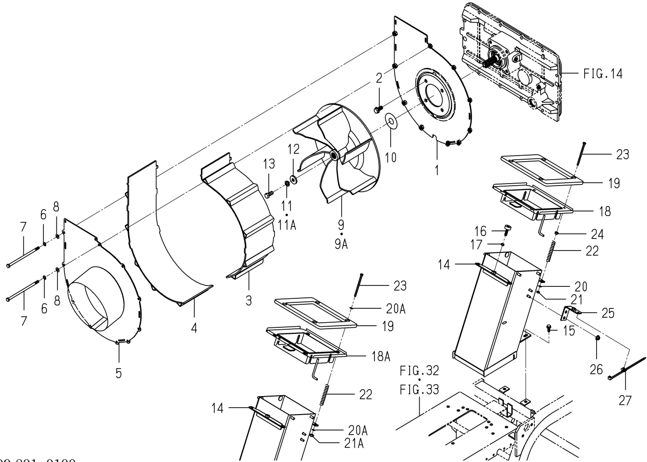
FIG. 60 BLOWER SYSTEM
