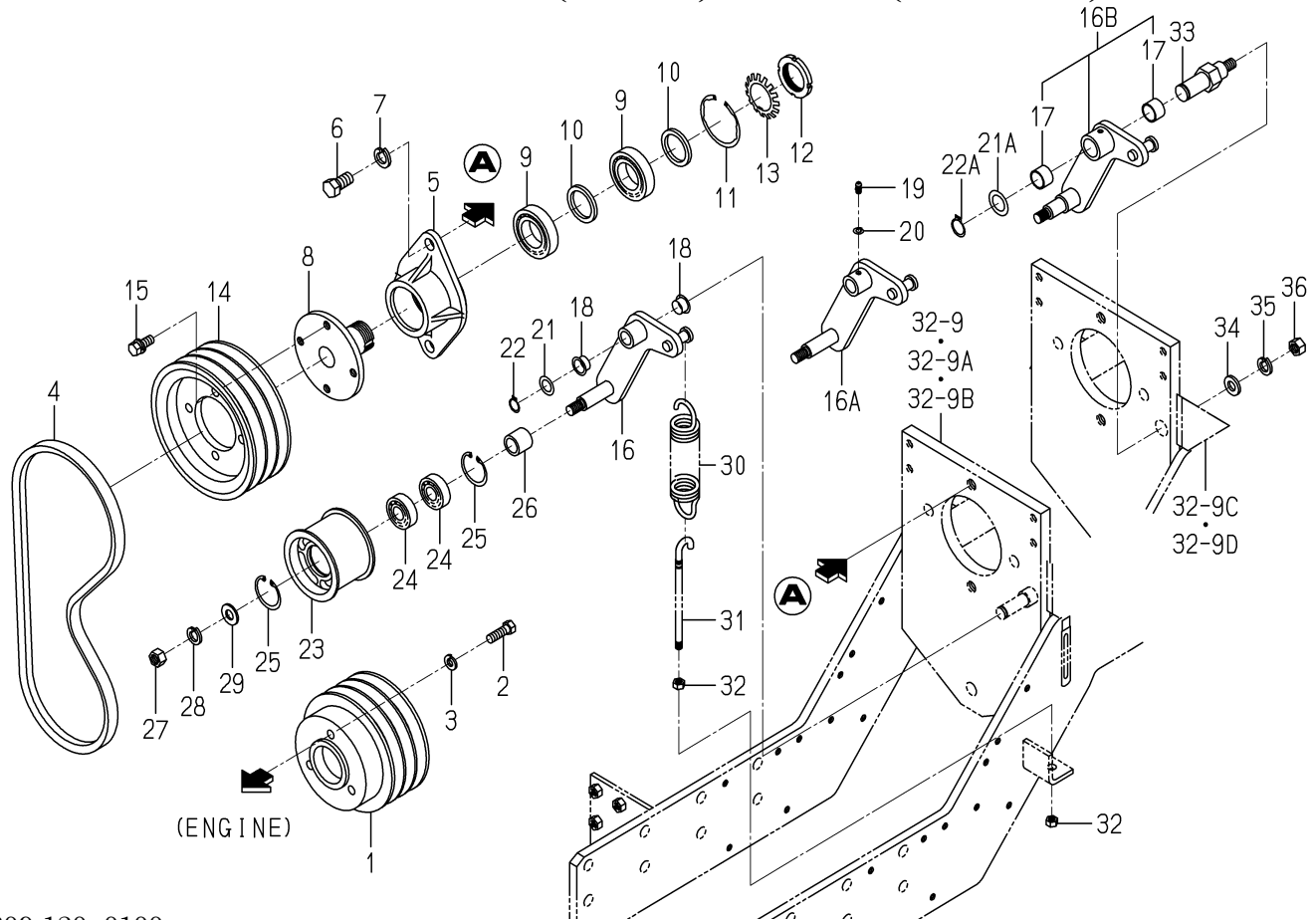
FIG. 12 PULLEY(INPUT)SYSTEM(450 TYPE)
