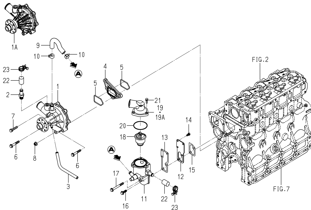
FIG. 21 WATER PUMP
