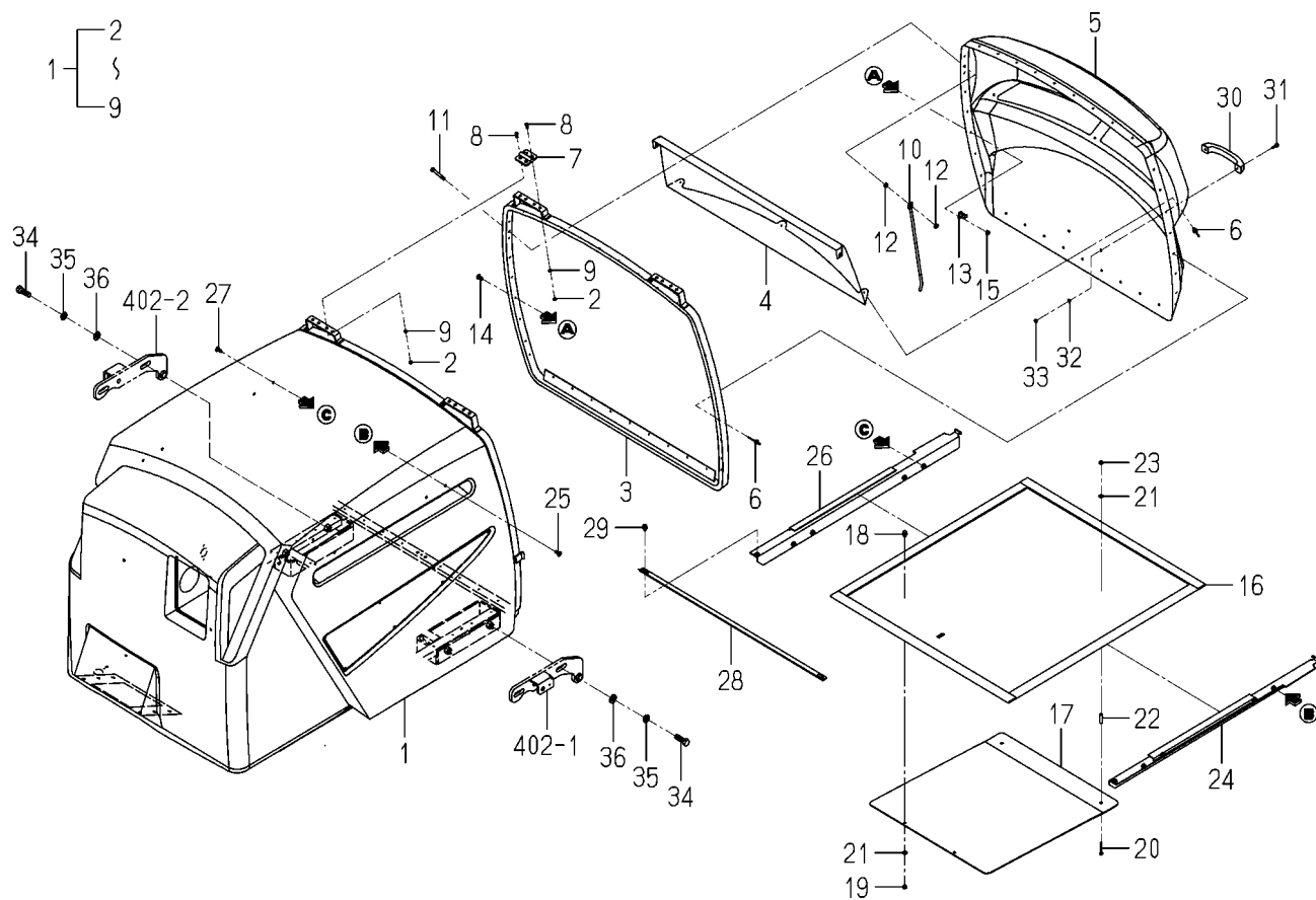
FIG.301 FRAME SYSTEM
