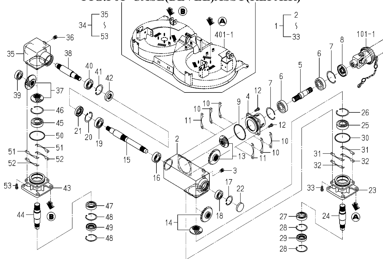
FIG.P01 CASE(BEVEL)ASSY(REPAIR)
