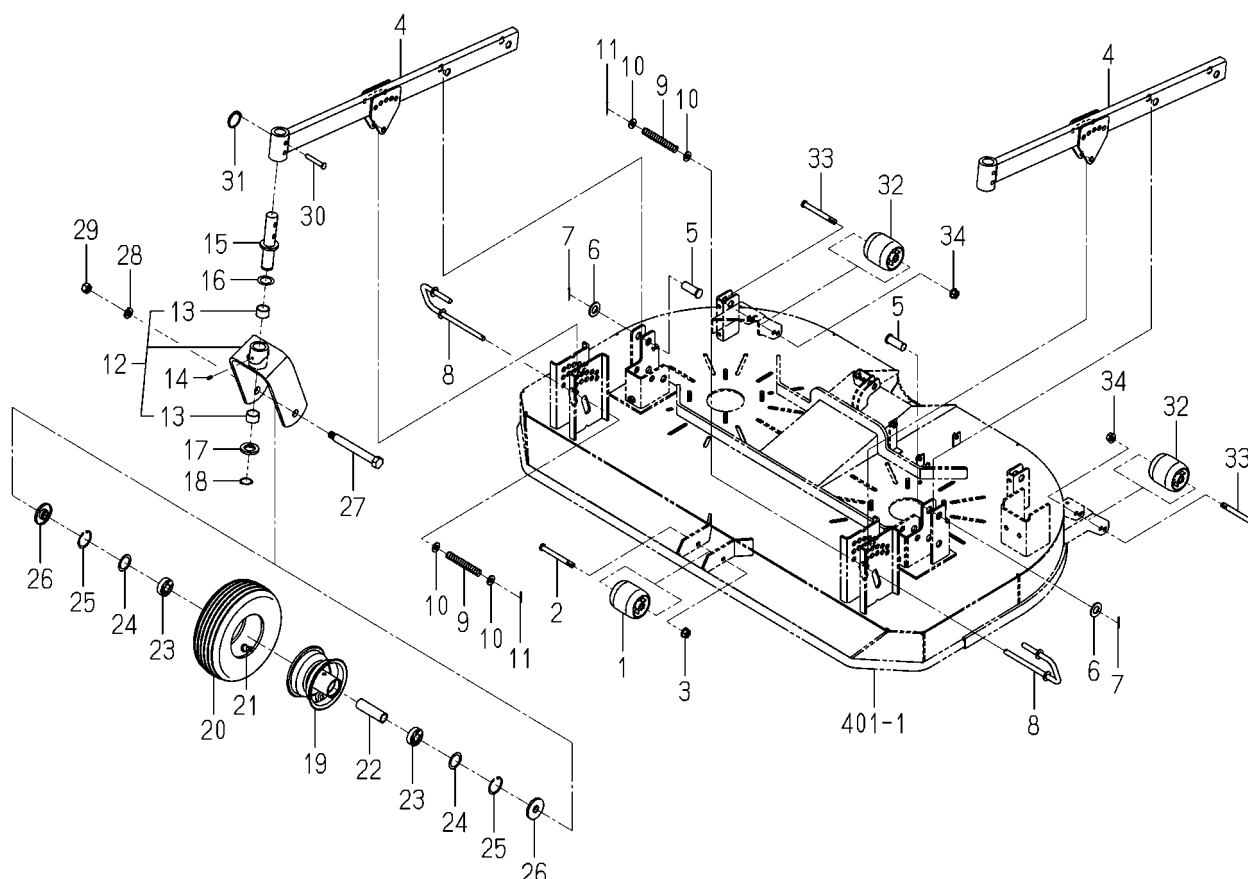
FIG.501 WHEEL(GAUGE)SYSTEM
