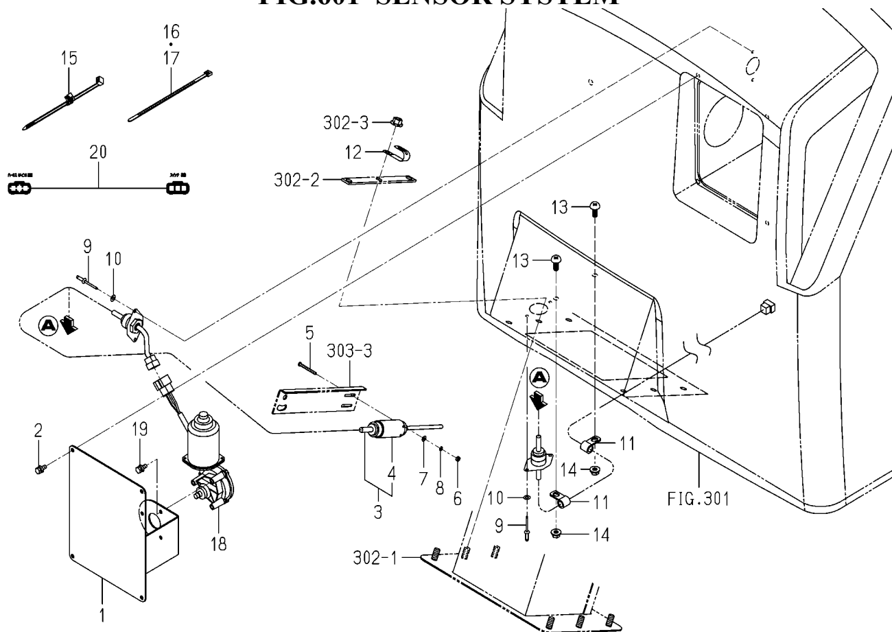
FIG.601 SENSOR SYSTEM
