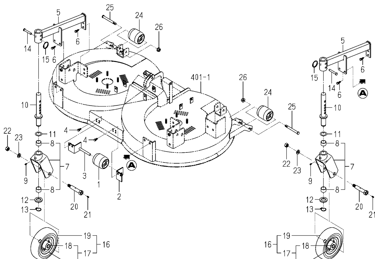
FIG.501 WHEEL(GAUGE)SYSTEM
