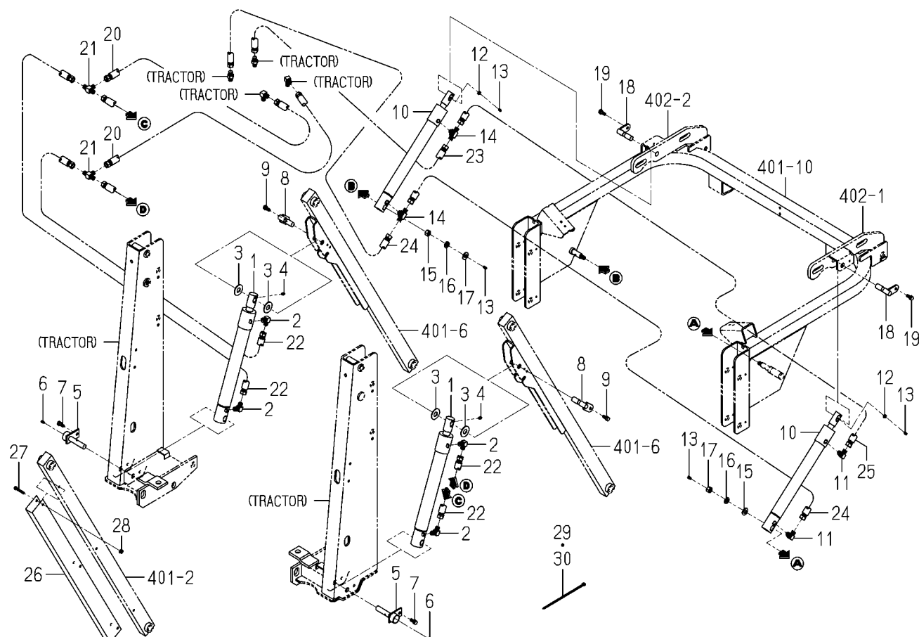
FIG.501 CYLINDER SYSTEM
