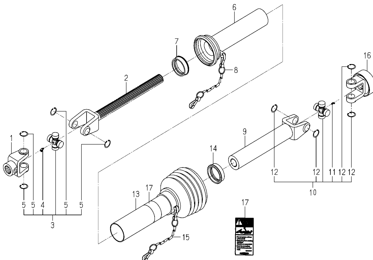
FIG.S01 COMPONENT PARTS FOR 8667-101-310-00 ON Fig.101
