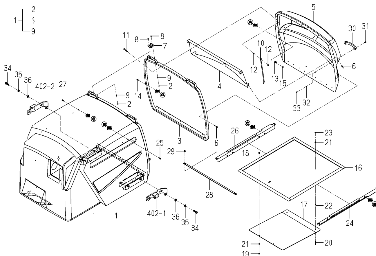
FIG.301 FRAME SYSTEM
