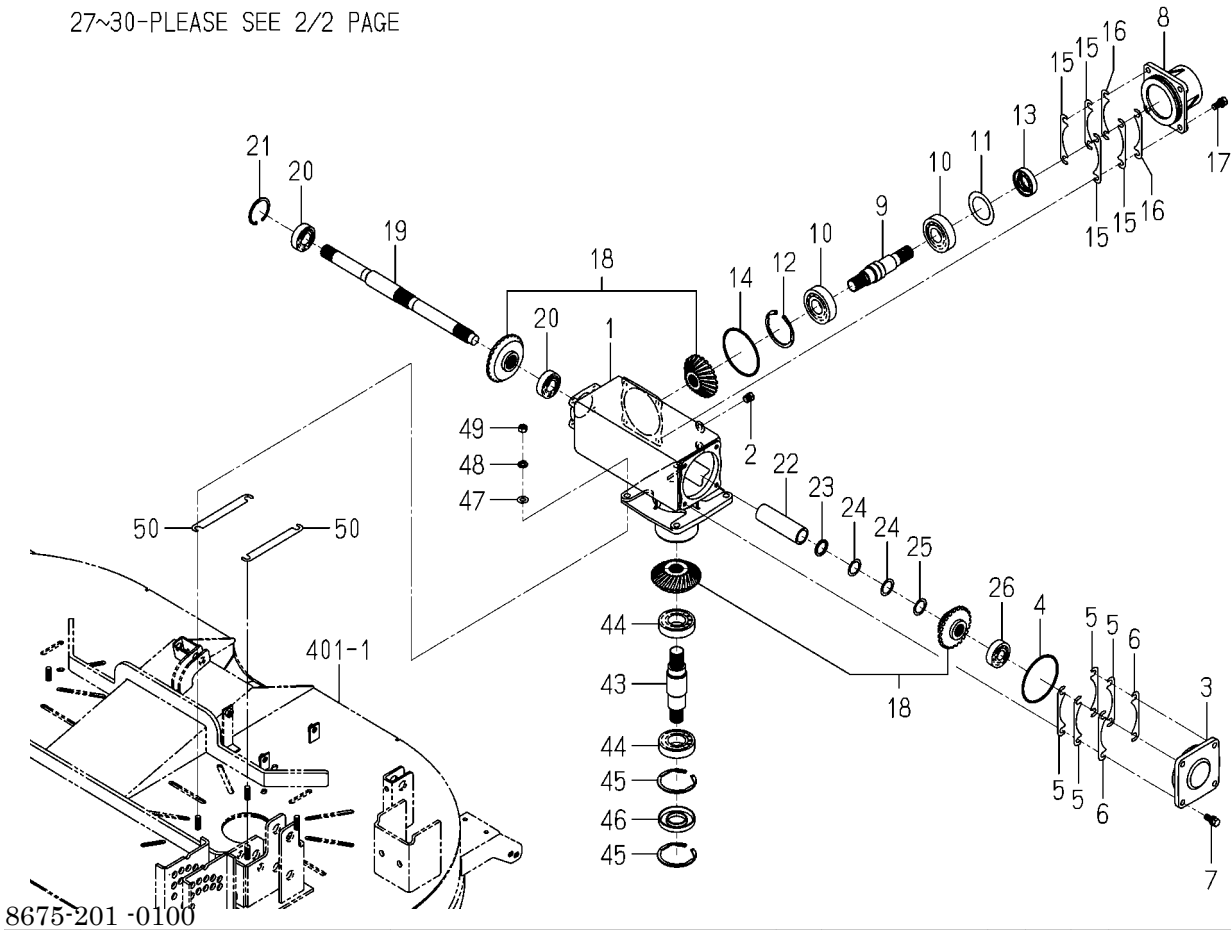
FIG.201 CASE(BEVEL)SYSTEM(1/2)
