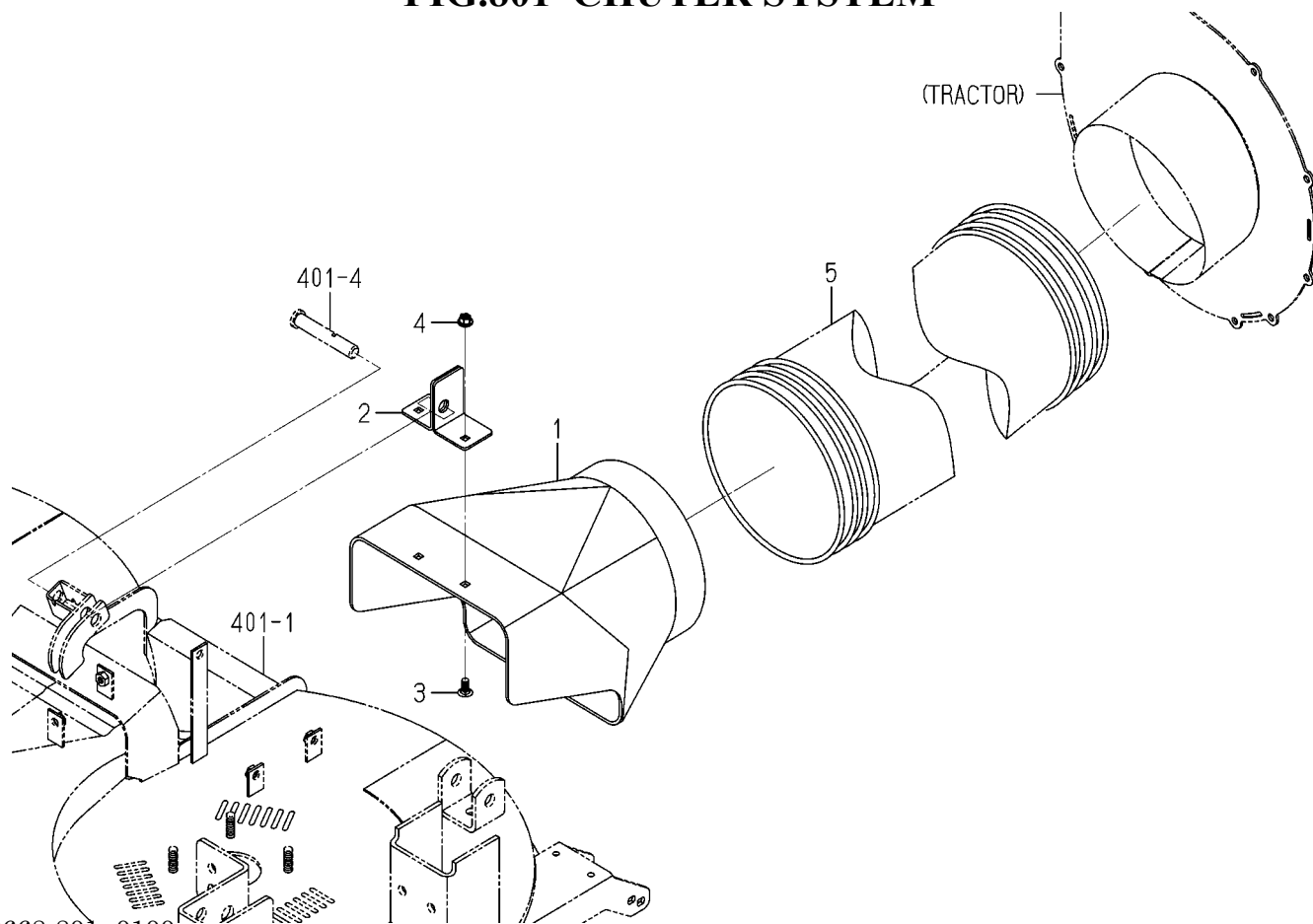
FIG.801 CHUTER SYSTEM
