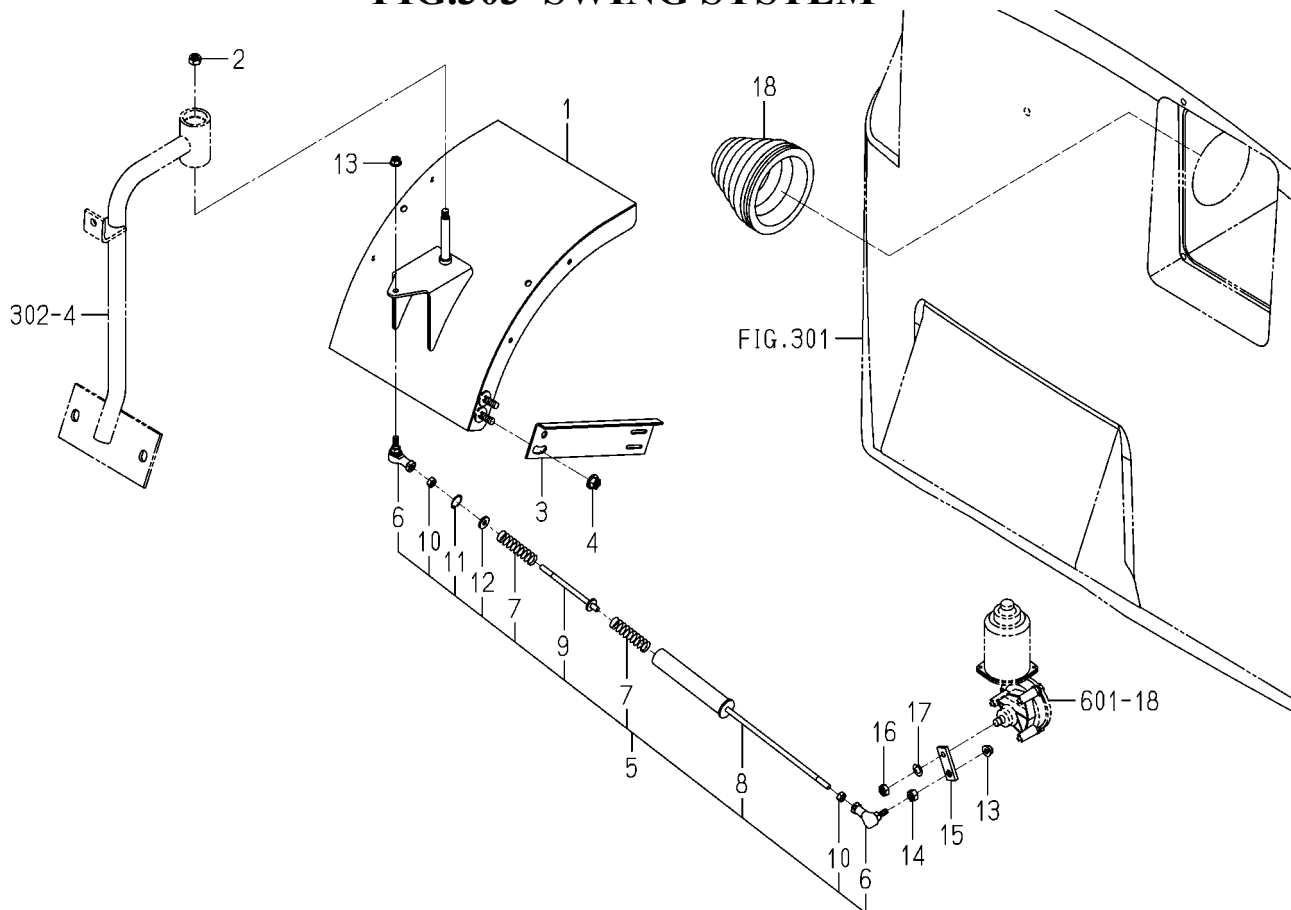
FIG.303 SWING SYSTEM
