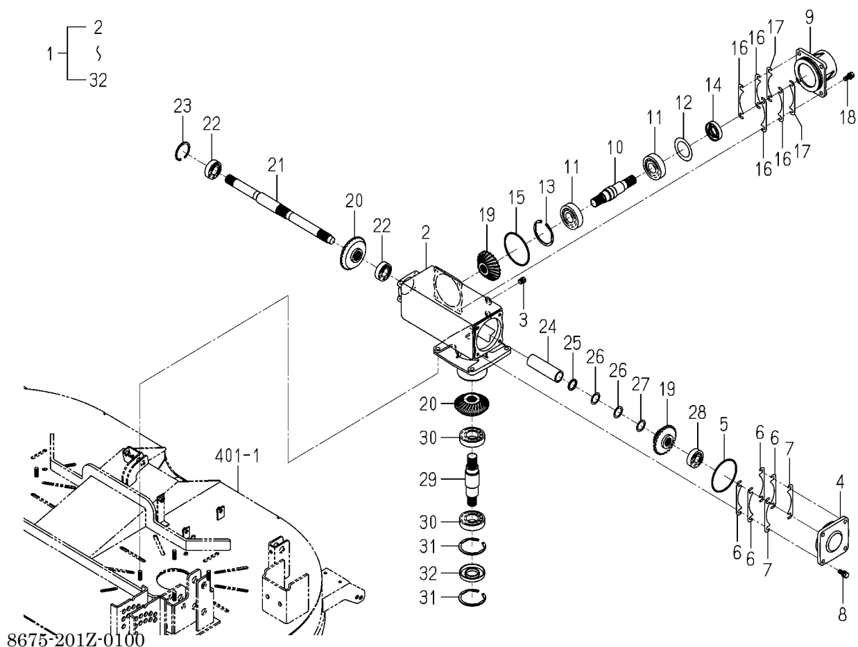
FIG.P01 CASE(BEVEL)ASSY(REPAIR)(1/2)
