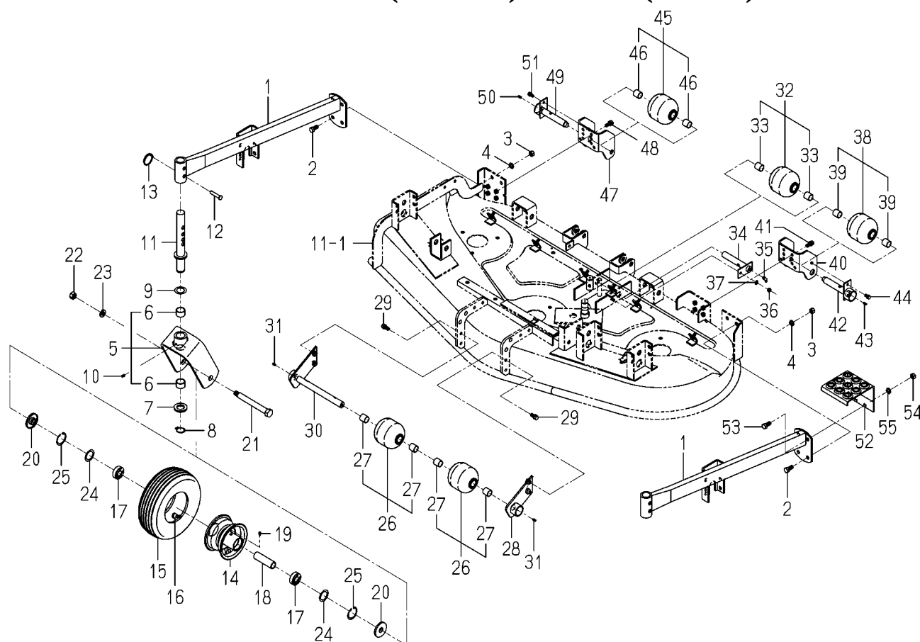
FIG. 16 WHEEL(GAUGE)SYSTEM(SSM60)
