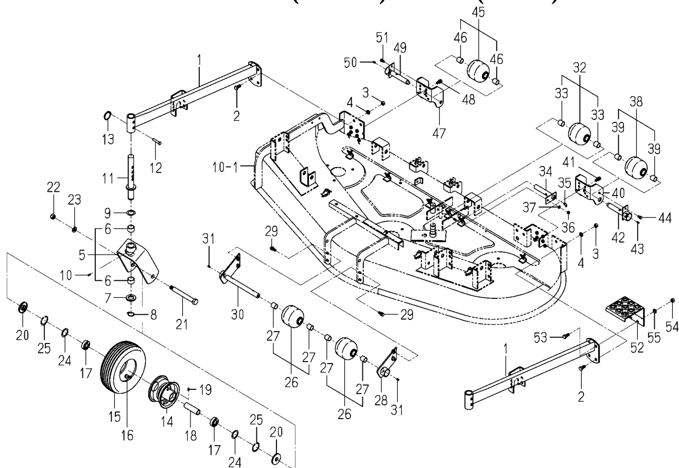
FIG. 17 WHEEL(GAUGE)SYSTEM(SSM72)
