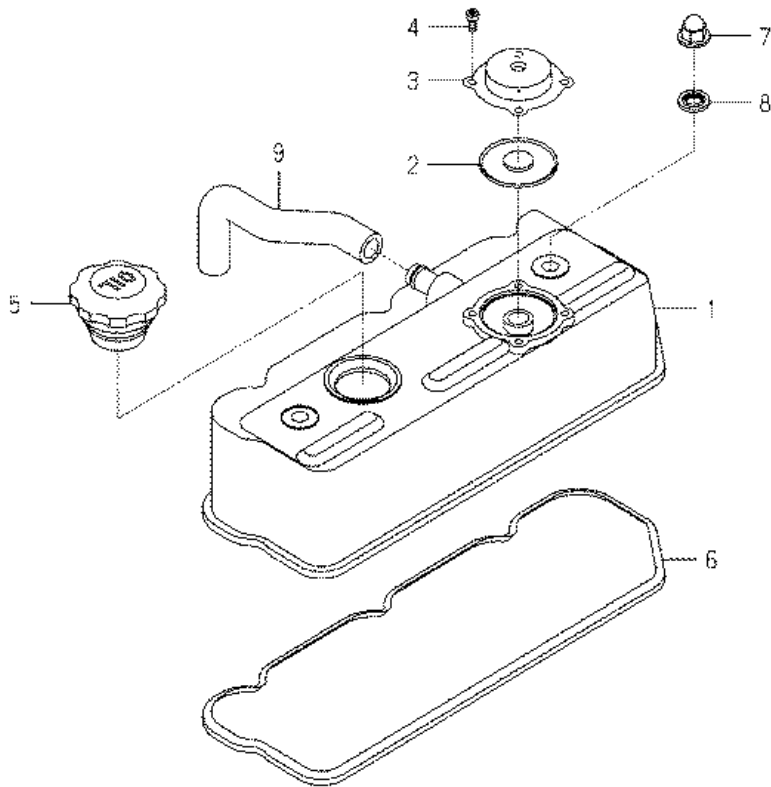
FIG. 2 CYLINDER HEAD COVER
