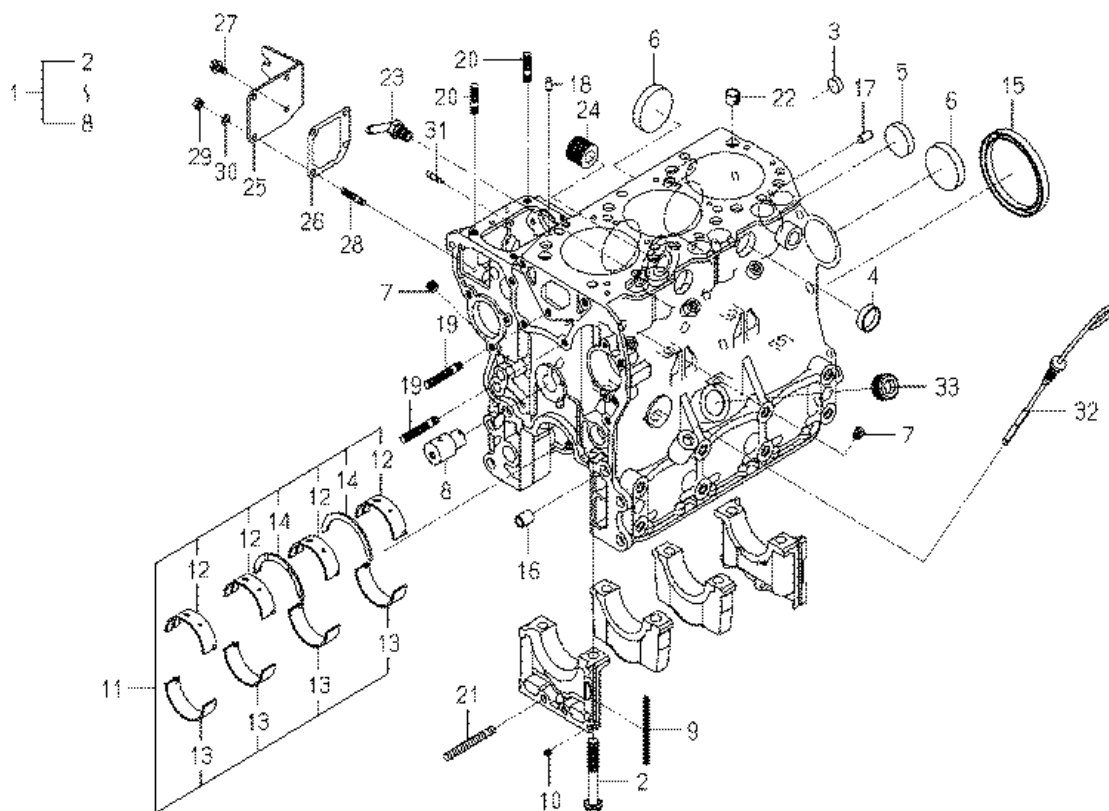
FIG. 5 CYLINDER BLOCK
