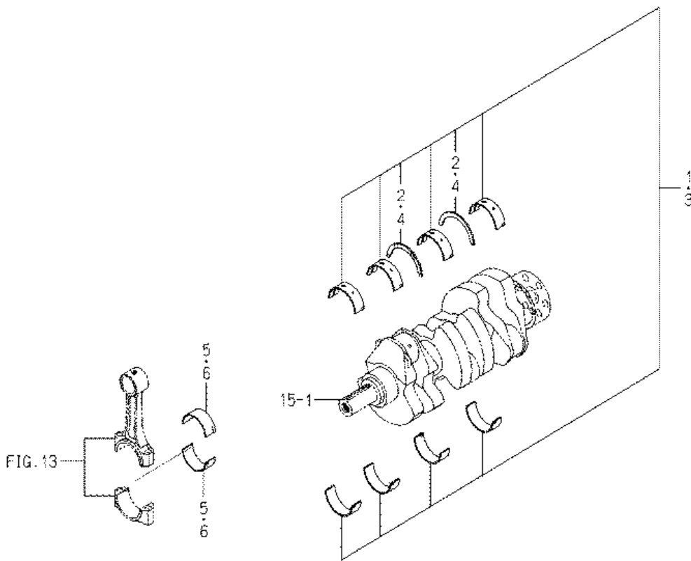
FIG. 6 BEARING/UNDER SIZE (OPTION)
