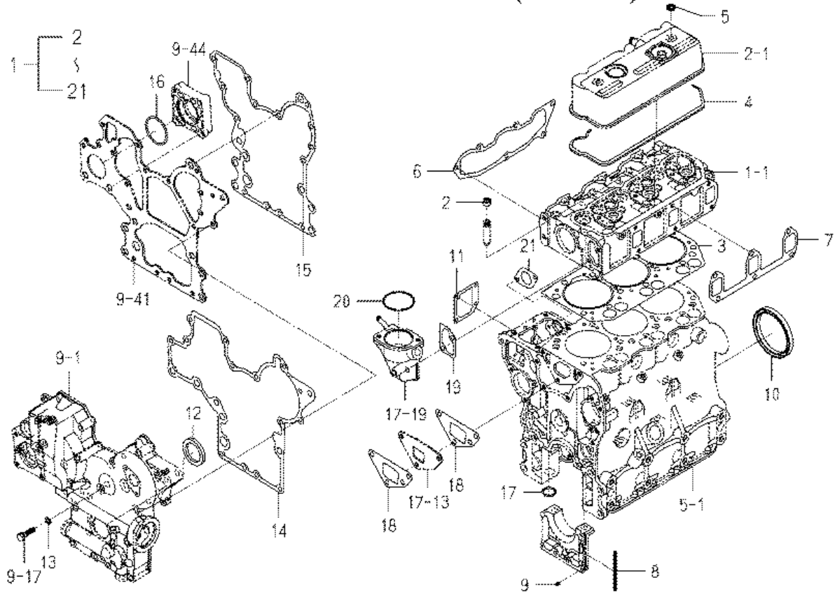
FIG. 26 REPAIR PARTS (OPTION)
