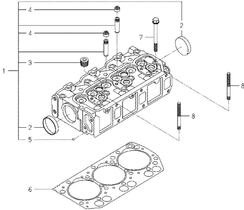
FIG. 1 CYLINDER HEAD
