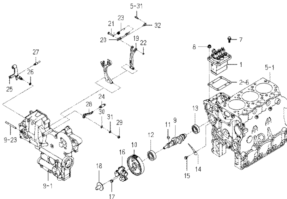
FIG. 20 INJECTION PUMP
