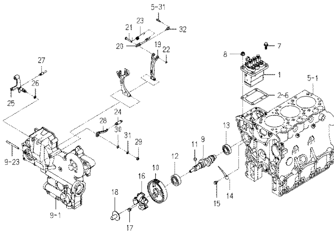
FIG. 20 INJECTION PUMP
