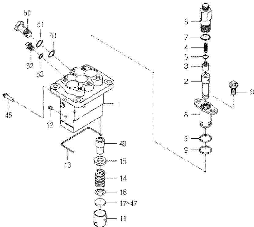
FIG. 28 COMPONENT PARTS FOR 6215-600-078-00 ON Fig.20
