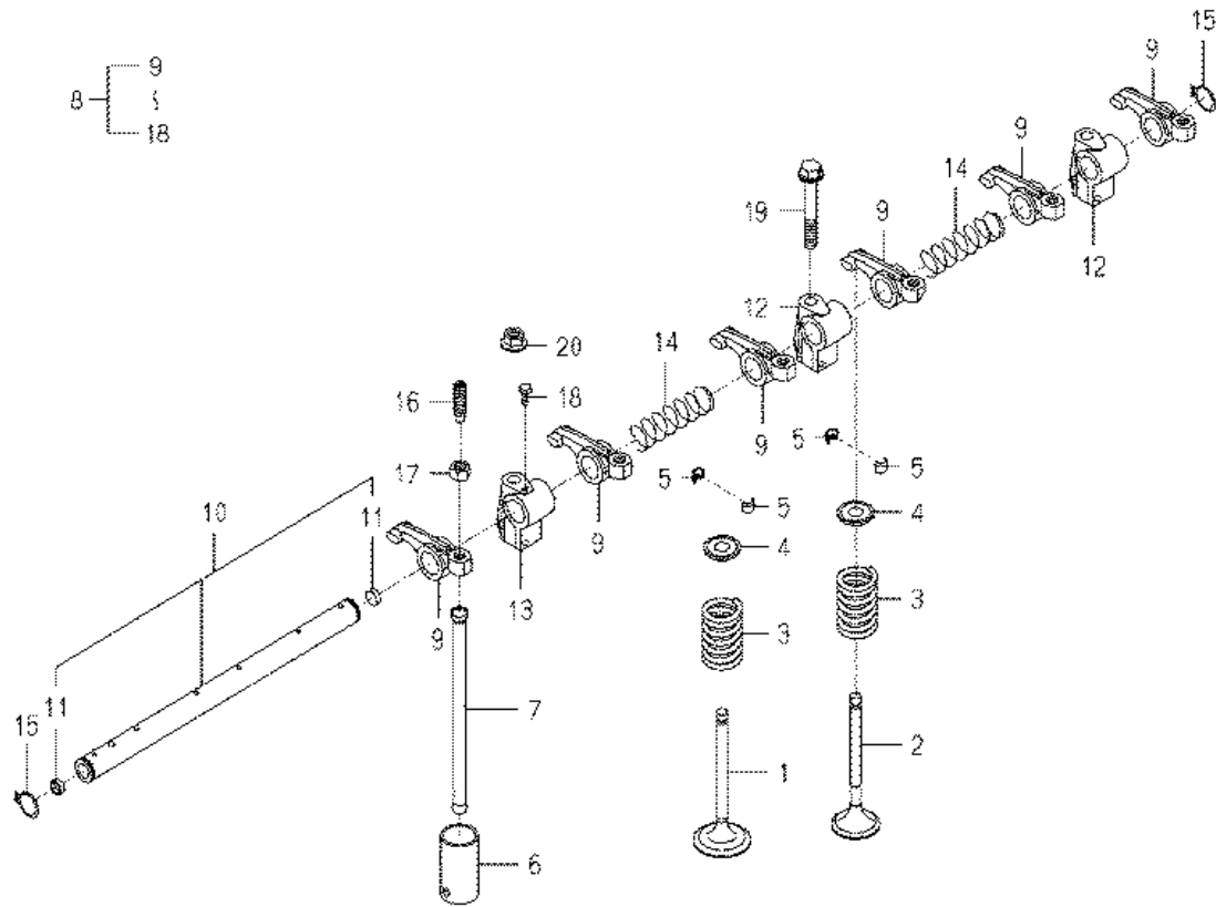
FIG. 11 VALVE
