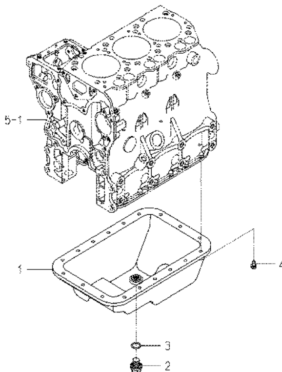
FIG. 7 OIL PAN
