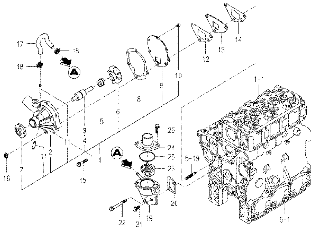
FIG. 17 WATER PUMP
