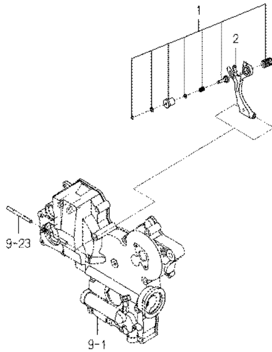
FIG. 22 ADAPTER
