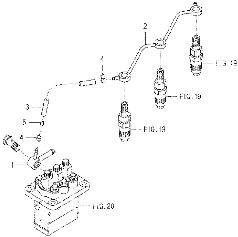
FIG. 21 FUEL PIPE
