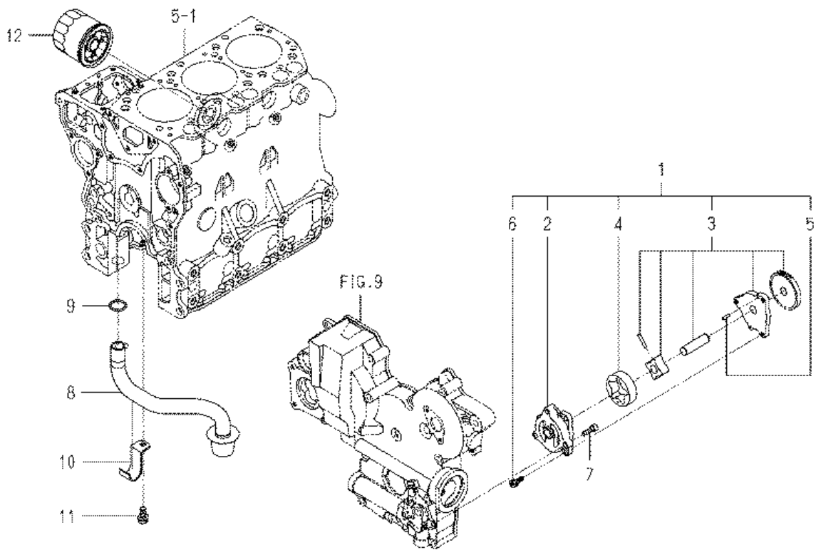
FIG. 16 OIL PUMP
