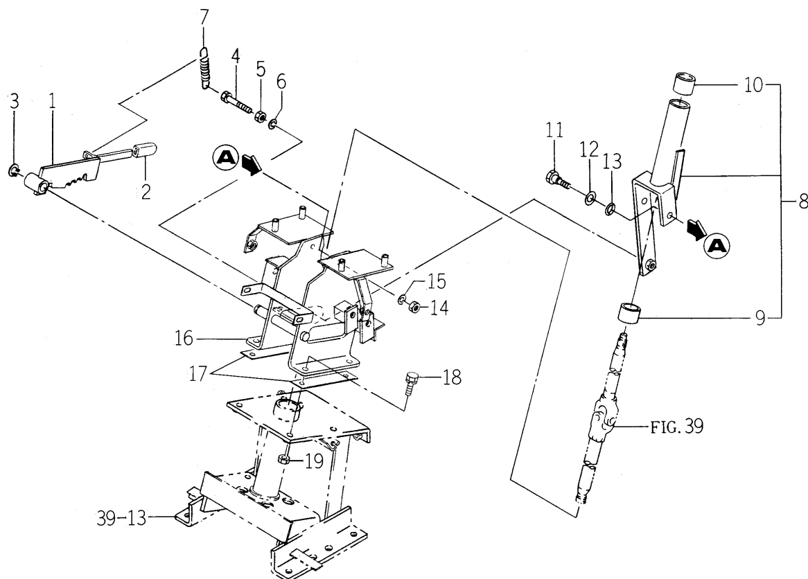
FIG. 40 LEVER (TILT) SYSTEM
