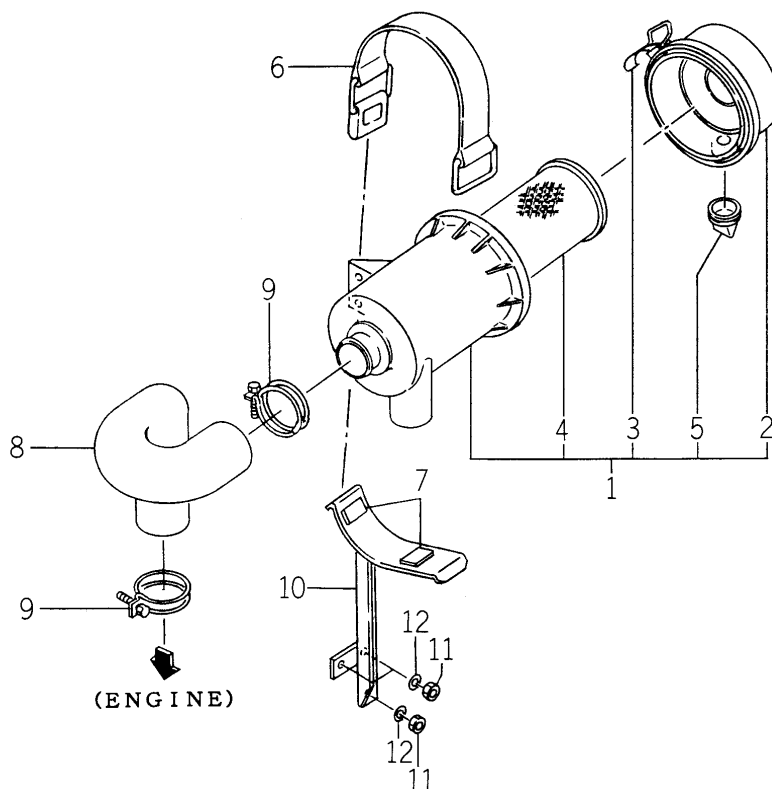
FIG. 3 CLEANER (AIR) SYSTEM
