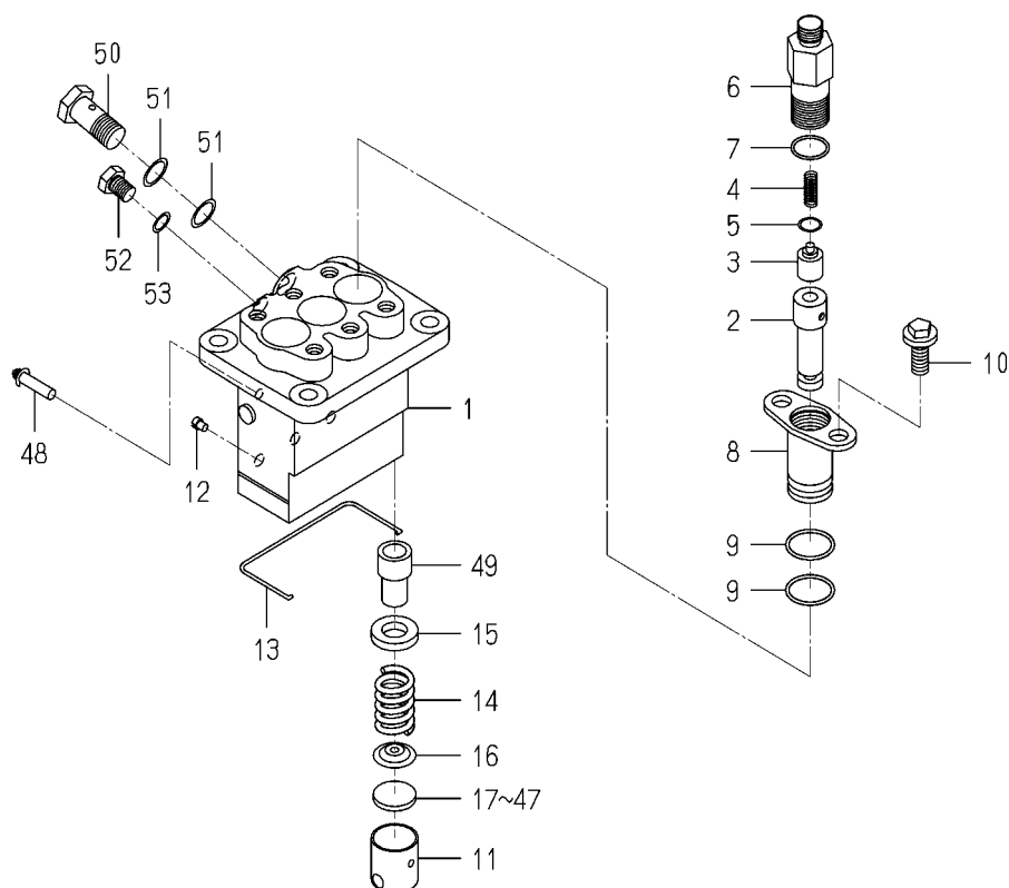
FIG. 28 COMPONENT PARTS FOR 6215-600-078-00 ON Fig.20
