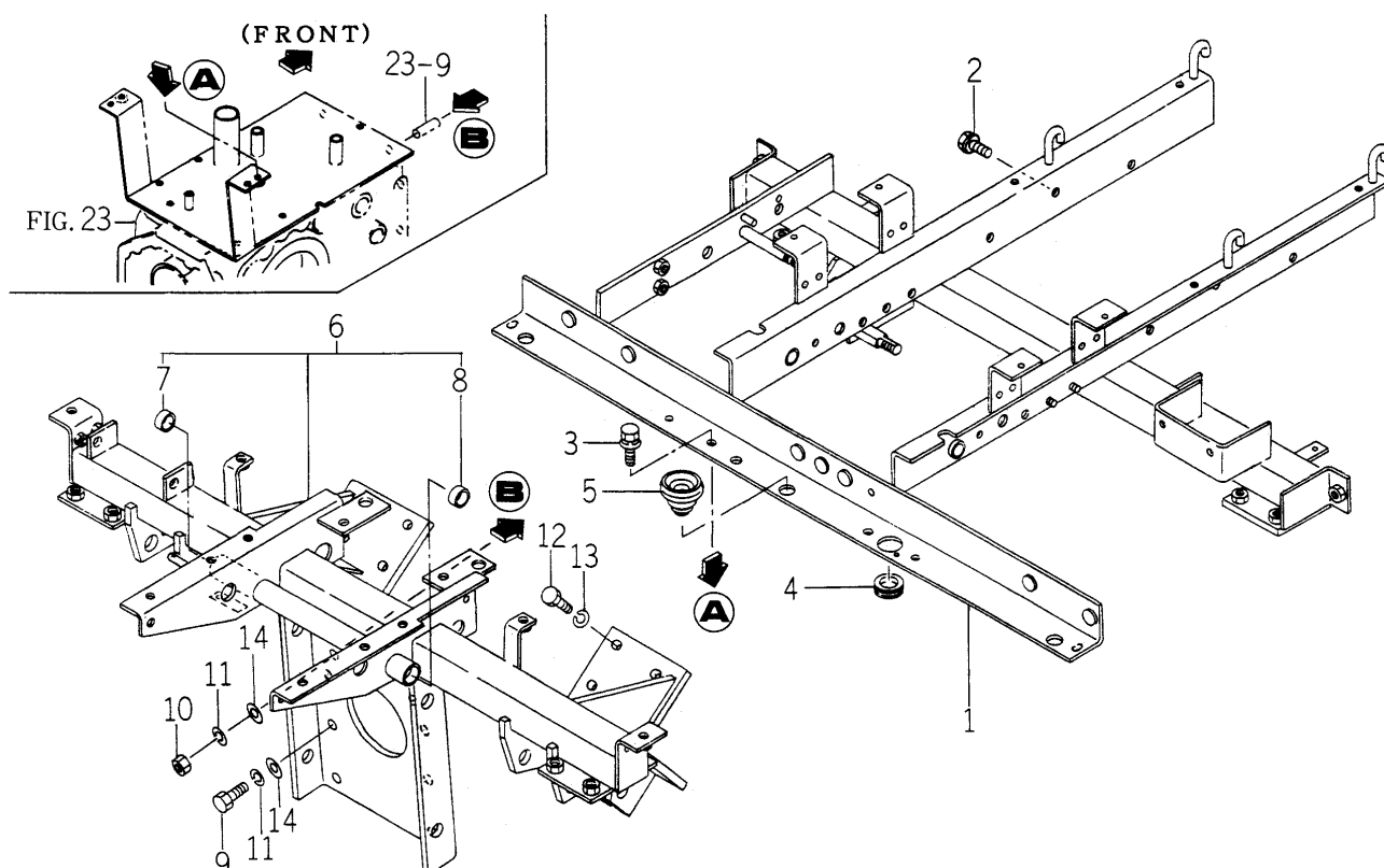
FIG. 55 SEAT FRAME,STEP FRAME SYSTEM
