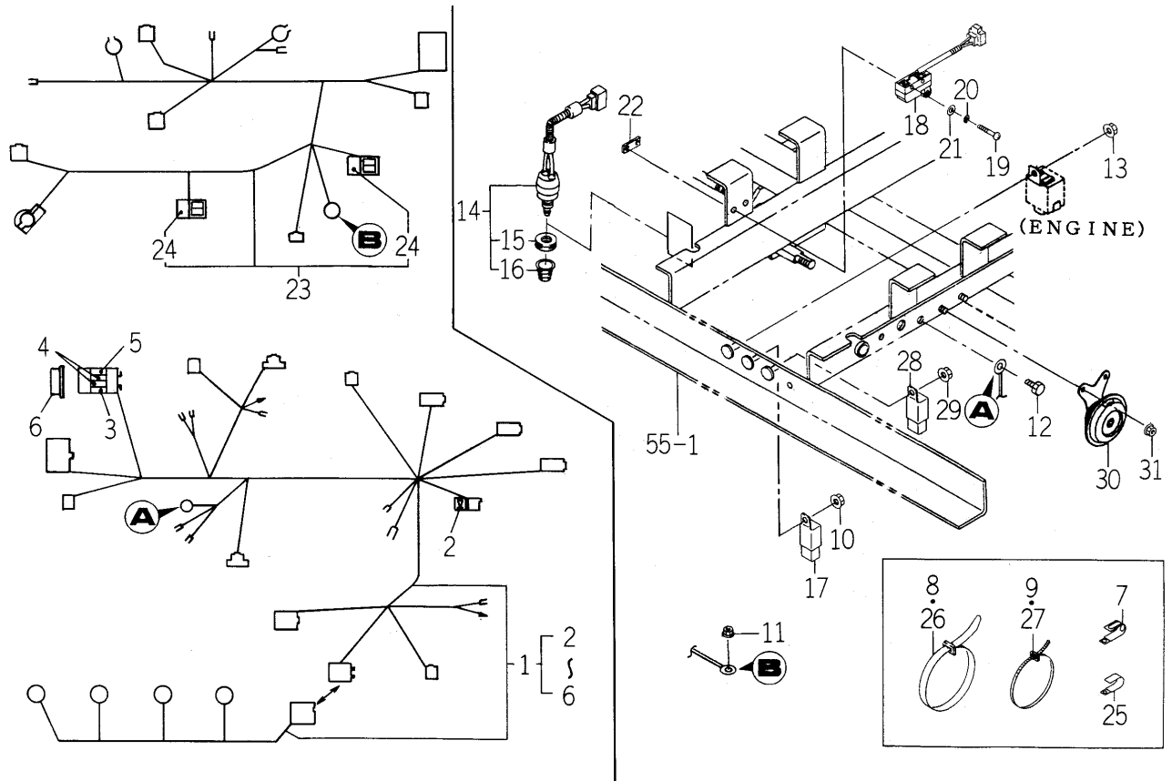
FIG. 60 HARNESS SYSTEM
