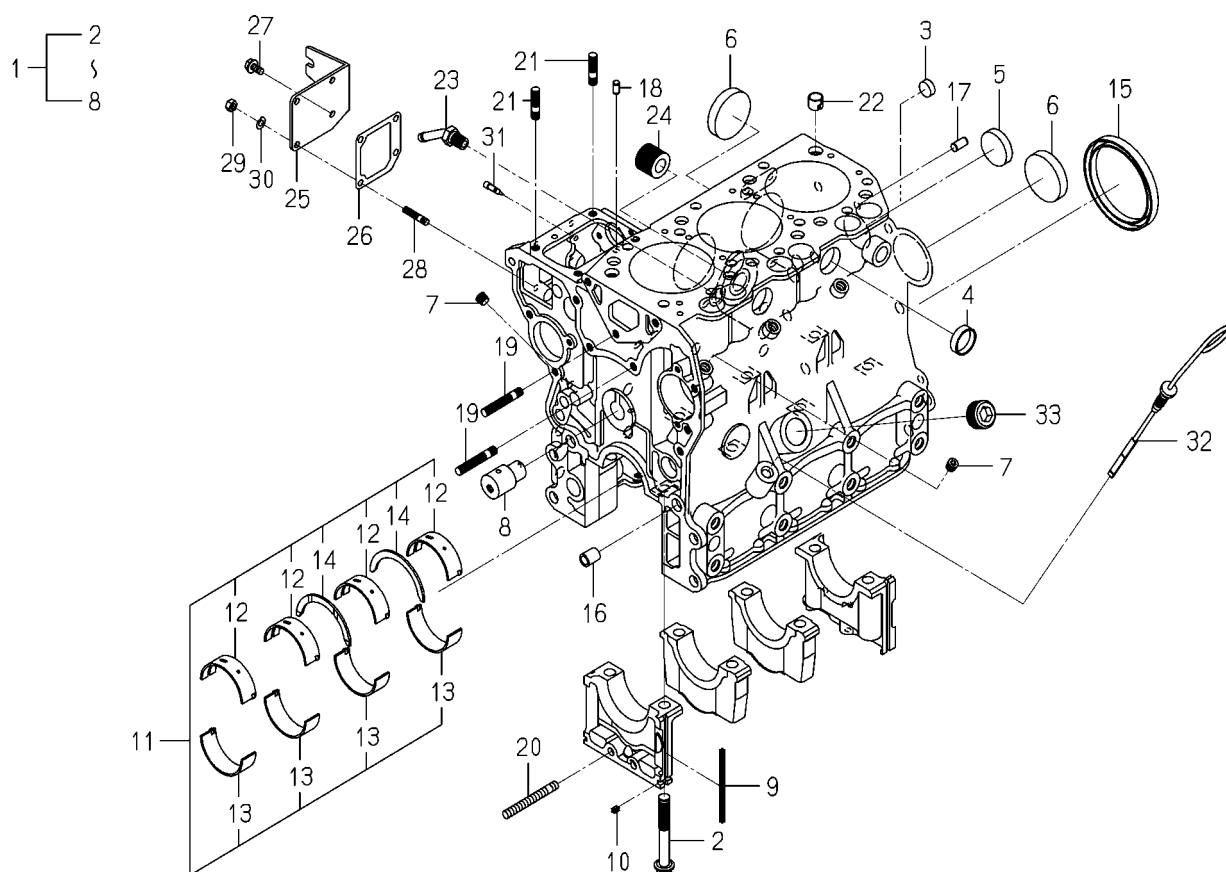
FIG. 5 CYLINDER BLOCK
