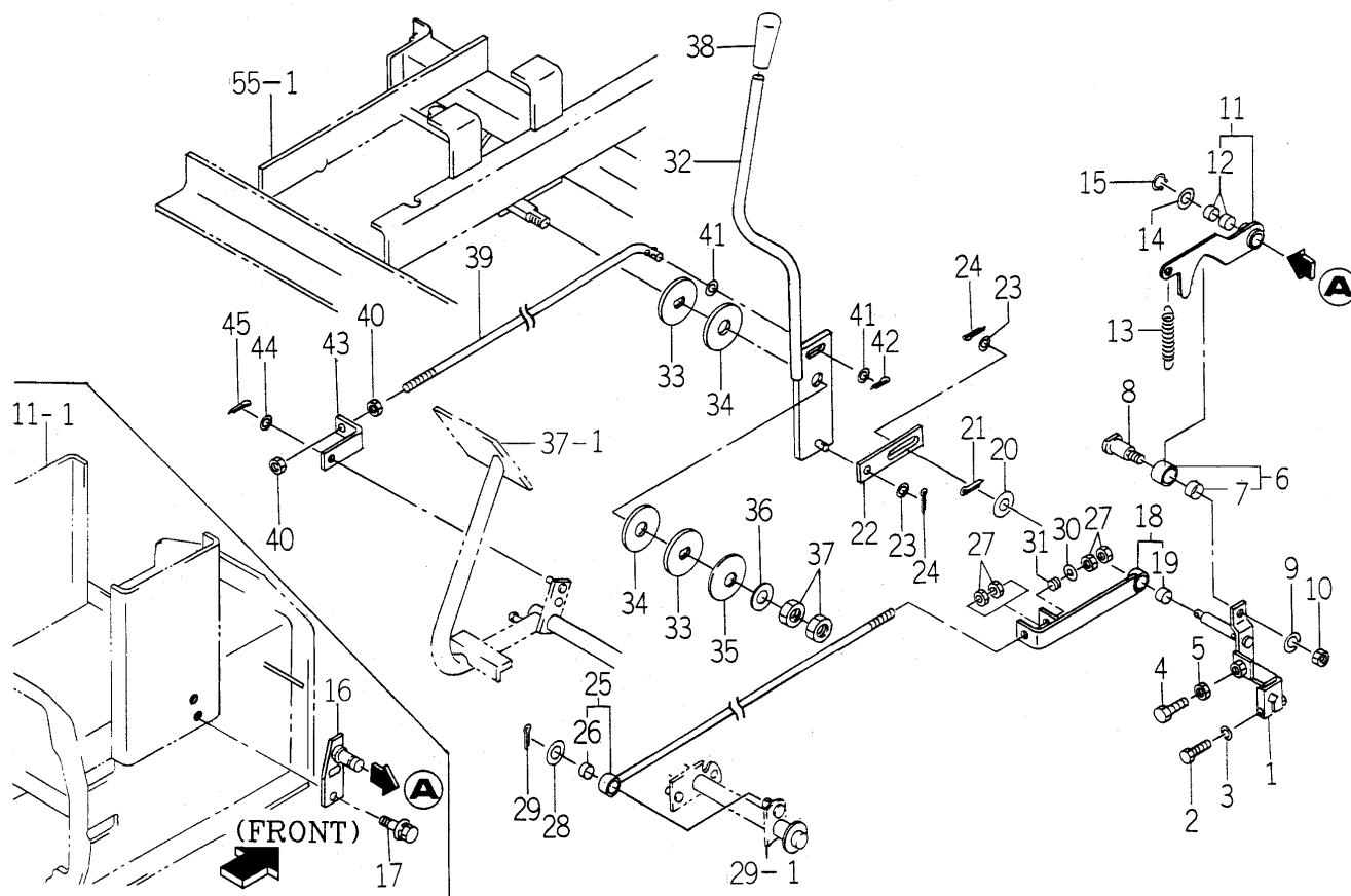
FIG. 28 LINK (HST) SYSTEM
