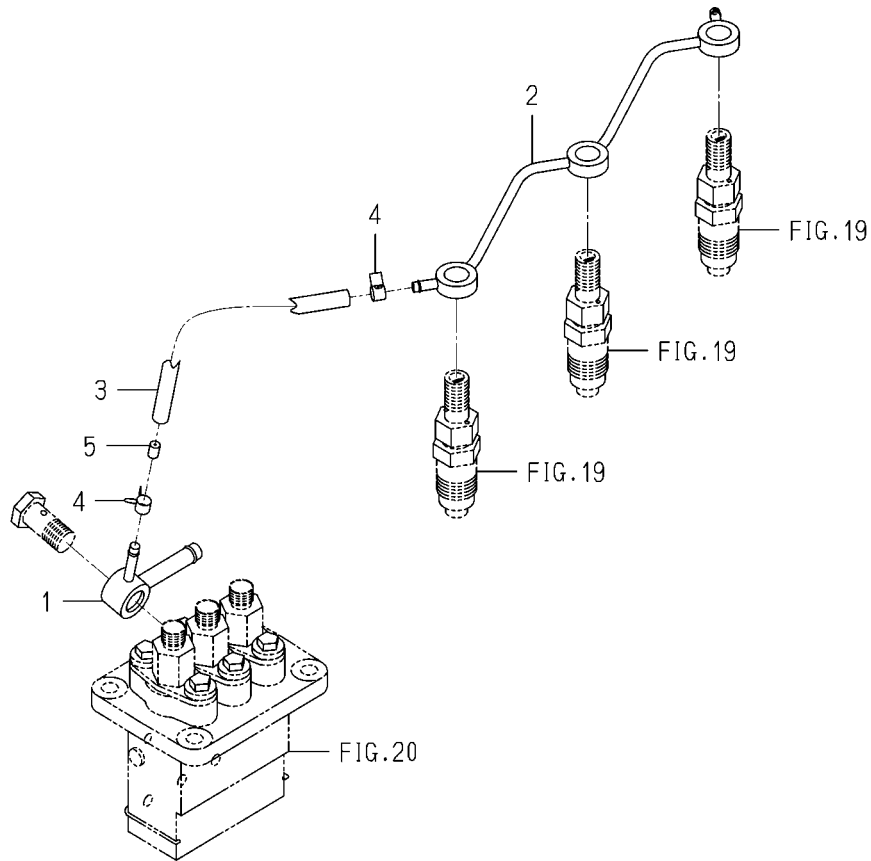
FIG. 21 FUEL PIPE
