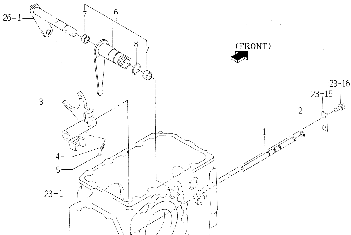
FIG. 25 PTO CHANGE SYSTEM
