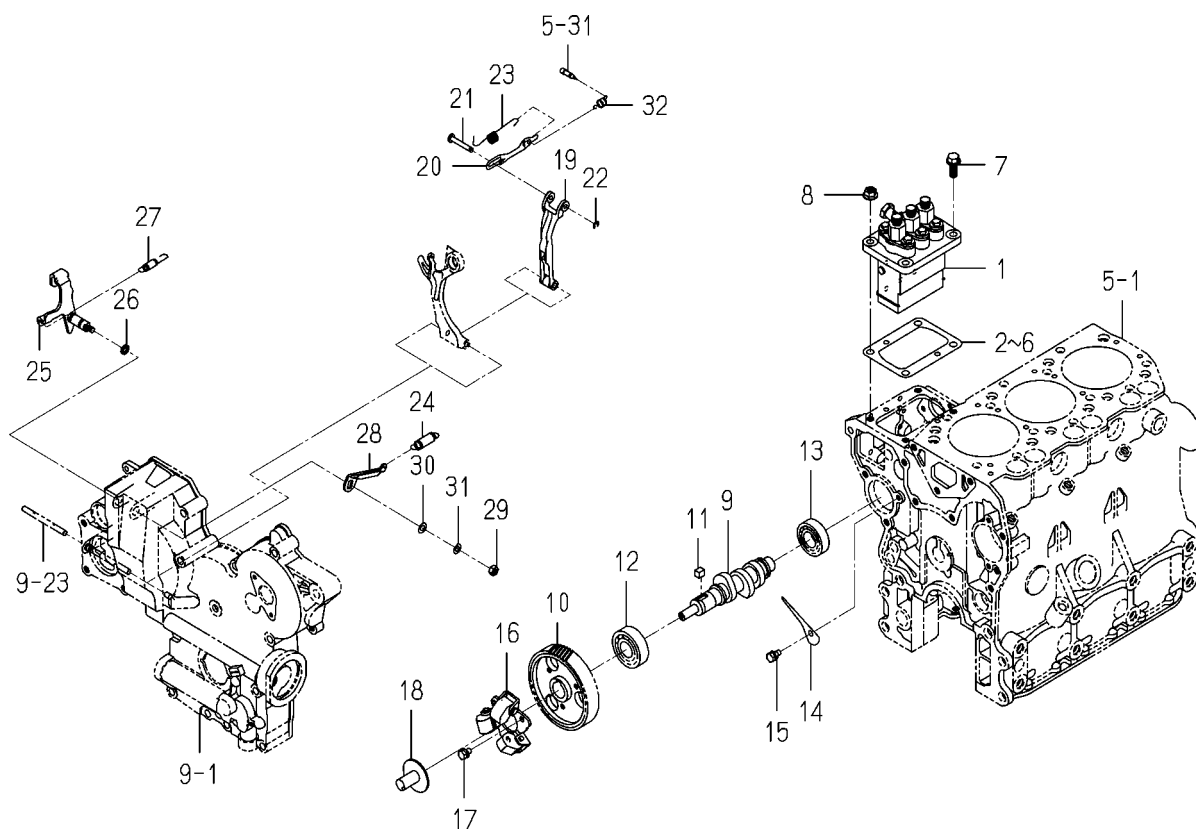
FIG. 20 INJECTION PUMP
