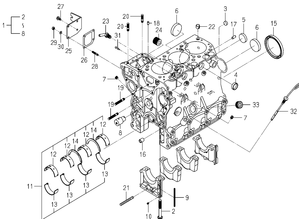
FIG. 5 CYLINDER BLOCK
