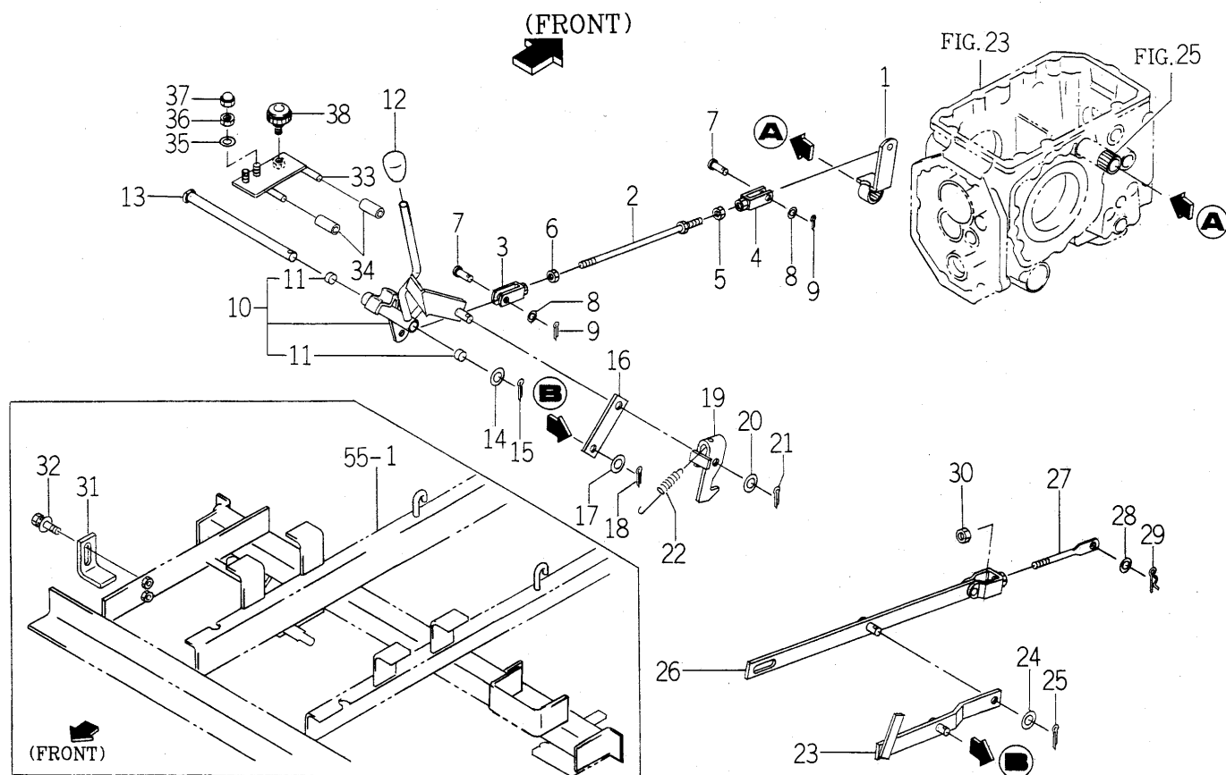
FIG. 27 CHANGE LEVER (PTO) SYSTEM
