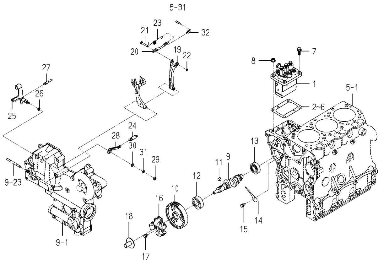
FIG. 20 INJECTION PUMP
