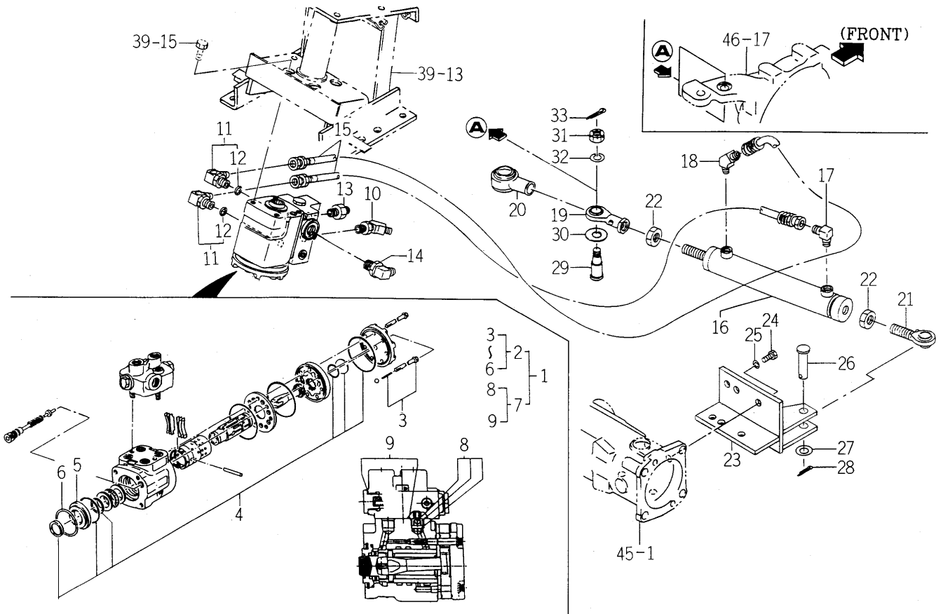
FIG. 41 STEERING (UNIT) SYSTEM
