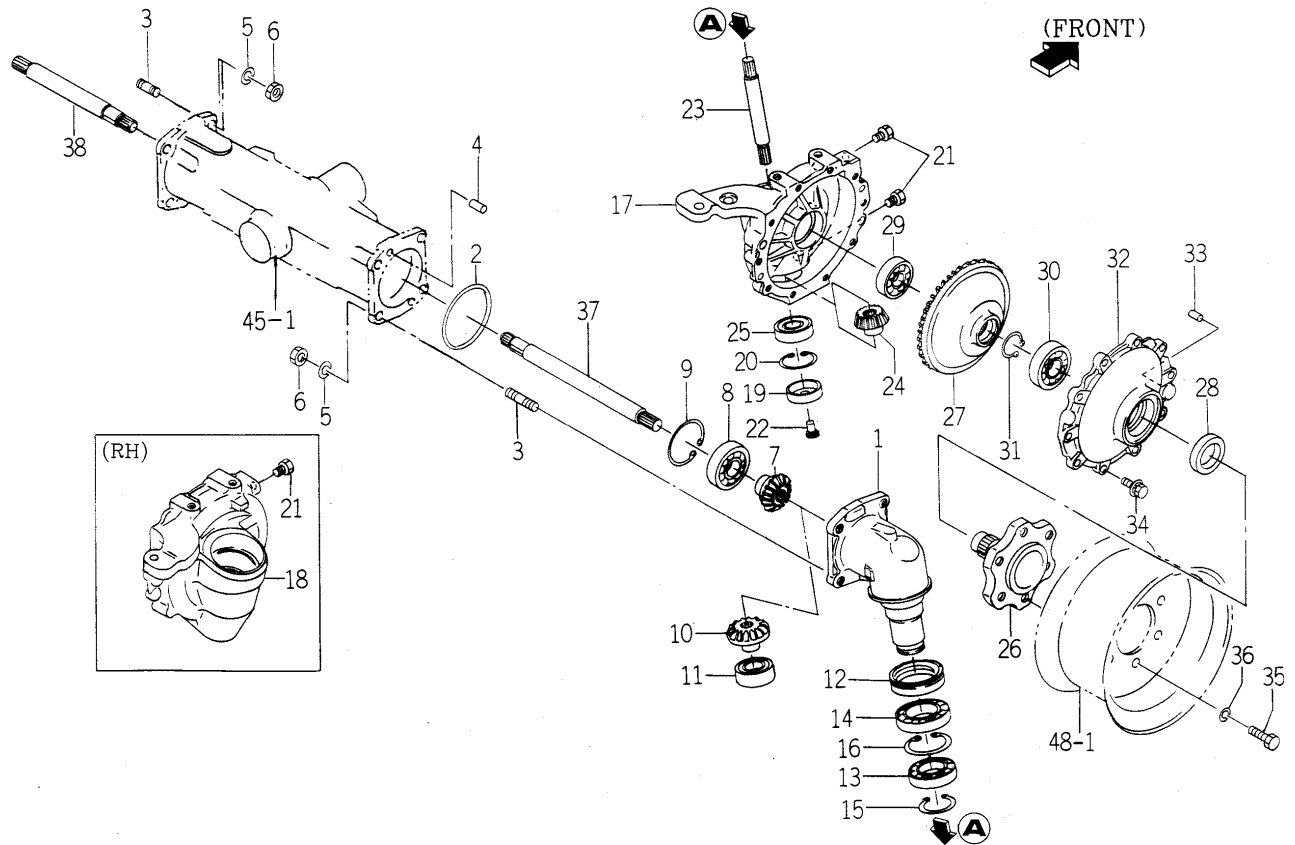
FIG. 46 FINAL GEAR CASE, FINAL DRIVE SHAFT SYSTEM
