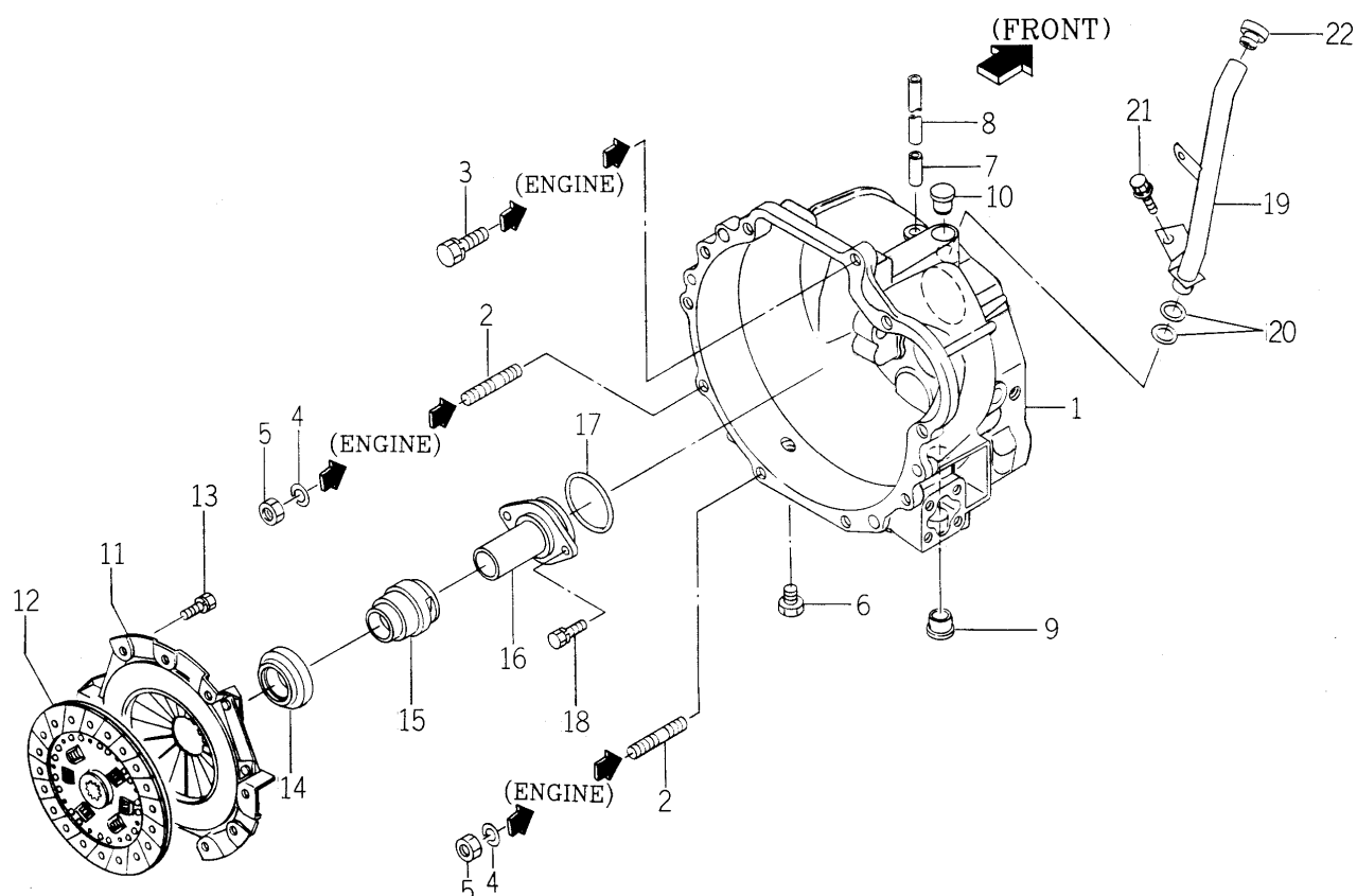
FIG. 8 MAIM CLUTCH SYSTEM
