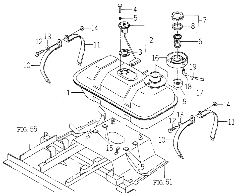
FIG. 5 TANK (FUEL) SYSTEM
