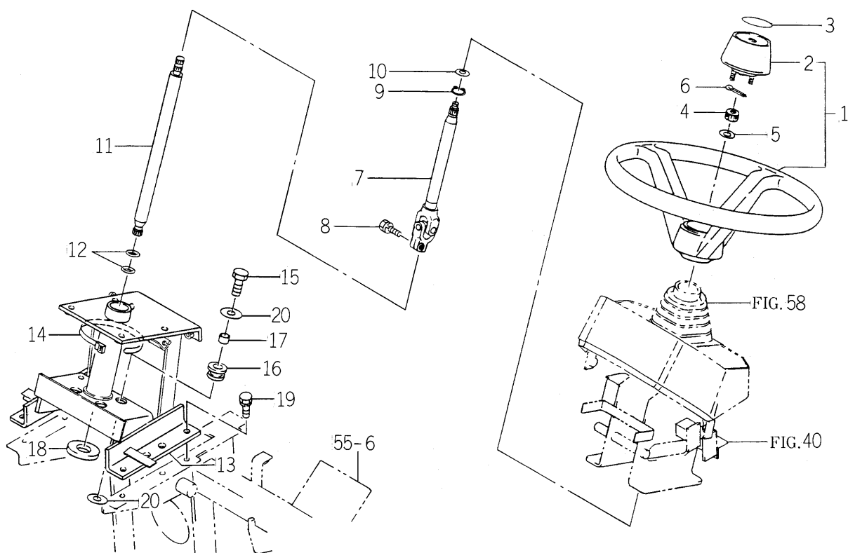
FIG. 39 WHEEL (STEERING), SHAFT (STEERING) SYSTEM
