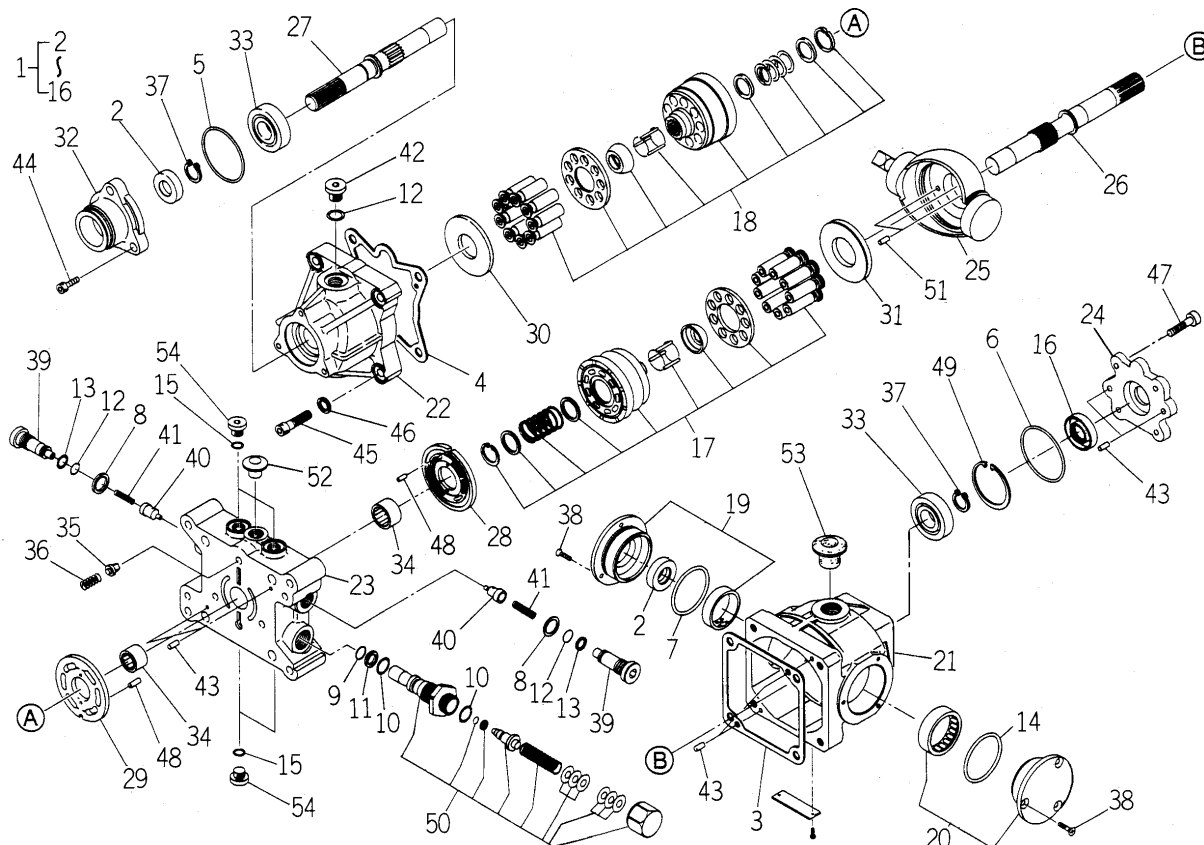
FIG. 72 COMPONENT PARTS FOR 1720-202-200-20 ON Fig.15
