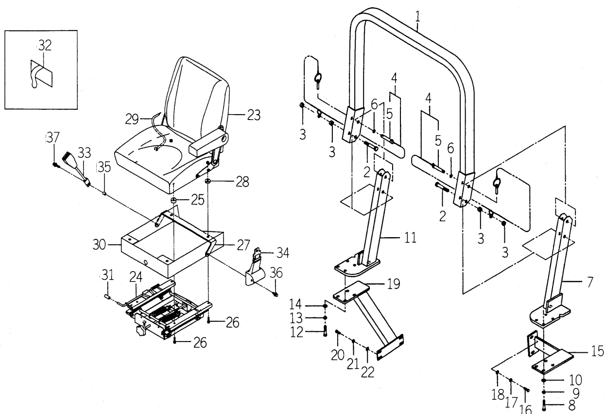
FIG. 67 ROPS,SEAT SYSTEM (OPTION)
