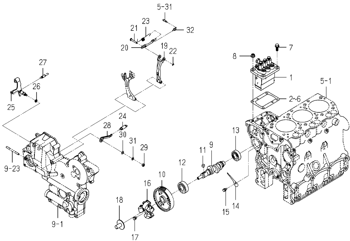
FIG. 20 INJECTION PUMP
