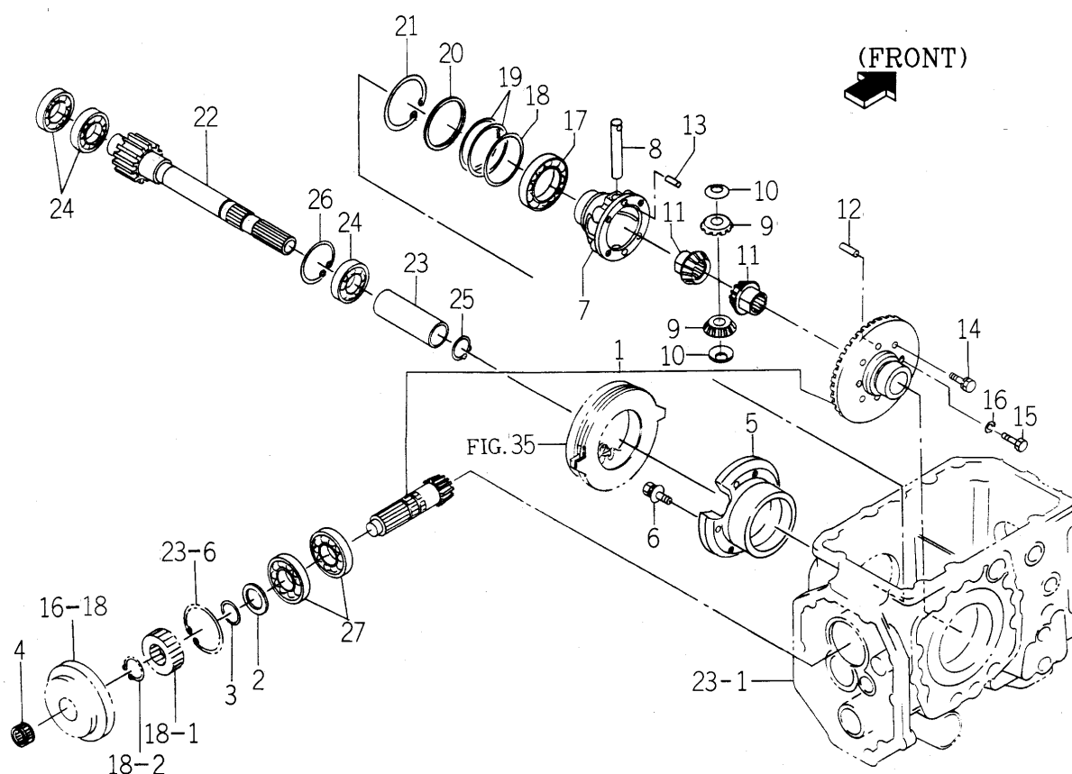
FIG. 31 DRIVE PINION (HST),CASE (DIFF) SYSTEM
