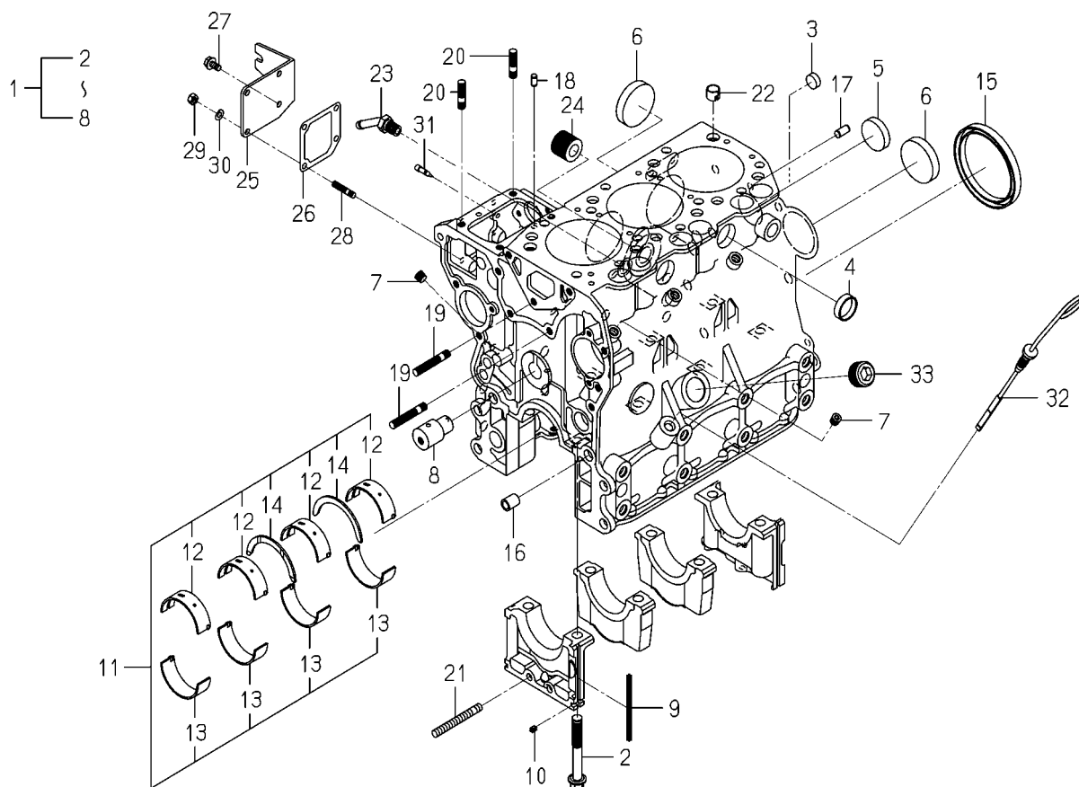
FIG. 5 CYLINDER BLOCK
