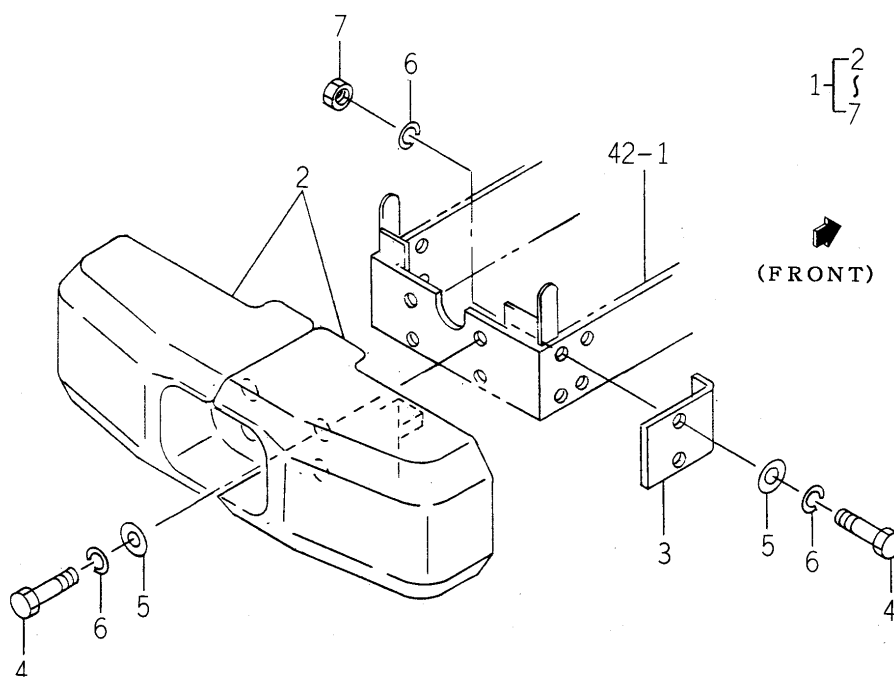
FIG. 65 REAR WEIGHT SET (EXCEPT W TYPE) (OPTION)
