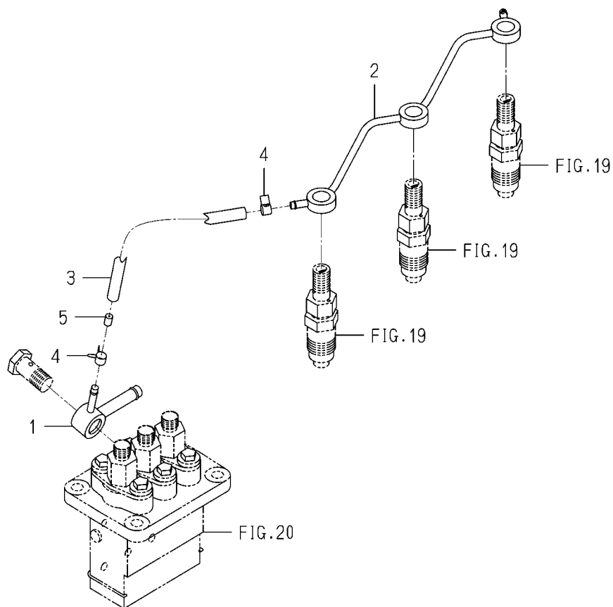
FIG. 21 FUEL PIPE
