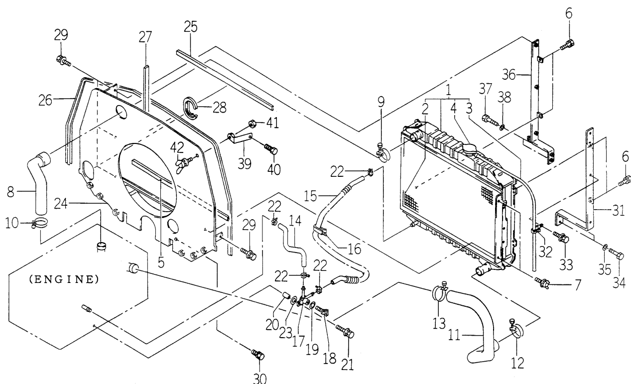
FIG. 1 RADIATOR SYSTEM
