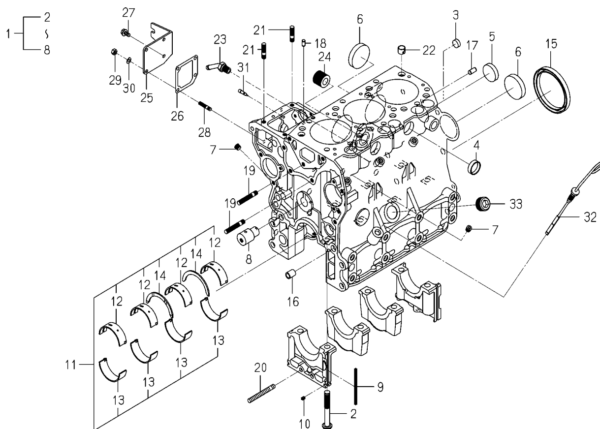
FIG. 5 CYLINDER BLOCK
