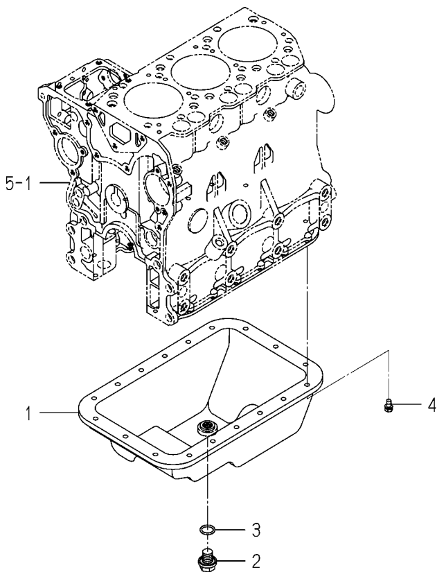
FIG. 7 OIL PAN
