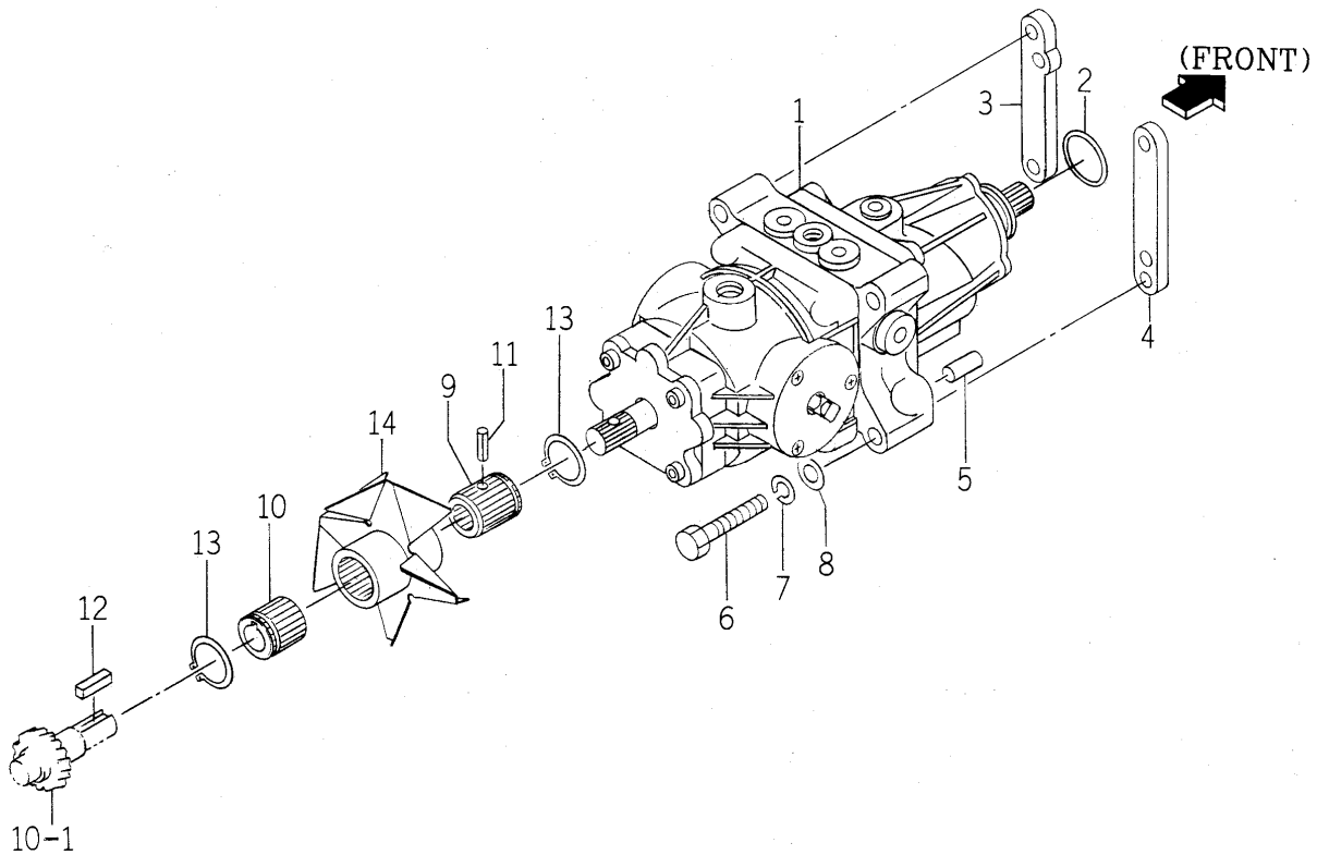
FIG. 15 HST SYSTEM
