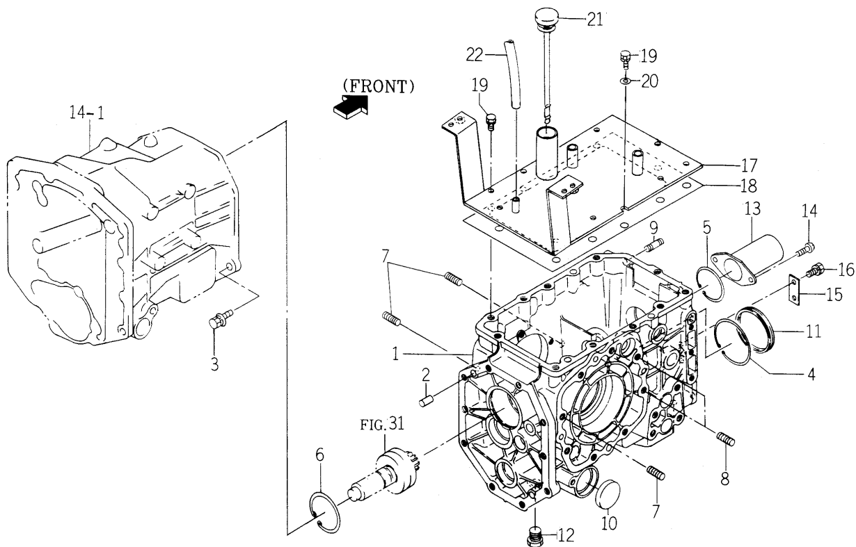
FIG. 23 REAR TRANSMISSION CASE SYSTEM
