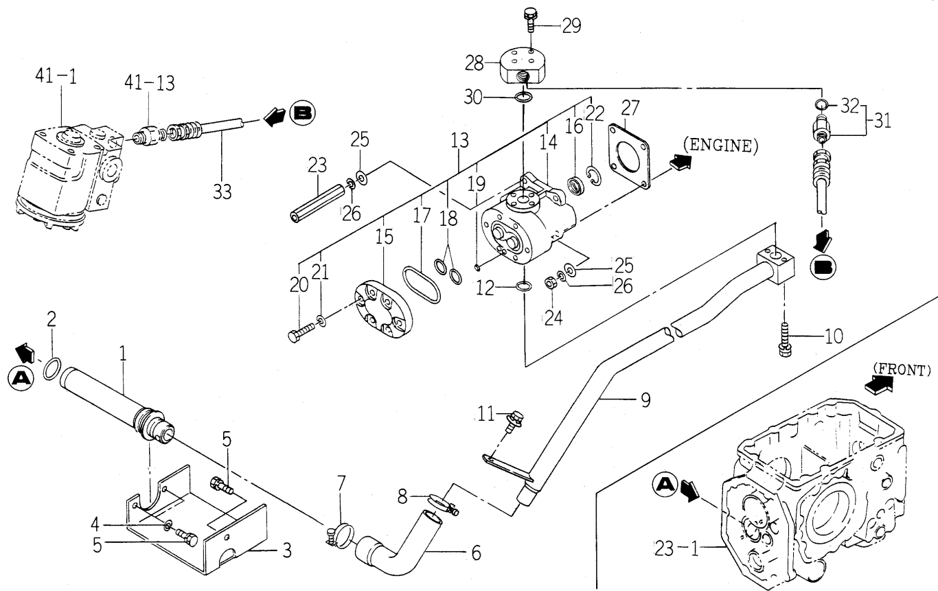
FIG. 52 PIPING (MAIN) SYSTEM
