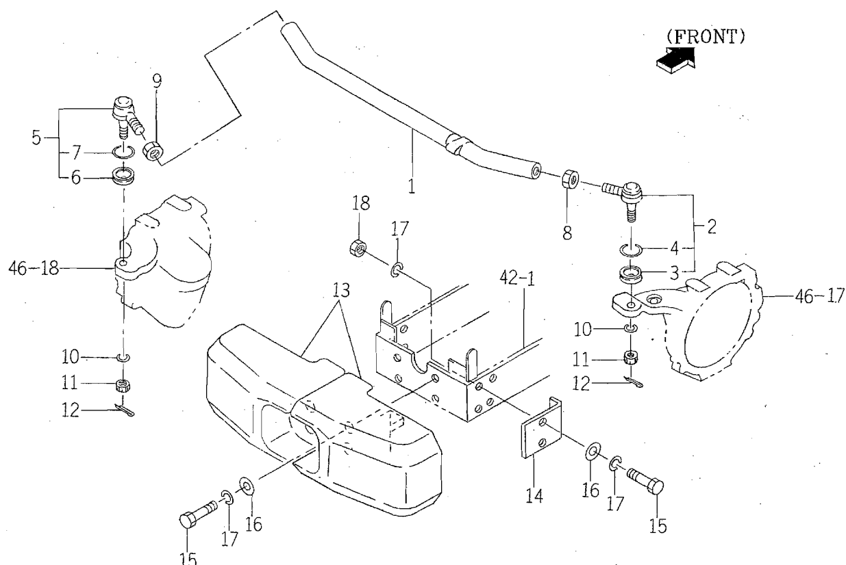
FIG. 47 TIE ROD SYSTEM
