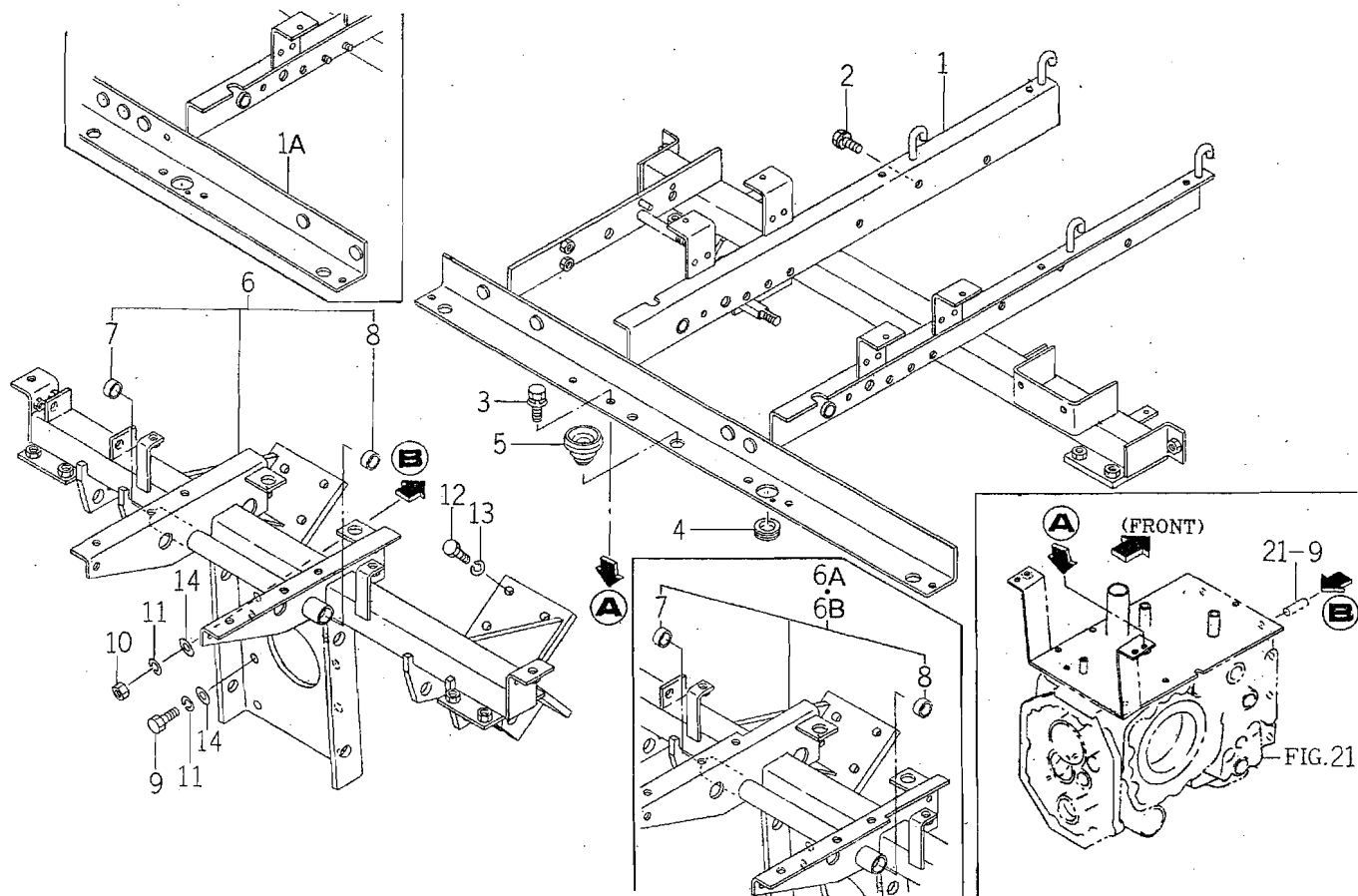
FIG. 54 SEAT FRAME,STEP FRAME SYSTEM
