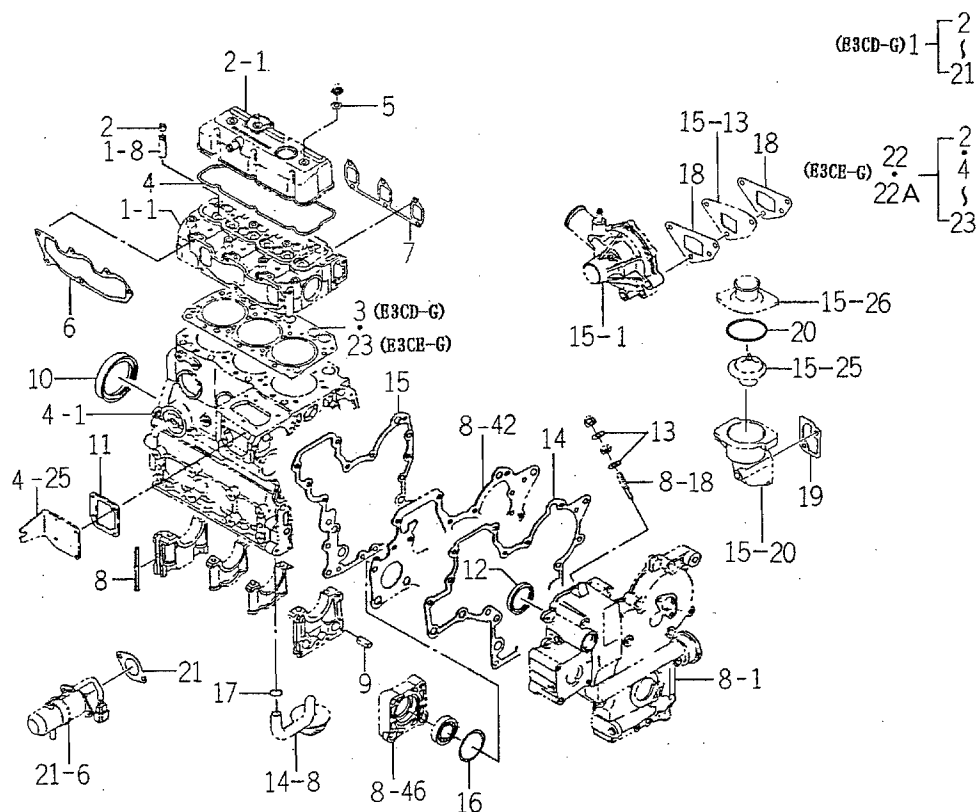
FIG. 22 REPAIR PARTS
