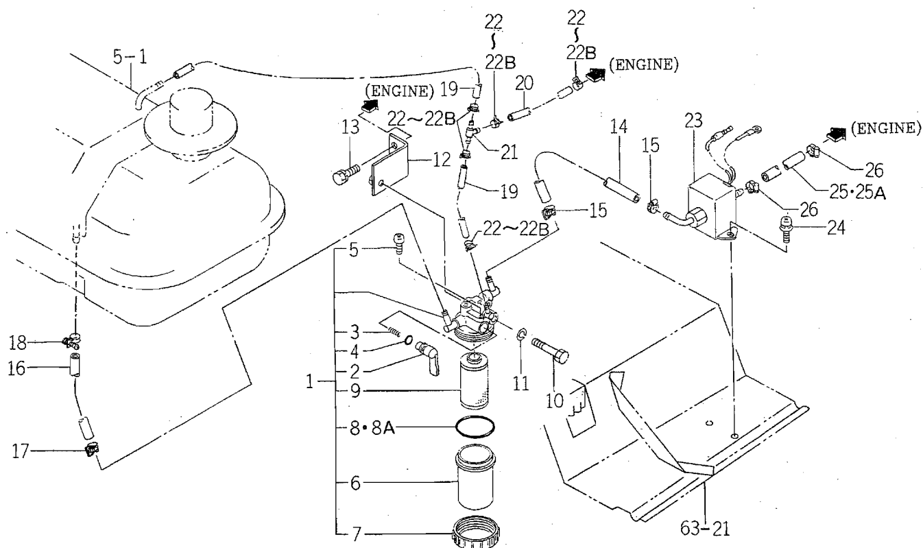
FIG. 4 FILTER SYSTEM
