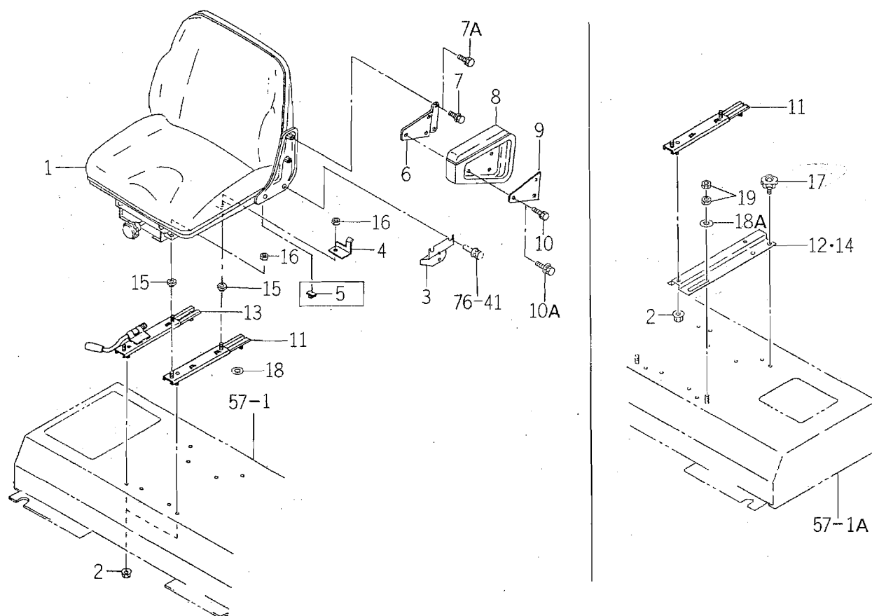
FIG. 59 SEAT SYSTEM
