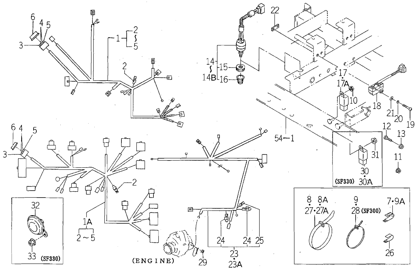
FIG. 62 HARNESS SYSTEM
