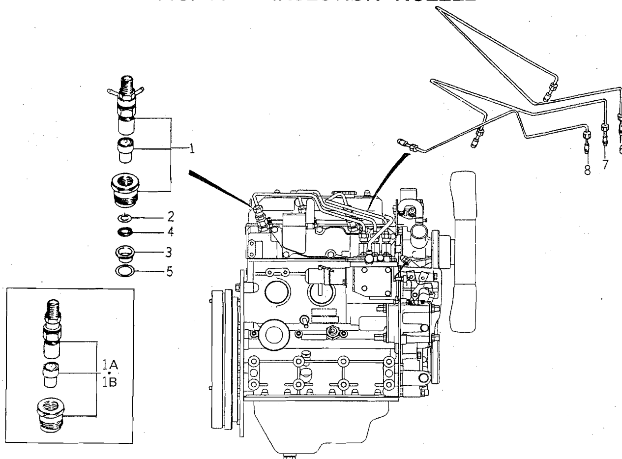
FIG. 17 INJECTION NOZZLE
