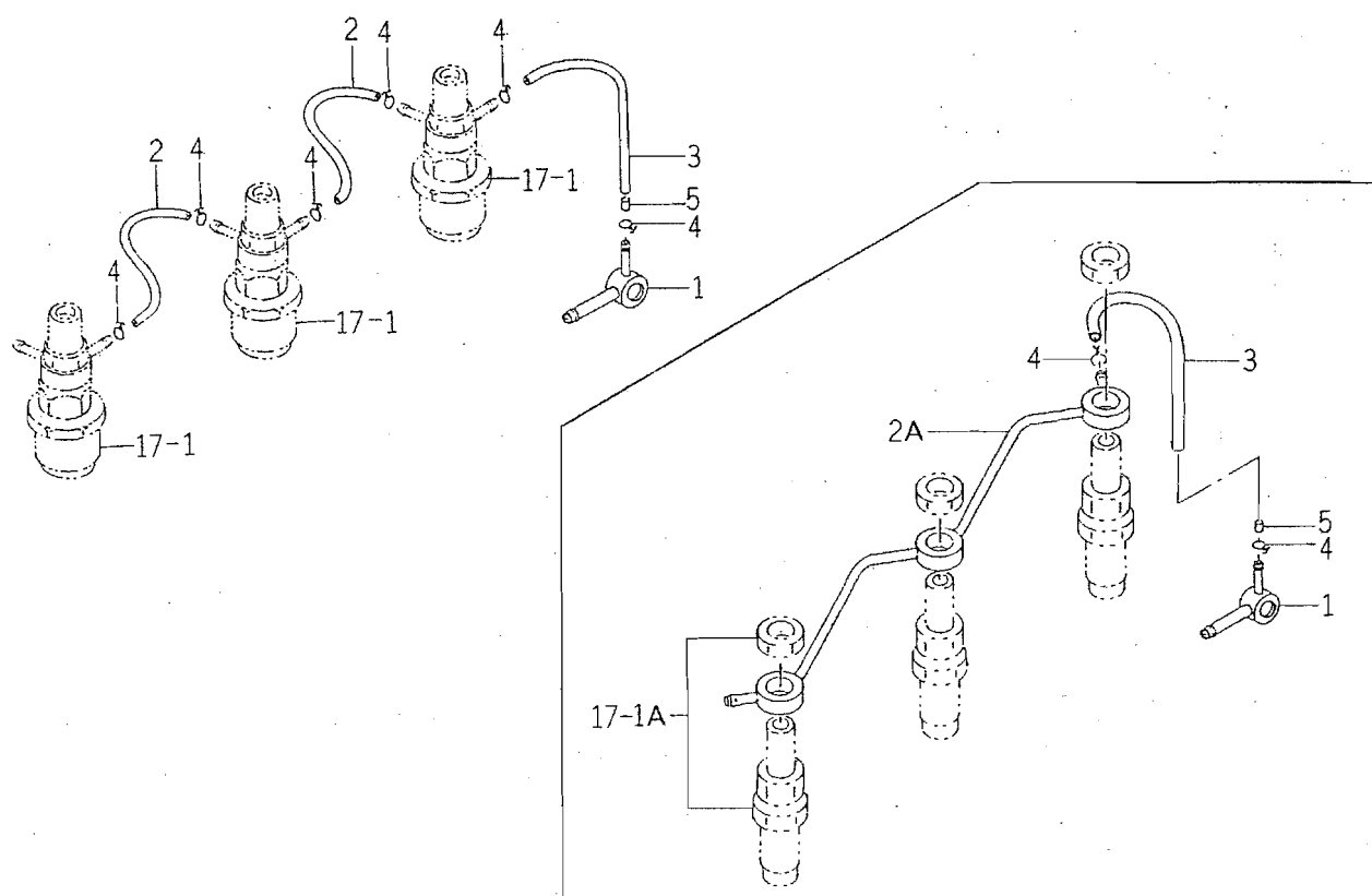
FIG. 19 FUEL PIPE
