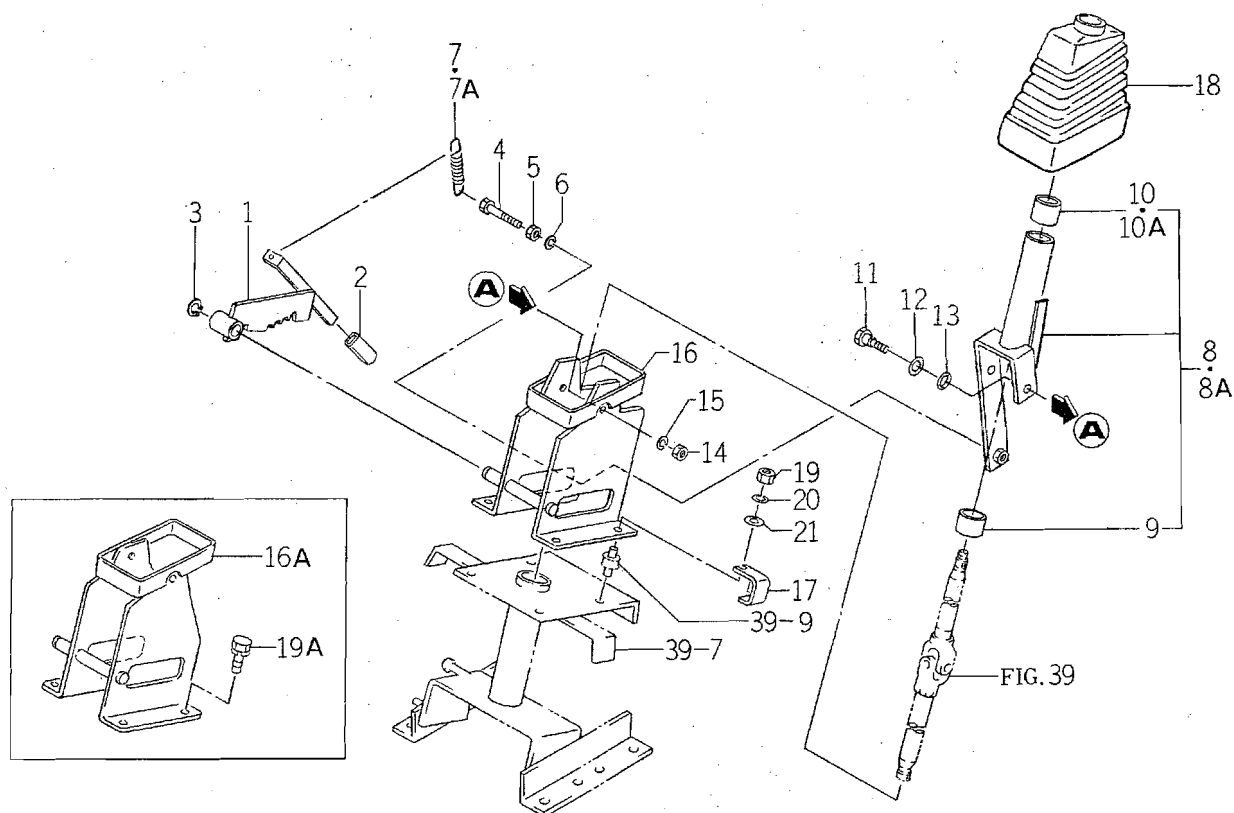
FIG. 40 LEVER (TILT) SYSTEM
