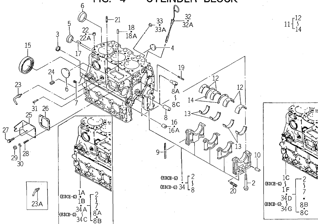
FIG. 4 CYLINDER BLOCK
