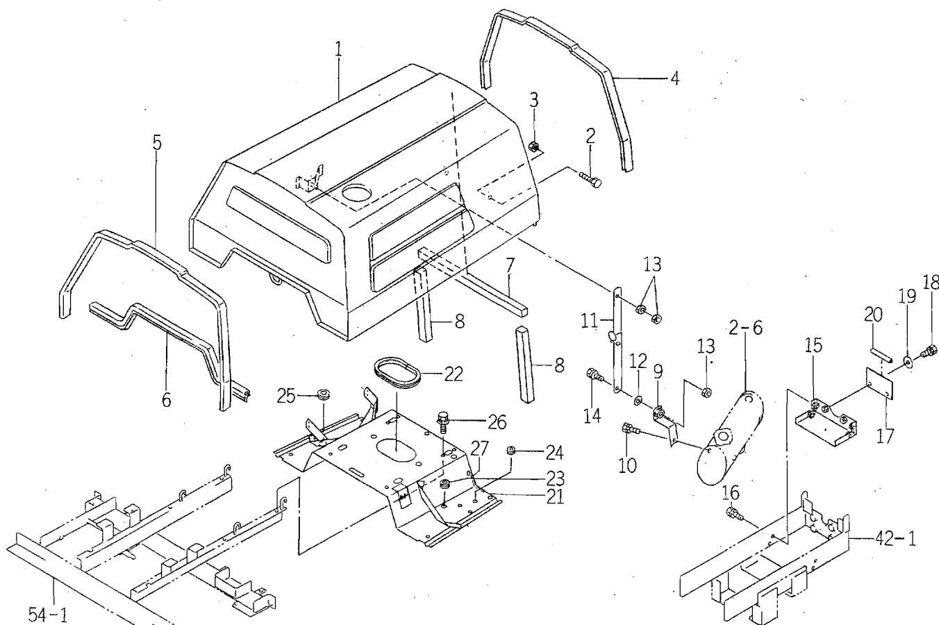
FIG. 63 HOOD SYSTEM
