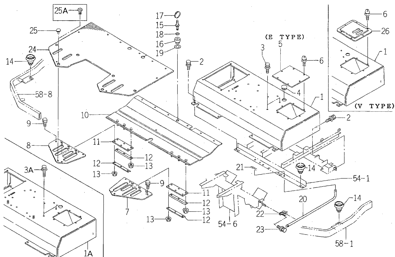
FIG. 57 STEP,FENDER SYSTEM
