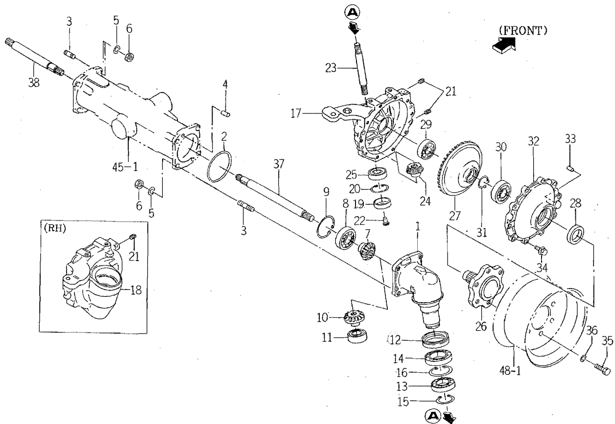
FIG. 46 FINAL GEAR CASE, FINAL DRIVE SHAFT SYSTEM
