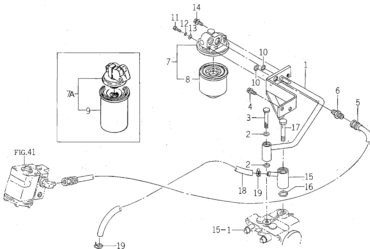
FIG. 28 PIPING (HST) SYSTEM
