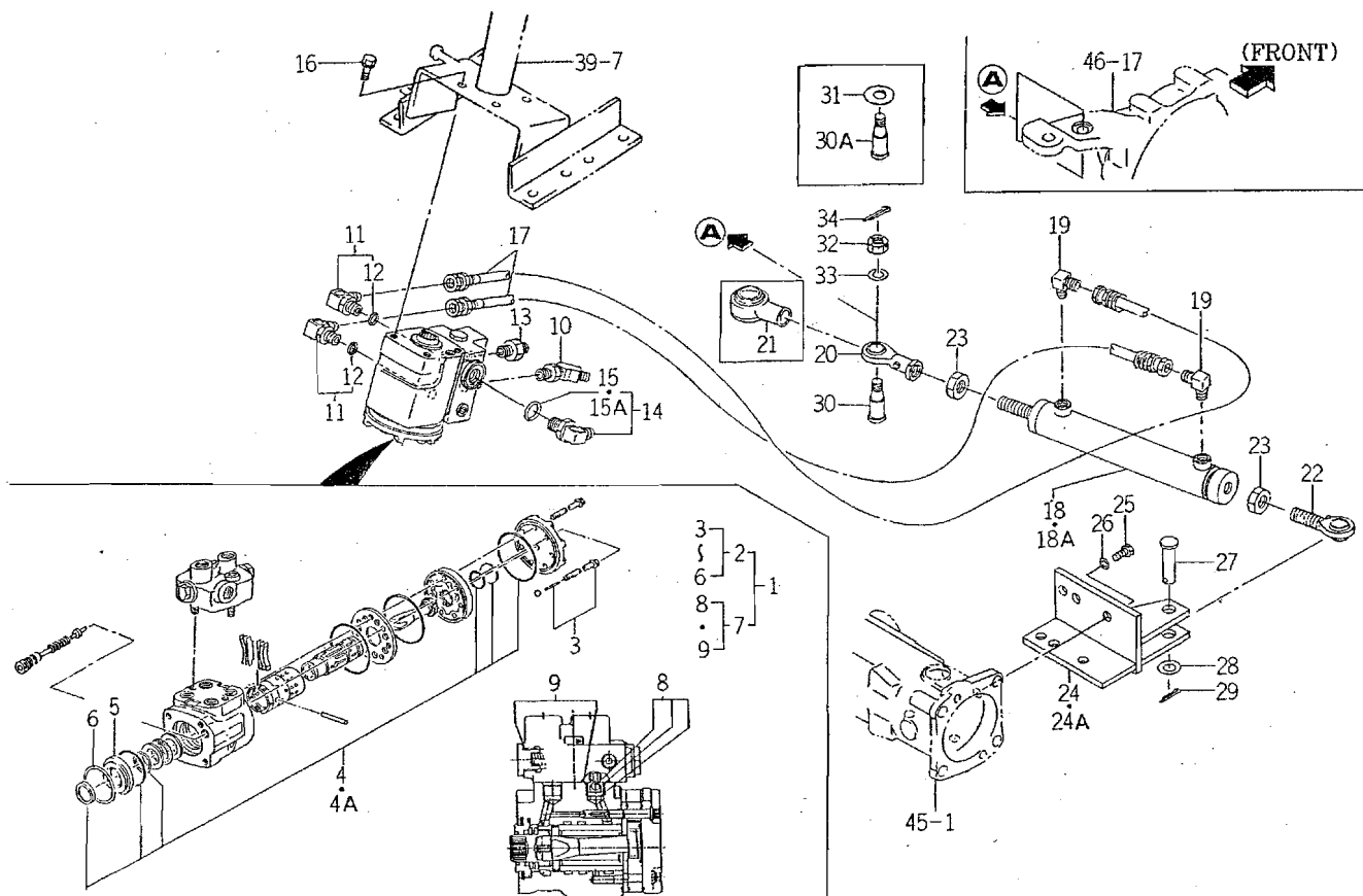
FIG. 41 STEERING (UNIT) SYSTEM
