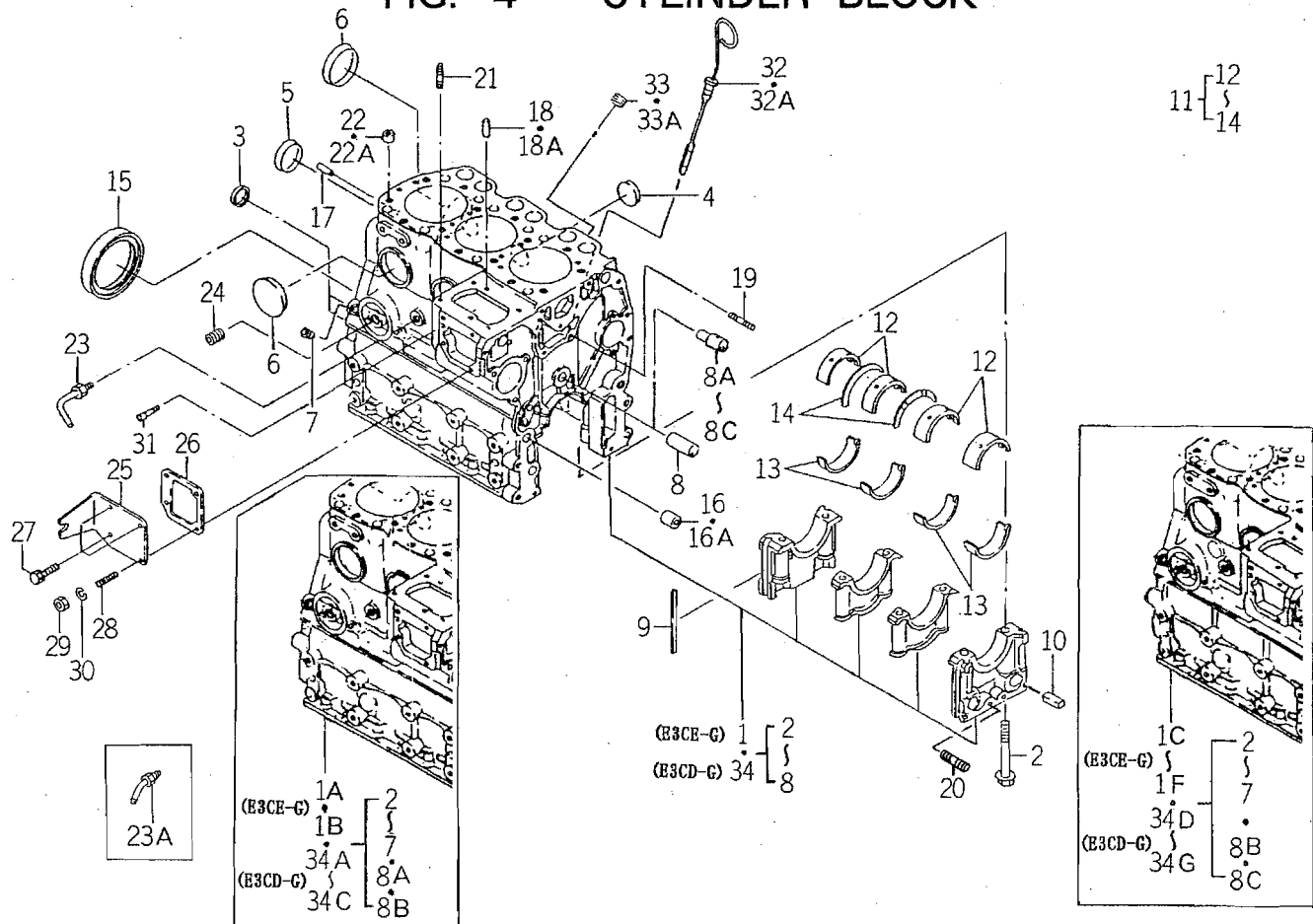
FIG. 4 CYLINDER BLOCK
