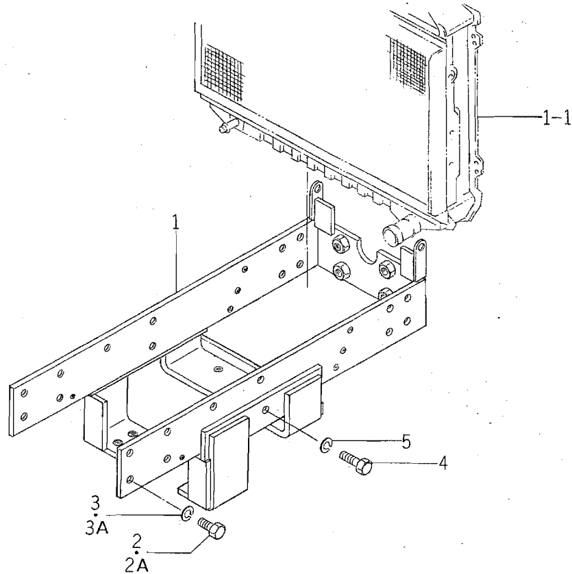
FIG. 42 BRACKET (AXLE) SYSTEM
