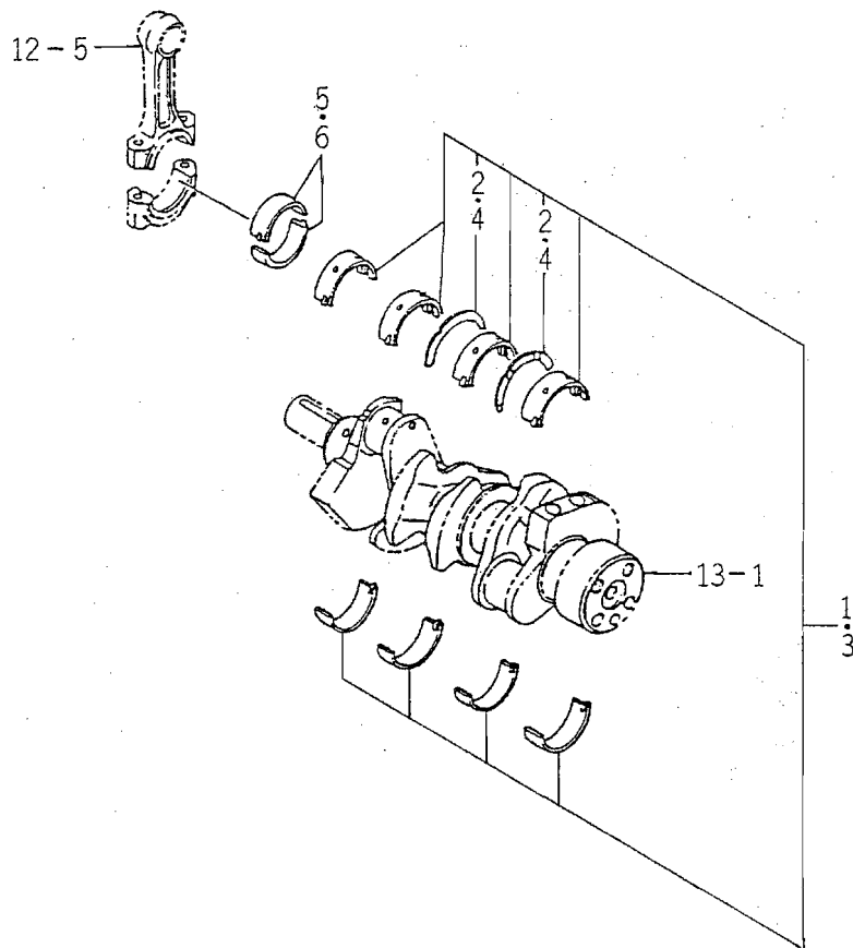
FIG. 5 BEARING/UNDER SIZE (OPTION)
