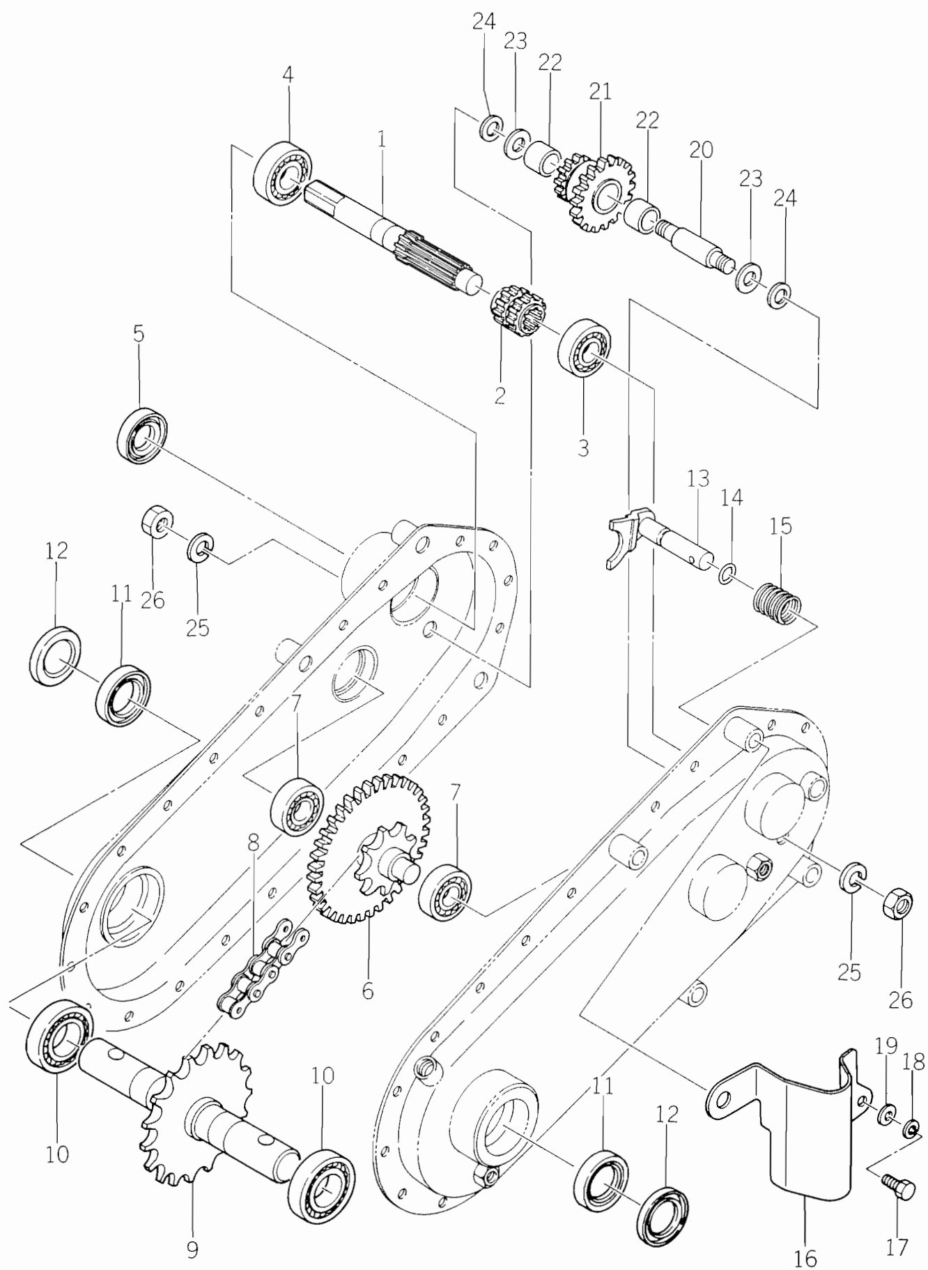
Fig. 6 TRANSMISSION GEAR (AC-20R, AC-40R)
